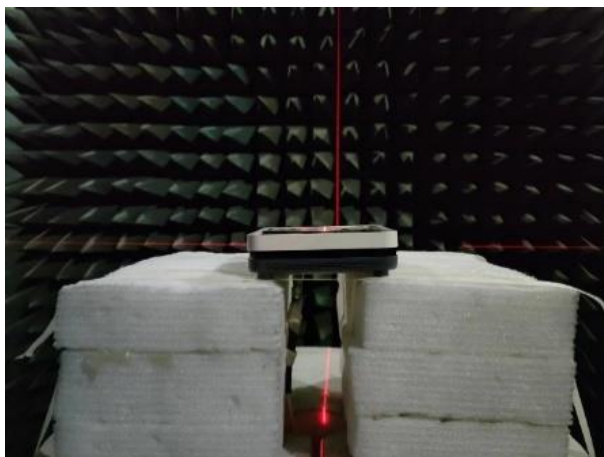
Radiation Pattern Test
