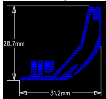
4G Secondary antenna
