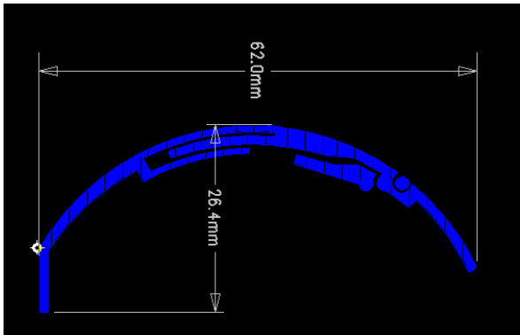
4G Main antenna
