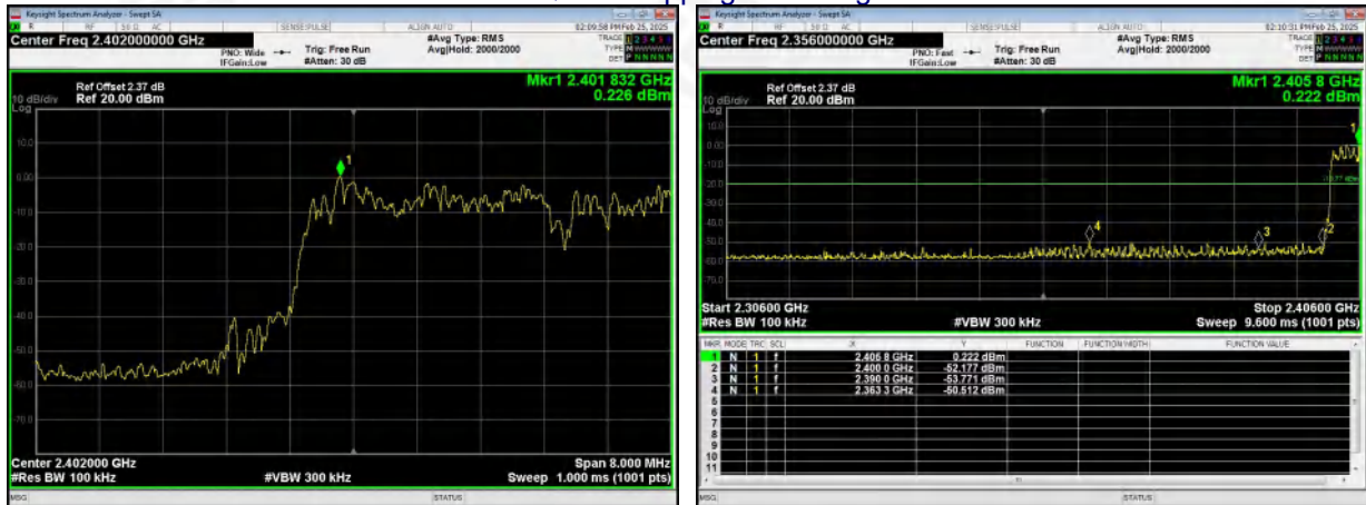
\pi/4 -DQPSK Hopping Band edge-left side
