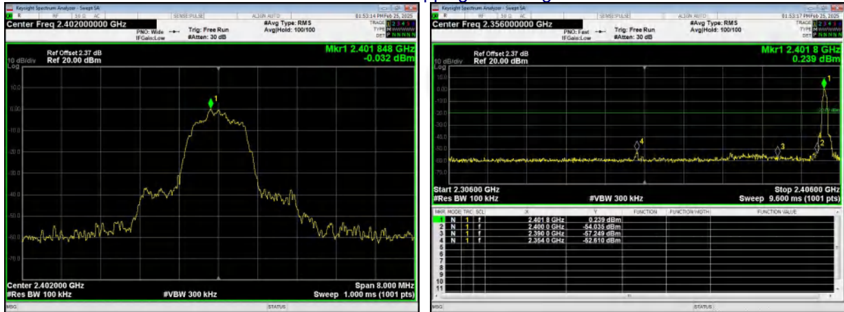
\pi/4 -DQPSK No-hopping Band edge-left side
