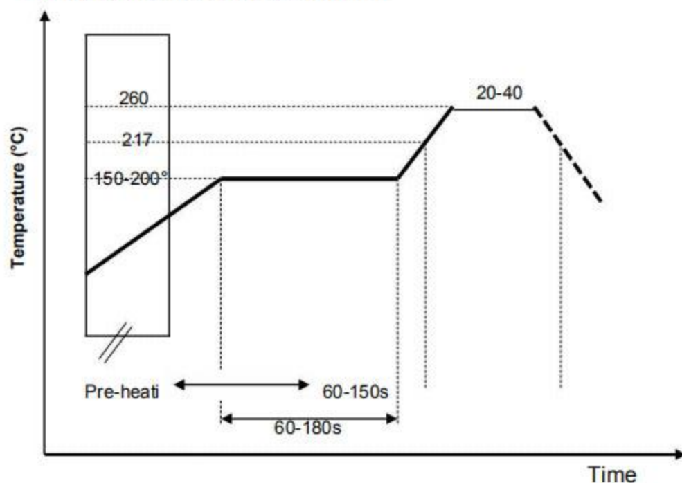
Typical Soldering Profile for Lead-free Process
