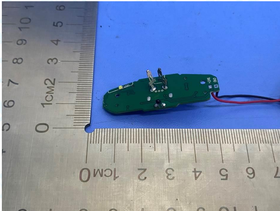
Photo 20 Appearance of Battery(BOX)
