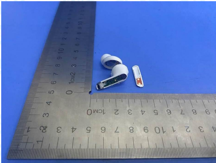
Photo 10 Internal of Battery(Earphone)
