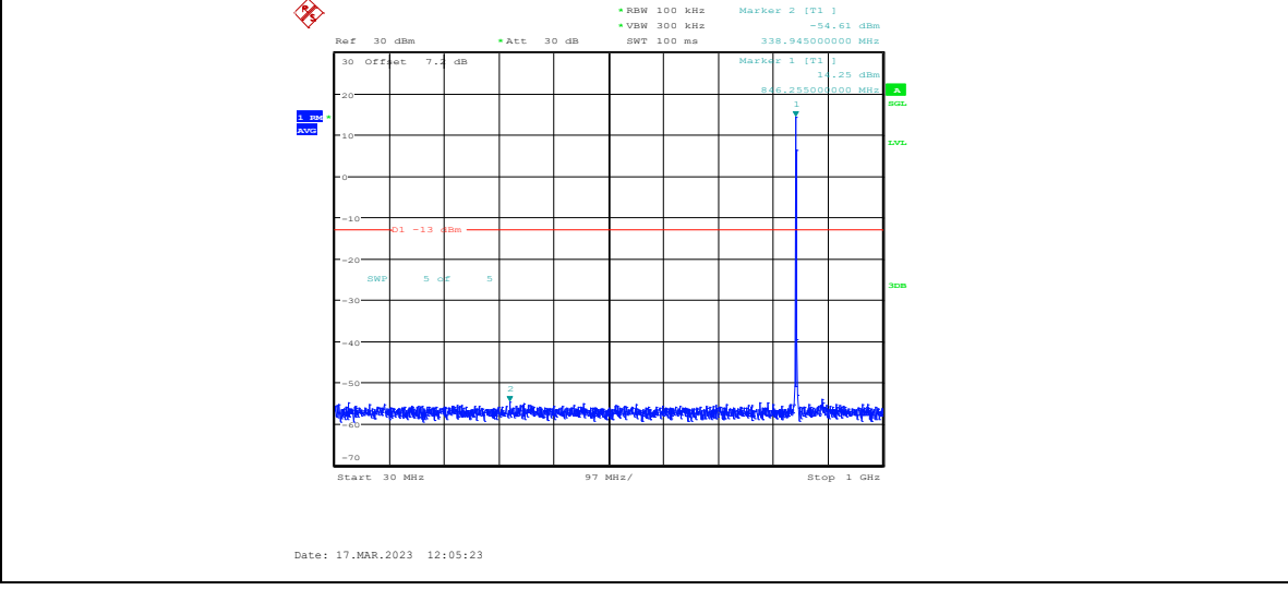
Band5-3MHz-QPSK-20635-1RB#0-Range3:30~1000MHz
