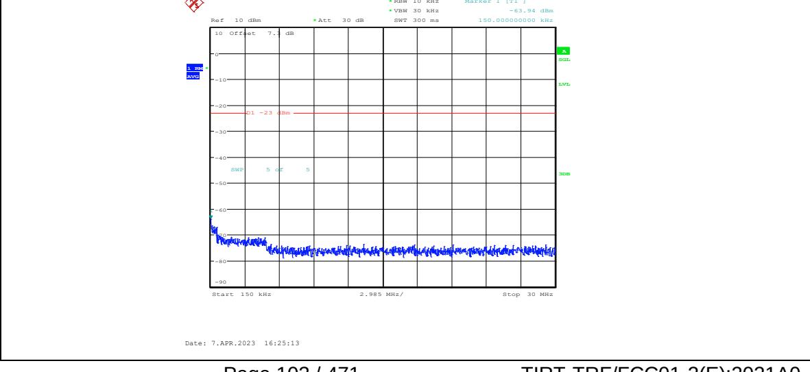
Band2-3MHz-16QAM-18900-1RB#0-Range2:0.15~30MHz
