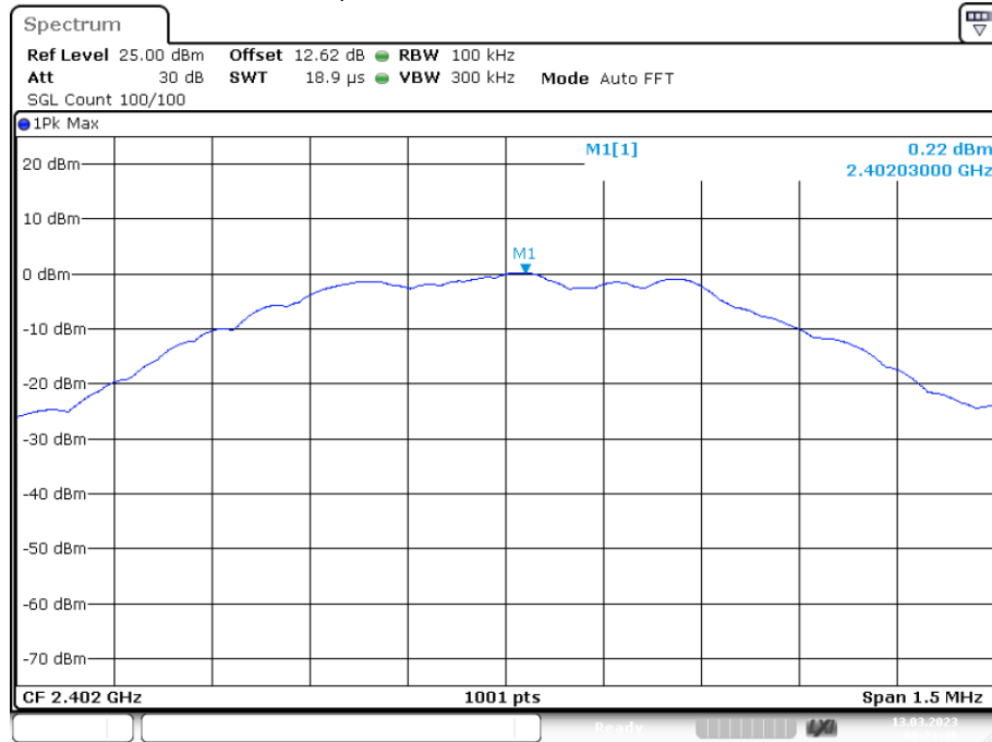
Tx. Spurious NVNT 1M 2402MHz Ant1 Ref
