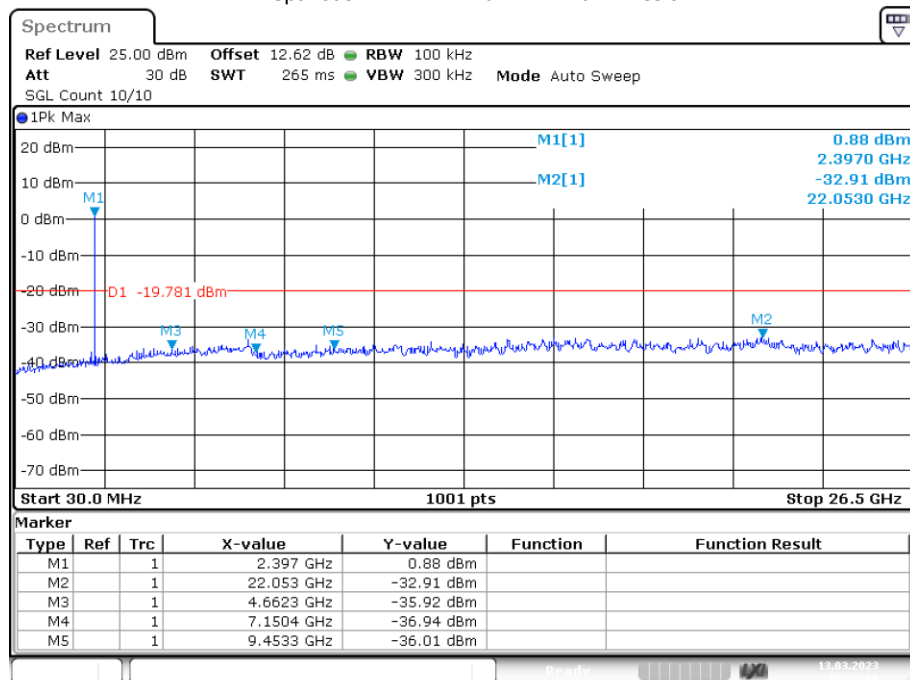
Tx. Spurious NVNT 1M 2402MHz Ant1 Emission
