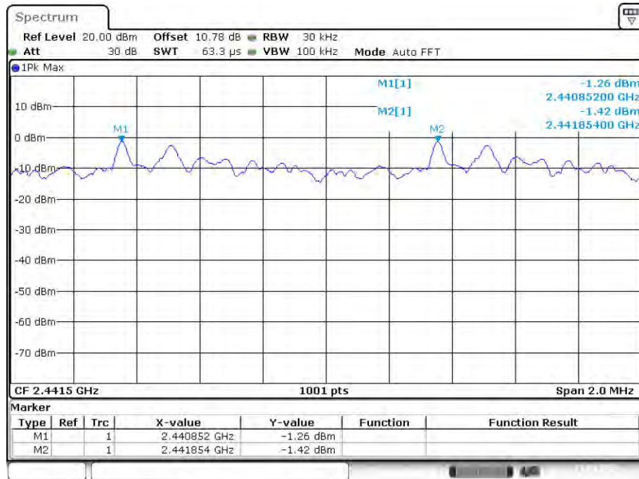
CFS NVNT 3-DH1 2441MHz Ant1
