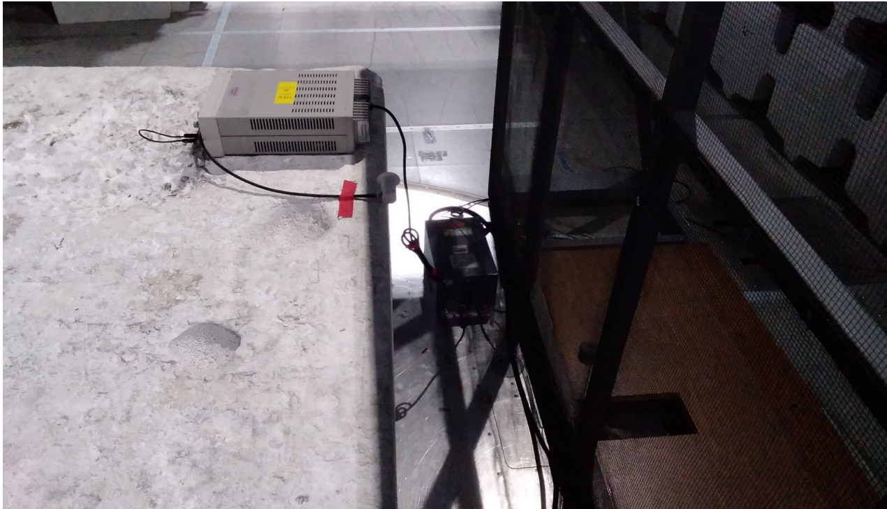
Test Configuration Photograph #1 (Conducted Emissions - Power Port)
