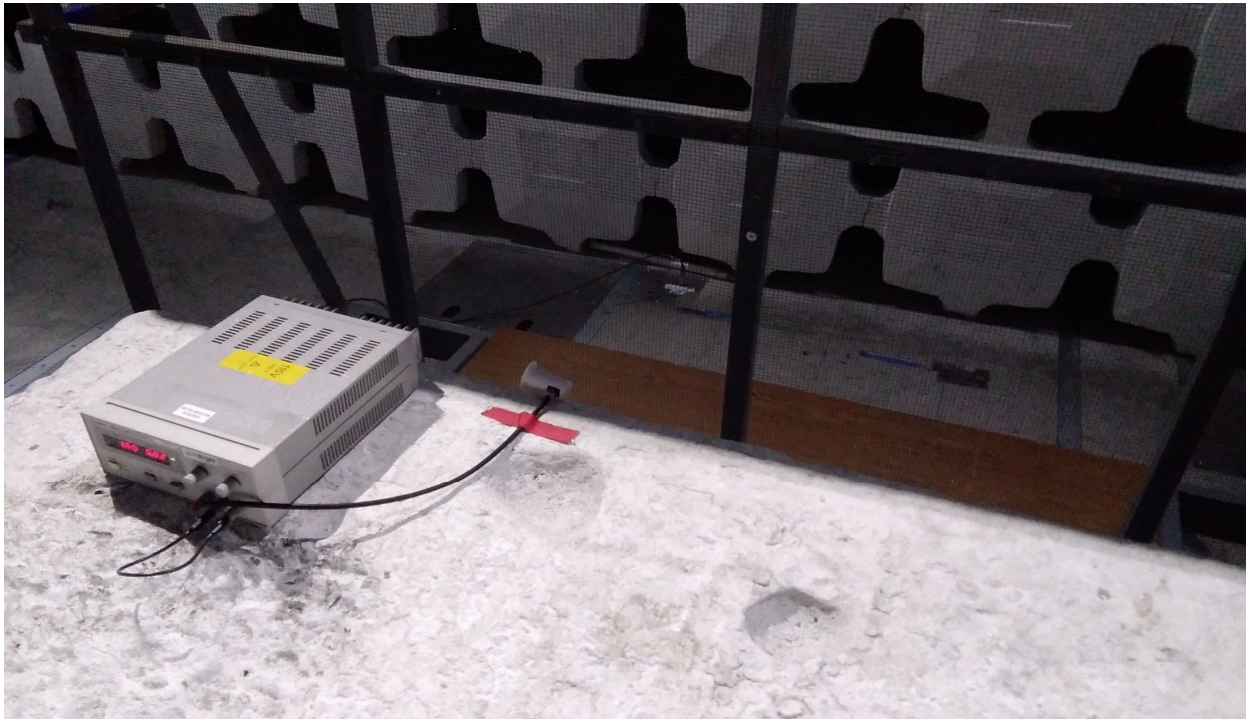
Test Configuration Photograph #2 (Conducted Emissions - Power Port)
