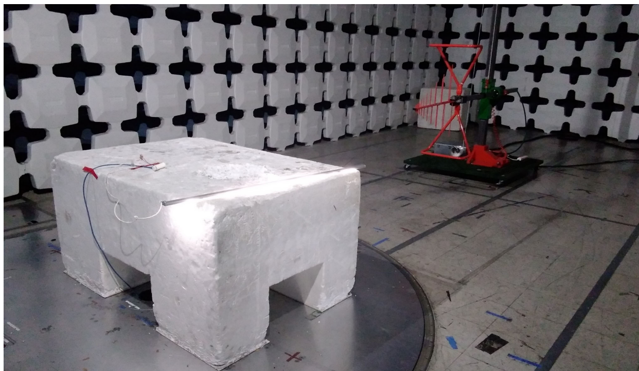
Test Configuration Photograph #1 (Radiated Emissions)
