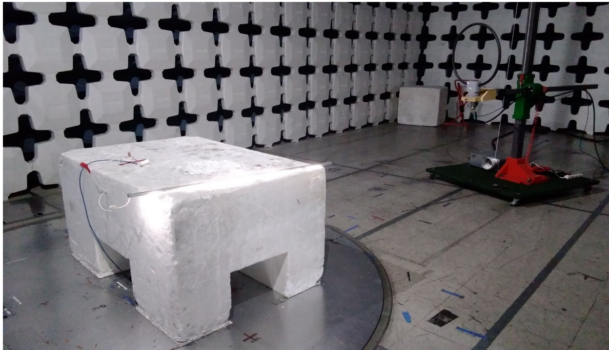
Test Configuration Photograph #2 (Radiated Emissions - Below 30 MHz)
