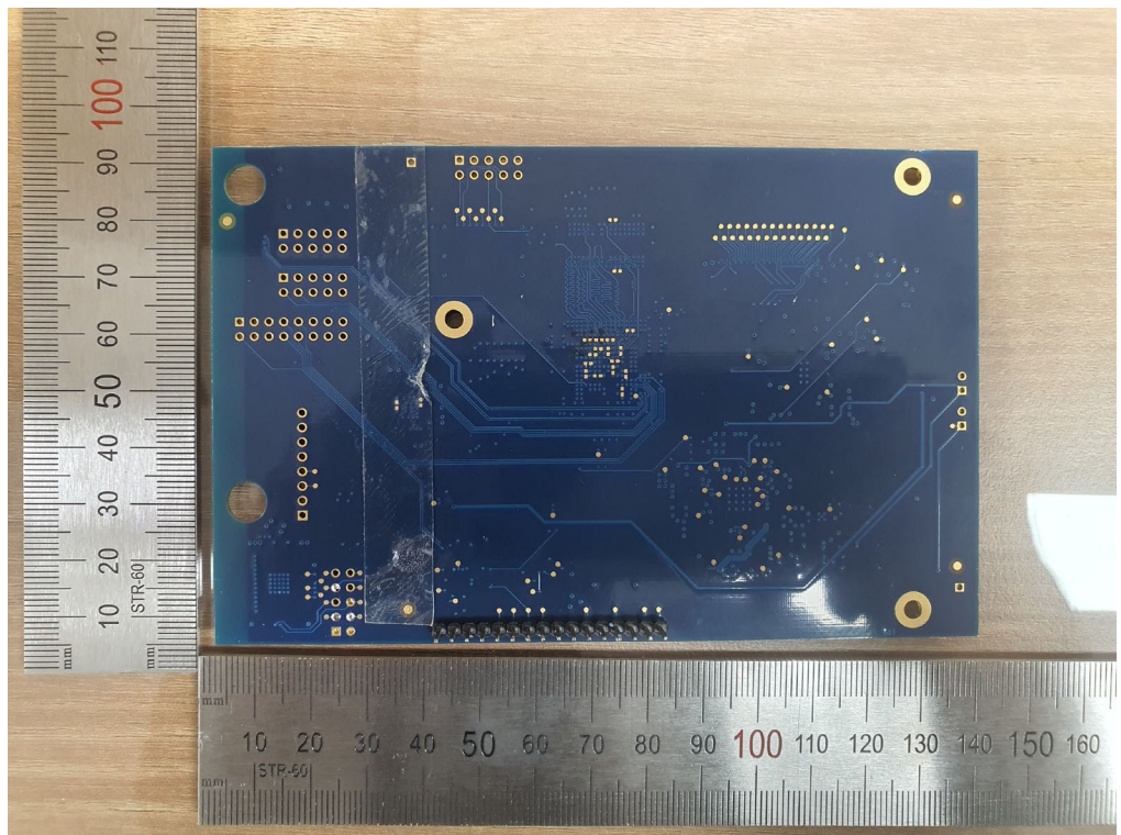
[Mainboard Rear]
