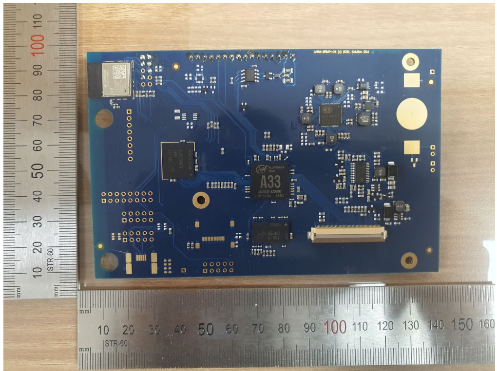
[Mainboard Rear]
