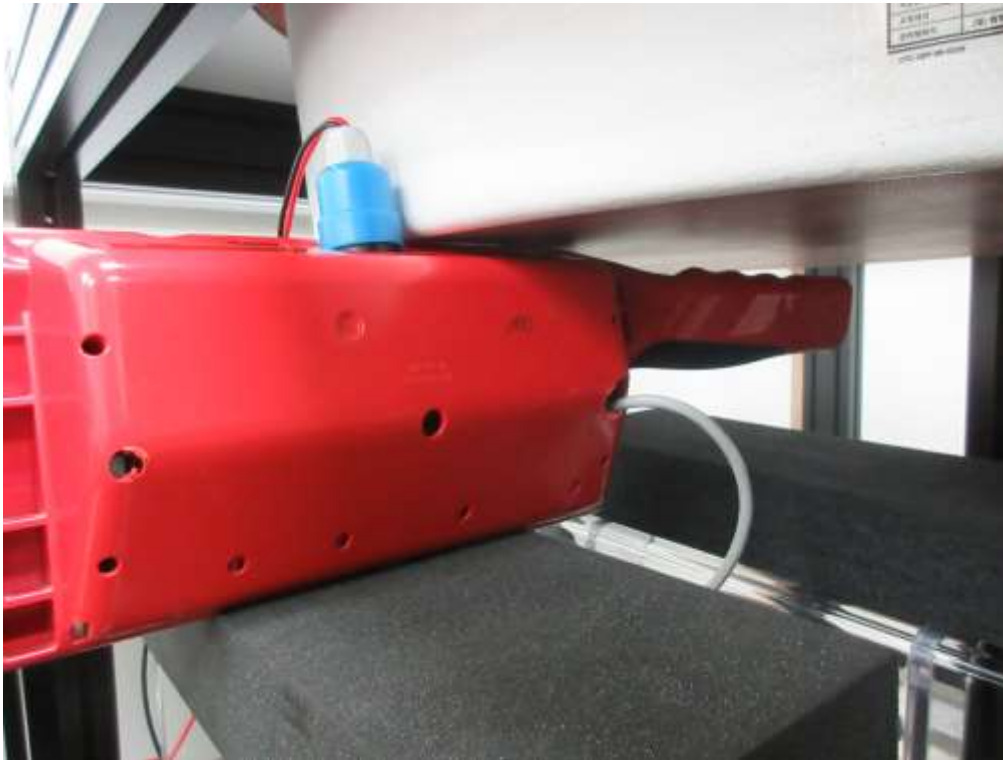
Top from ELI Phantom (Separation Distance: 0 cm)
