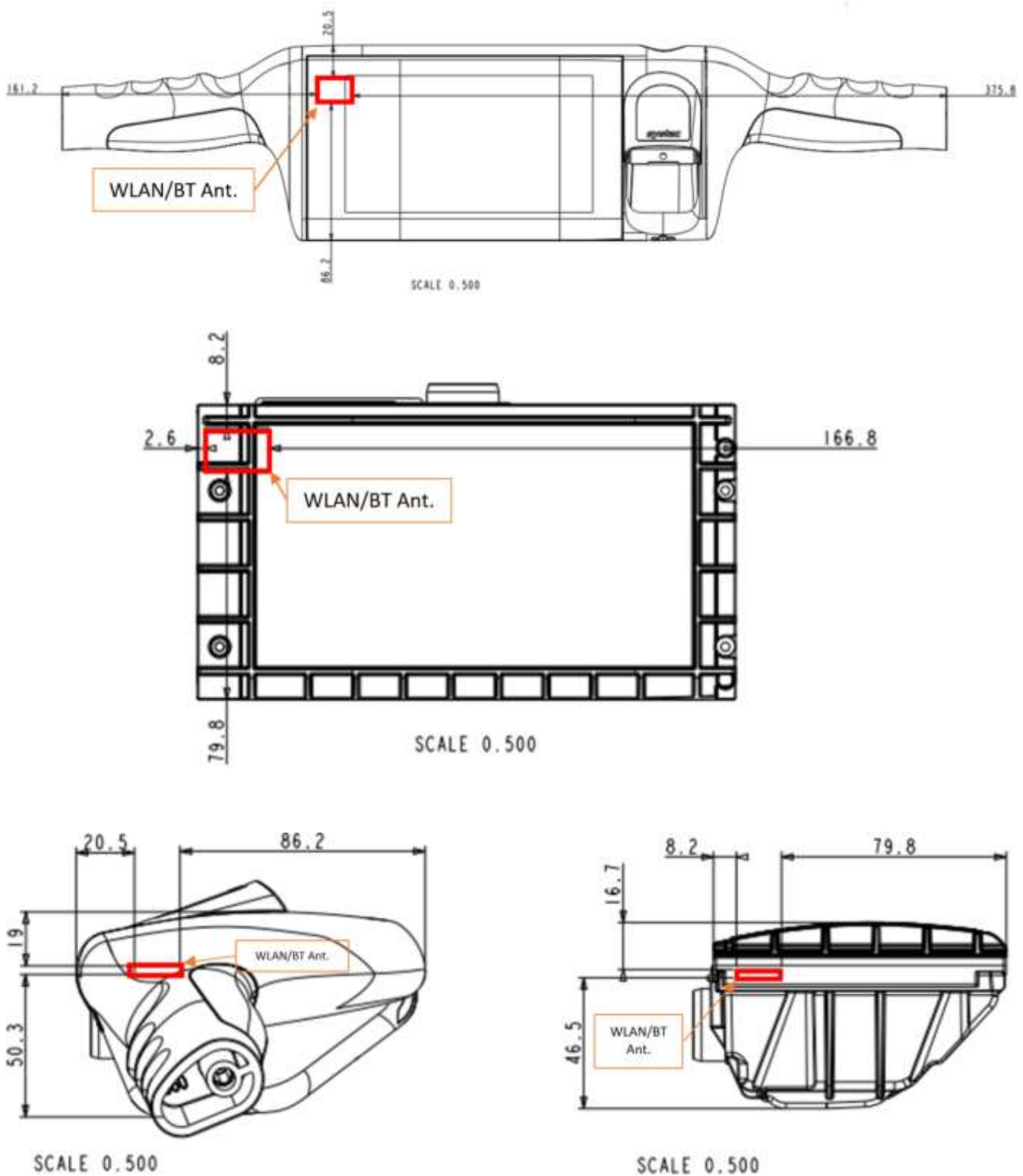
Figure F-1 Antenna Location
