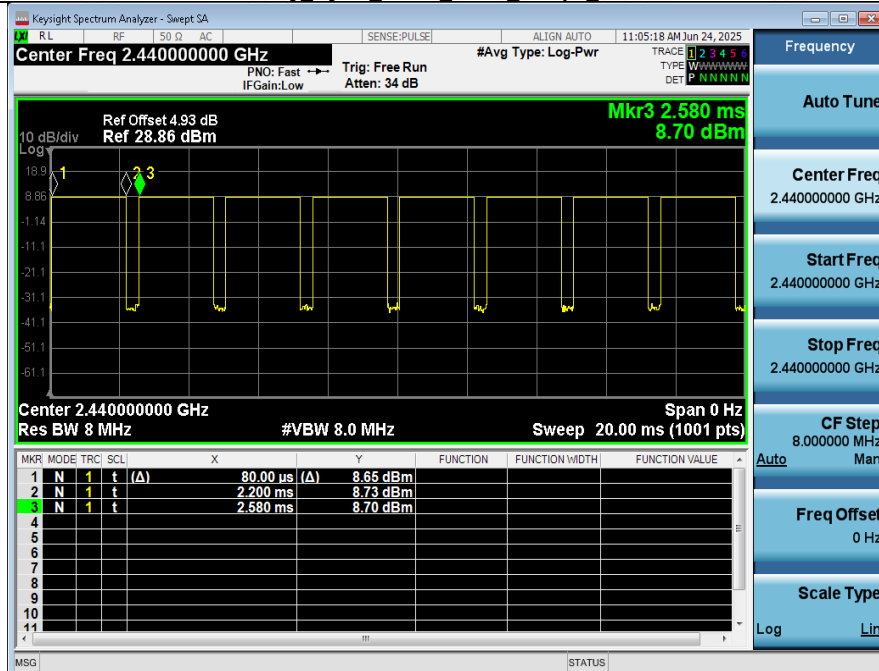
Duty Cycle_NVNT_ANT1_1Mbps_2440
