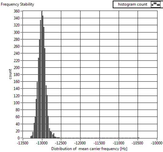
Histogram of Carrier Frequency Stability
