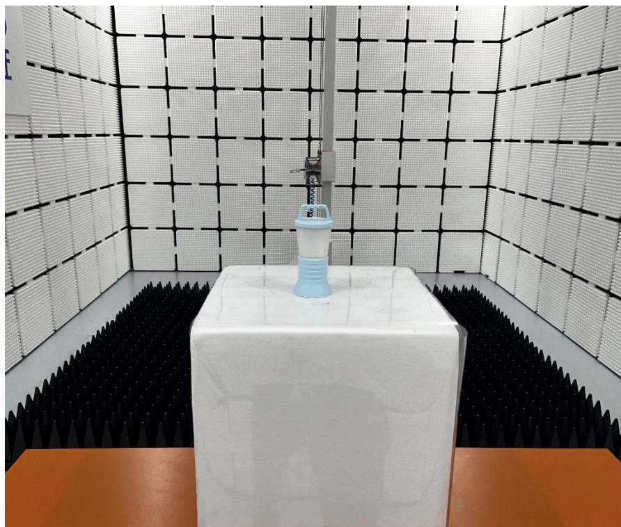
Radiated Emission Above 1GHz
