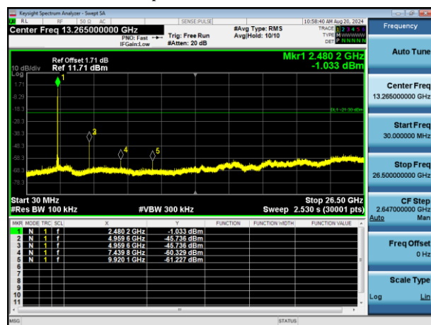
Spurious Emissions
