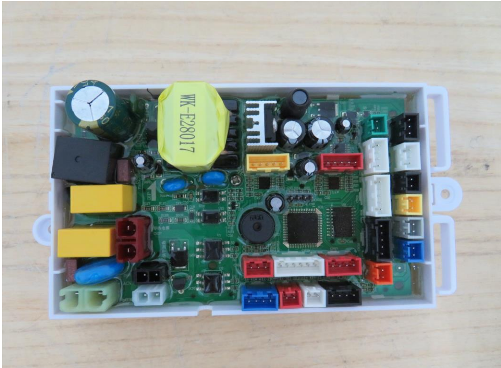
(7) EUT Photo
