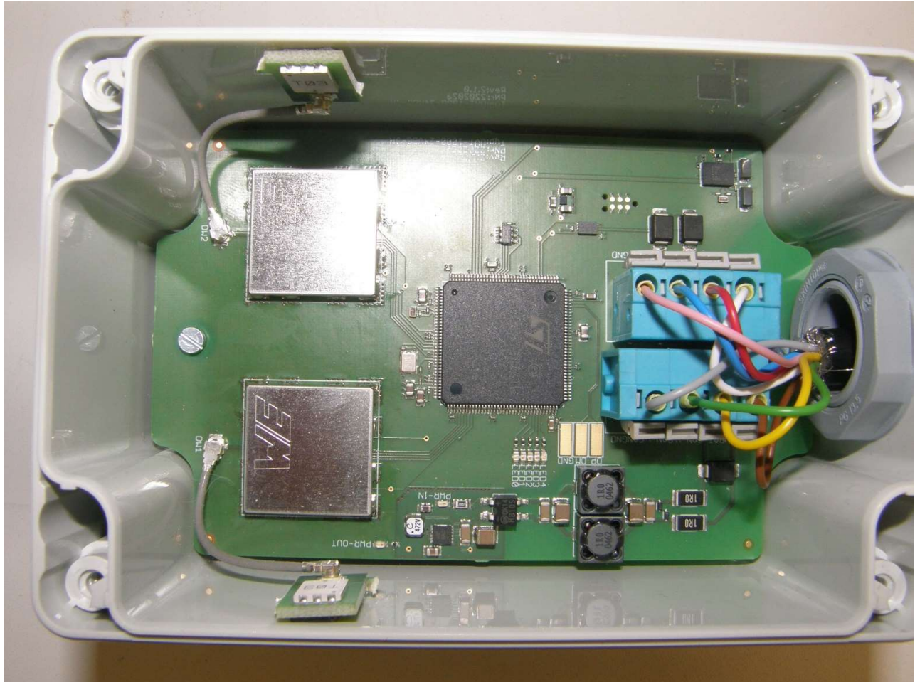
Photo of EUT: Internal construction upper side
