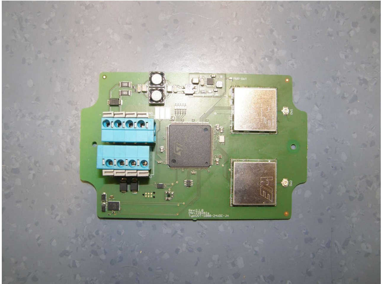
Photo of EUT: PCB upper side
