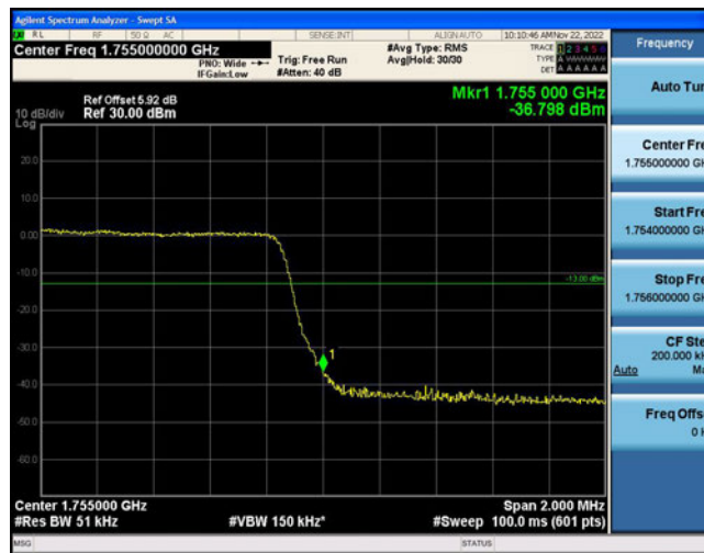
Band4-3MHz-QPSK-20385-15RB#0
