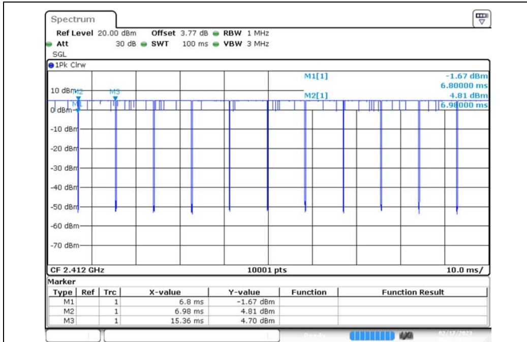
Test Graphs of Duty Cycle
