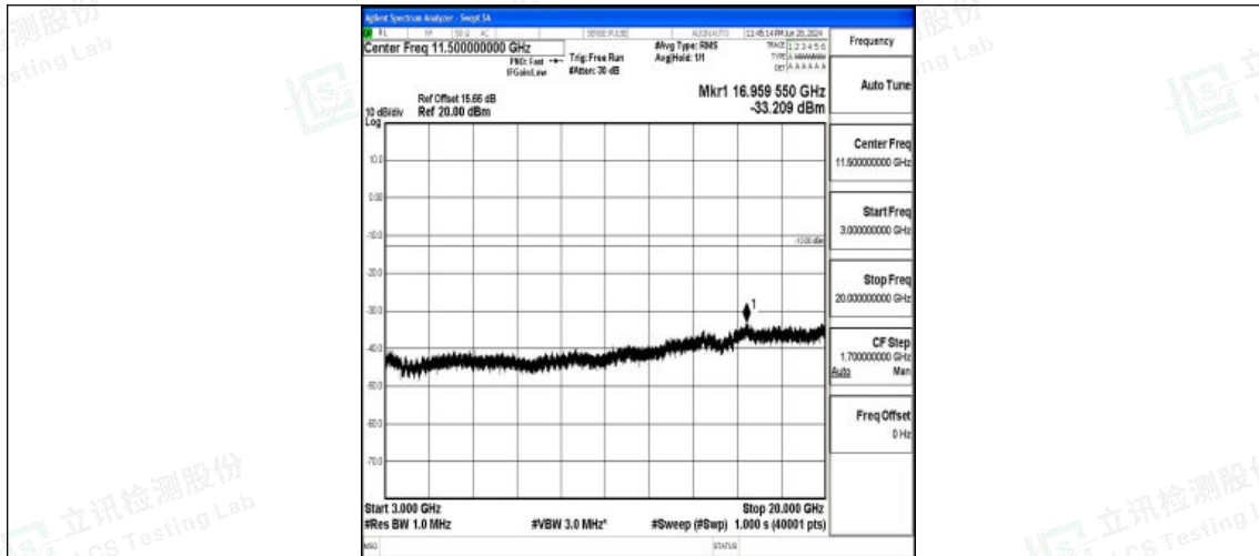
Band2_3MHz_QPSK_18615_1RB#0_3000~20000_3000~20000
