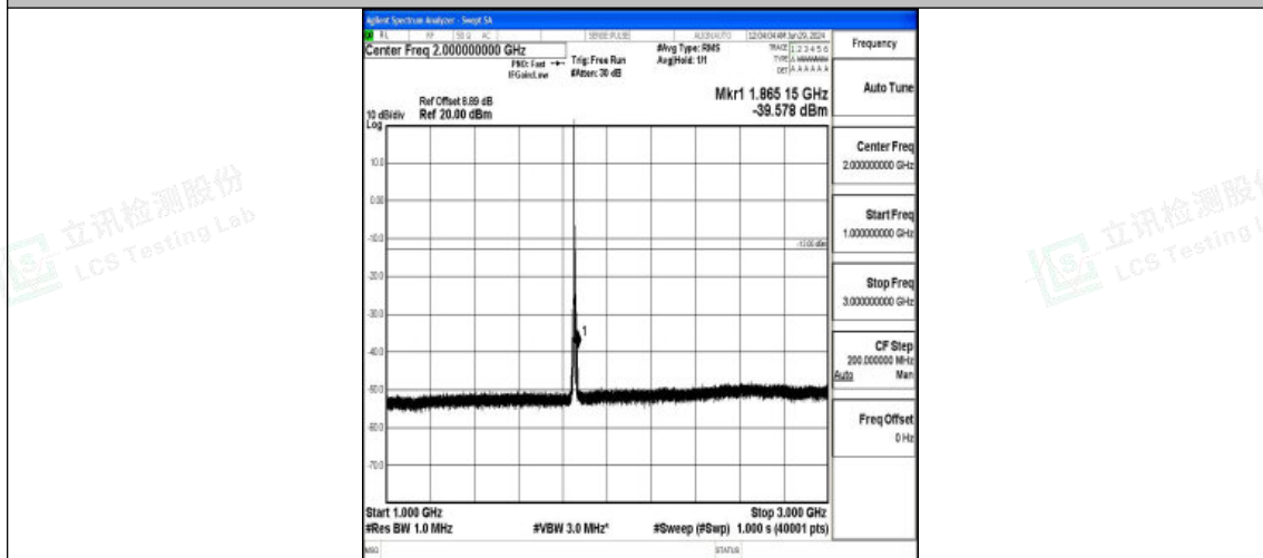
Band2_5MHz_QPSK_18625_1RB#0_1000~3000_1000~3000
