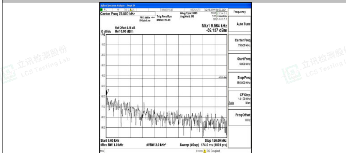
Band2_15MHz_16QAM_18900_1RB#0_0.009~0.15_0.009~0.15
