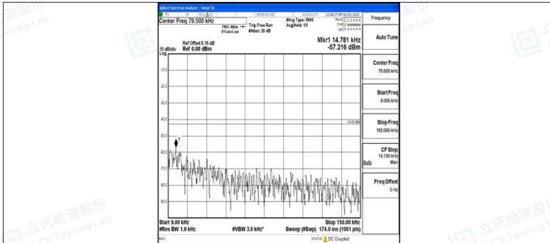
Band2_5MHz_16QAM_19175_1RB#0_0.009~0.15_0.009~0.15
