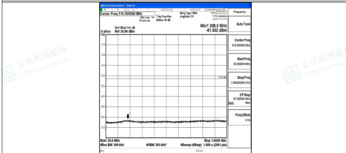
Band2_10MHz_16QAM_19150_1RB#0_30~1000_30~1000
