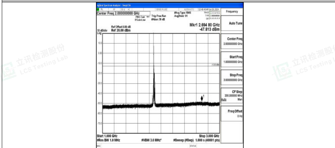
Band2_15MHz_16QAM_18900_1RB#0_1000~3000_1000~3000
