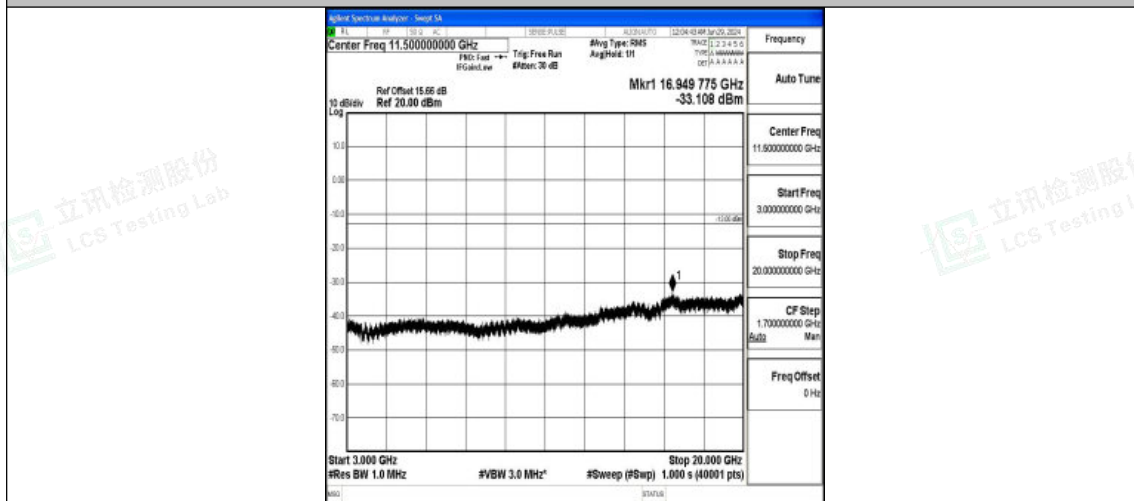
Band2_5MHz_16QAM_18625_1RB#0_3000~20000_3000~20000
