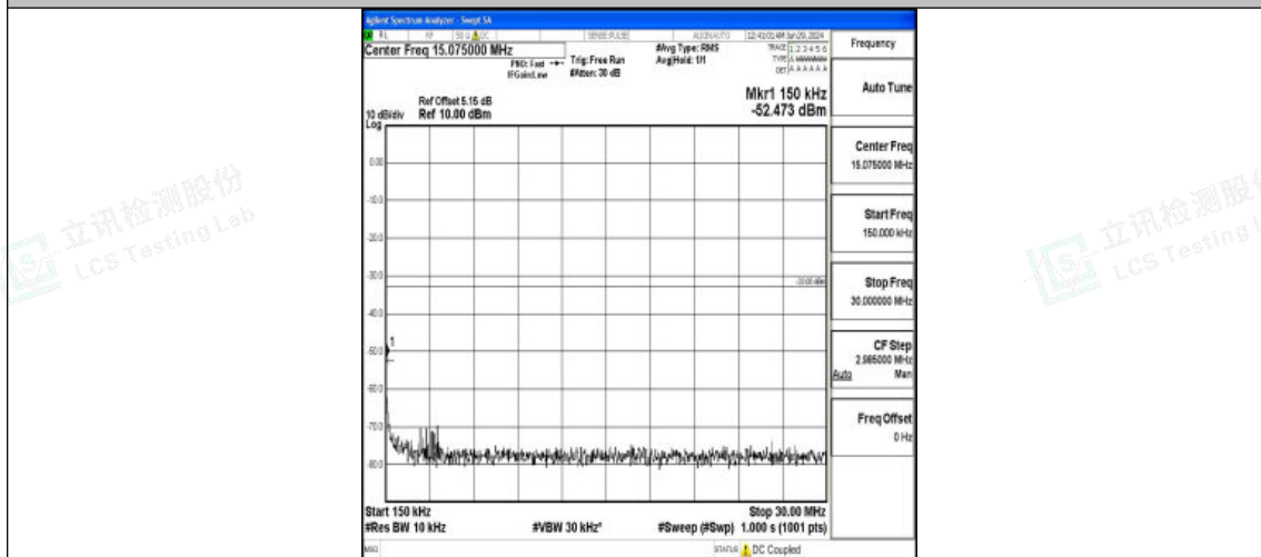
Band2_15MHz_QPSK_19125_1RB#0_0.15~30_0.15~30
