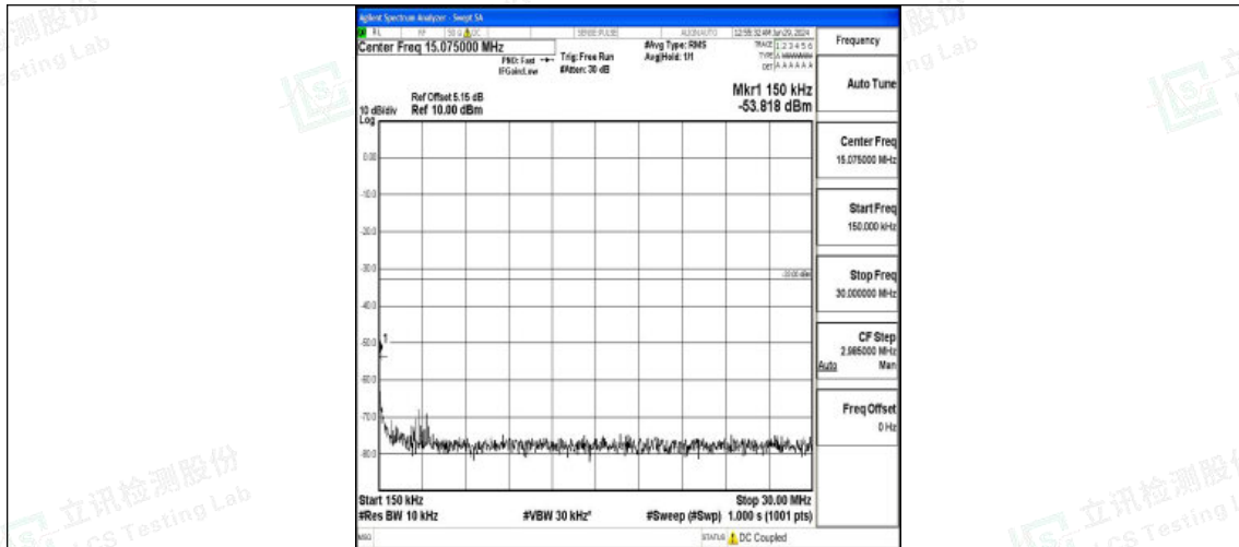
Band2_20MHz_QPSK_18700_1RB#0_0.15~30_0.15~30
