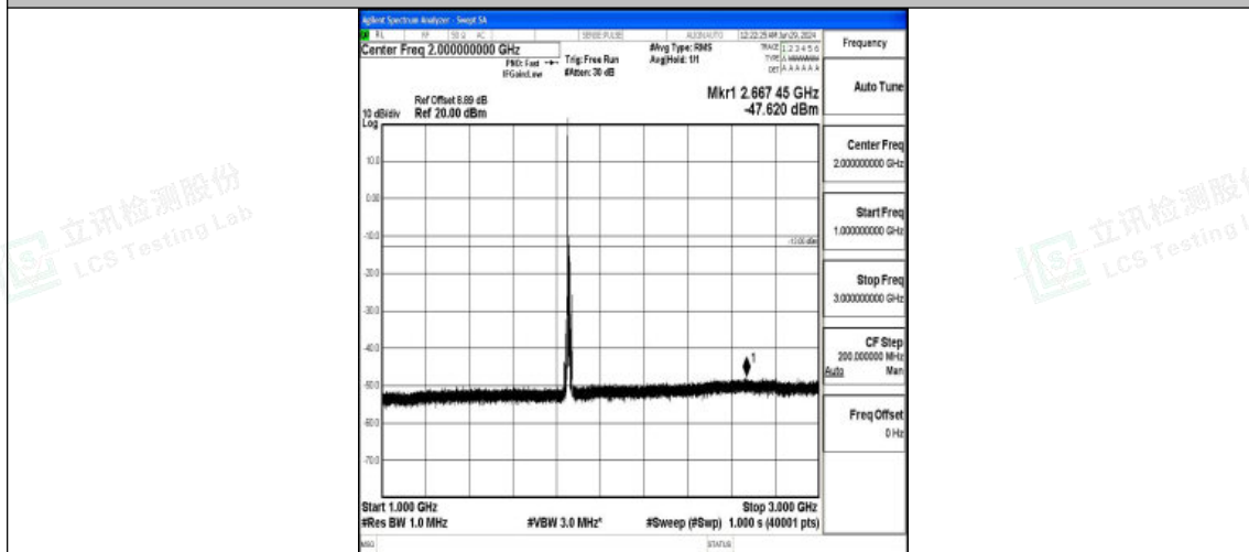
Band2_10MHz_QPSK_18650_1RB#0_1000~3000_1000~3000
