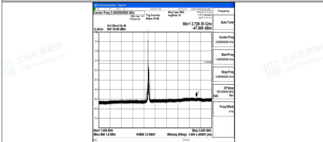
Band2_20MHz_16QAM_18900_1RB#0_1000~3000_1000~3000
