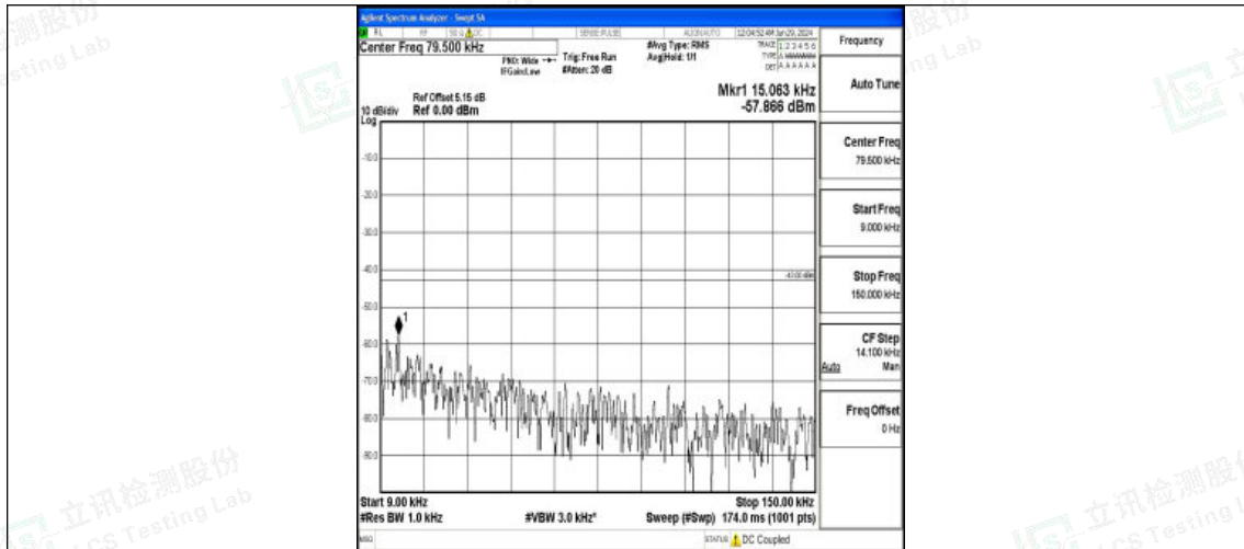
Band2_5MHz_QPSK_18900_1RB#0_0.009~0.15_0.009~0.15
