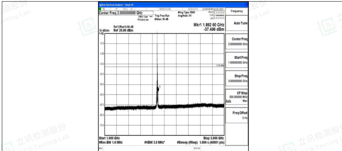
Band2_5MHz_QPSK_18900_1RB#0_1000~3000_1000~3000
