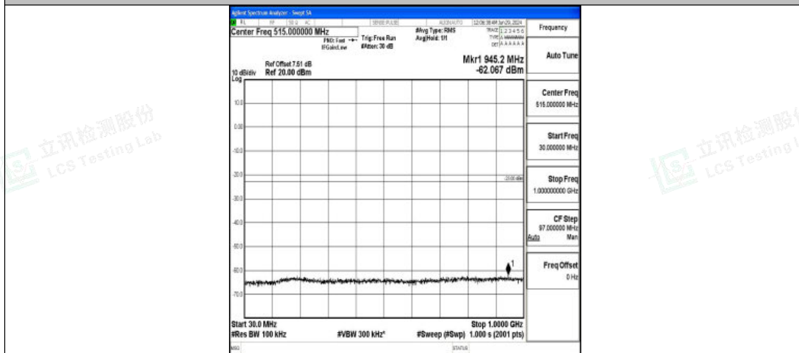
Band2_5MHz_16QAM_19175_1RB#0_30~1000_30~1000
