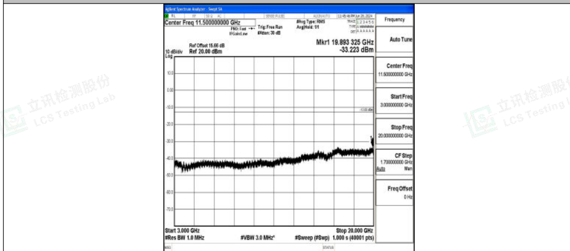
Band2_3MHz_16QAM_18615_1RB#0_3000~20000_3000~20000
