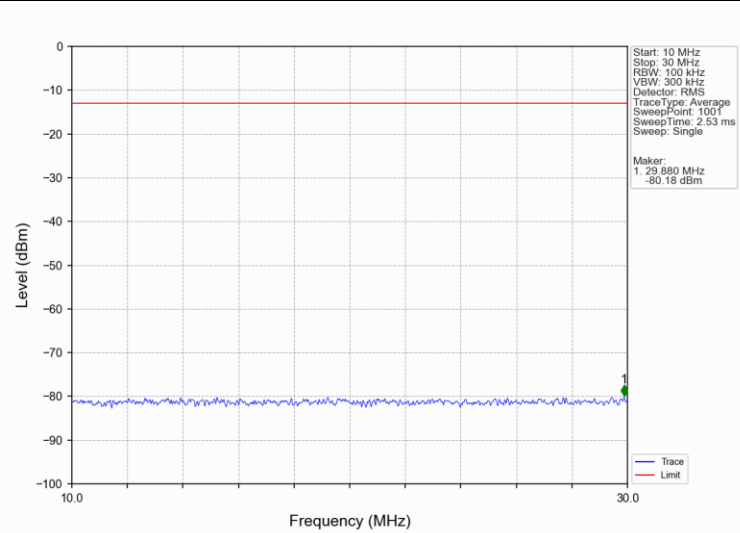
Band66_15MHz_QPSK_HCH_1772.5MHz_RB_1_0_NTNV
