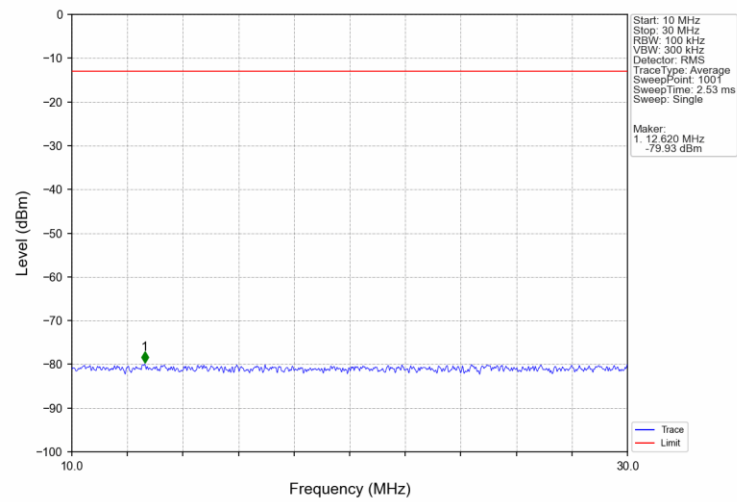
Band66_15MHz_QPSK_MCH_1745MHz_RB_1_0_NTNV
