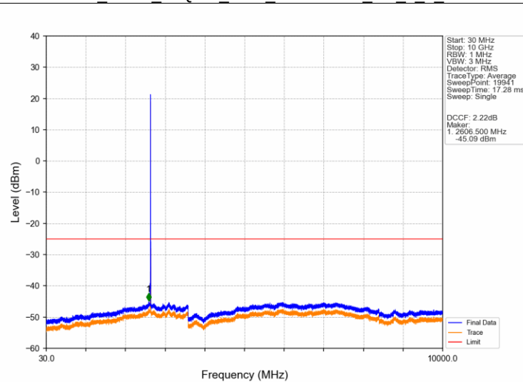
Band41_5MHz_16QAM_HCH_2652.5MHz_RB_1_0_NTNV
