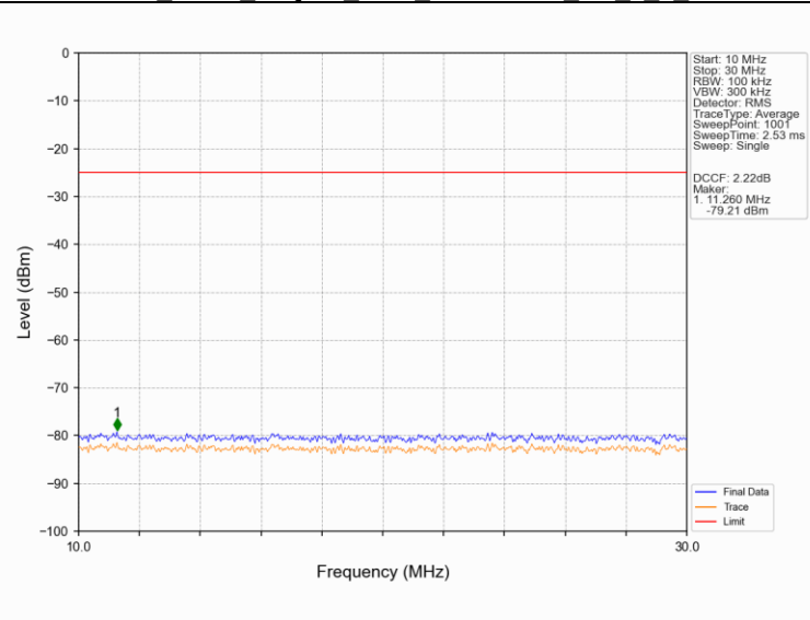
Band41_5MHz_16QAM_HCH_2652.5MHz_RB_1_0_NTNV
