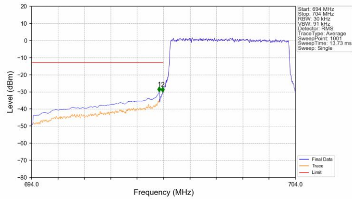
Band12 5MHz 16QAM LCH 701.5MHz RB 25 0 NTNV
