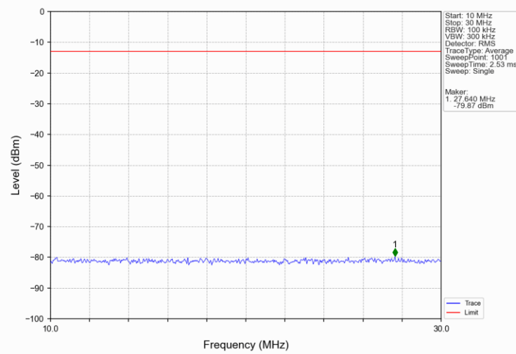
Band4 15MHz 16QAM HCH 1747.5MHz RB 1 0 NTVN
