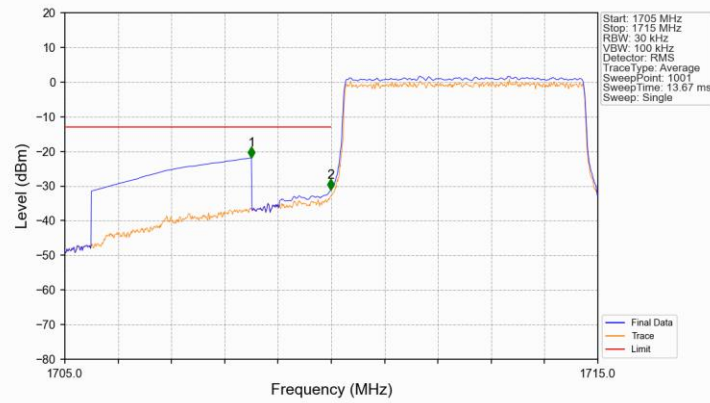
Band4_5MHz_16QAM_LCH_1712.5MHz_RB_25_0_NTV
