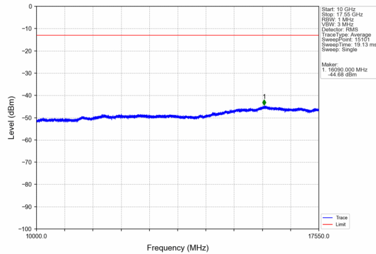
Band4_5MHz_16QAM_LCH_1712.5MHz_RB_25_0_NTV
