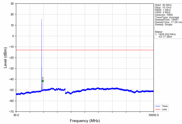
Band2_5MHz_16QAM_MCH_1880MHz_RB_1_0_NTNV
