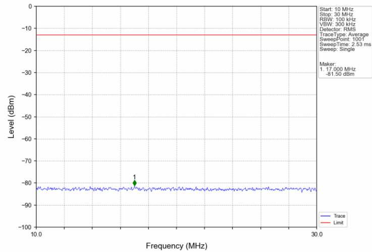
Band2 5MHz 16QAM LCH 1852.5MHz RB 1 0 NTNV
