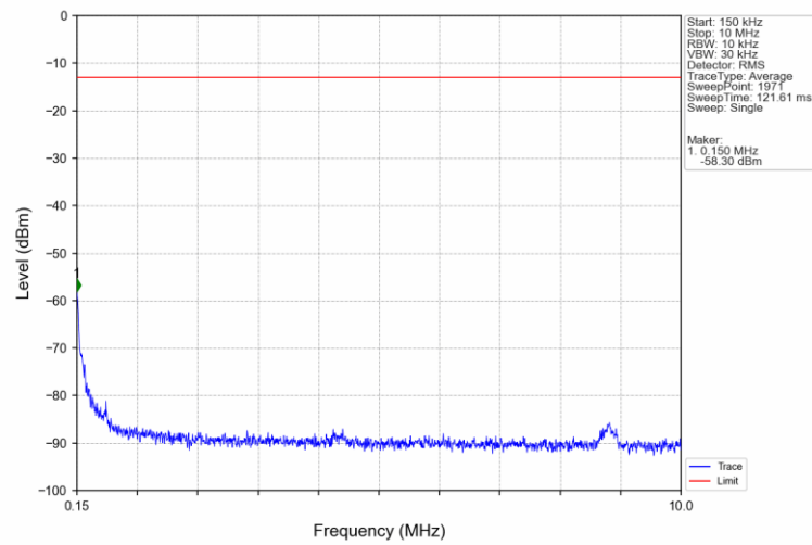
Band5_10MHz_16QAM_HCH_844MHz_RB_1_0 NTN
