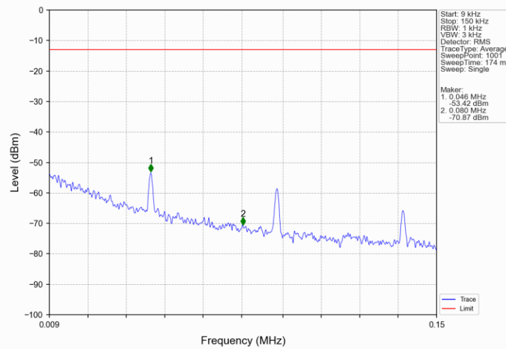
Band5_3MHz_16QAM_MCH_836.5MHz_RB_1_0_NTNV
