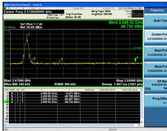
BLE_2M-Ant1-High-2480--0.48
