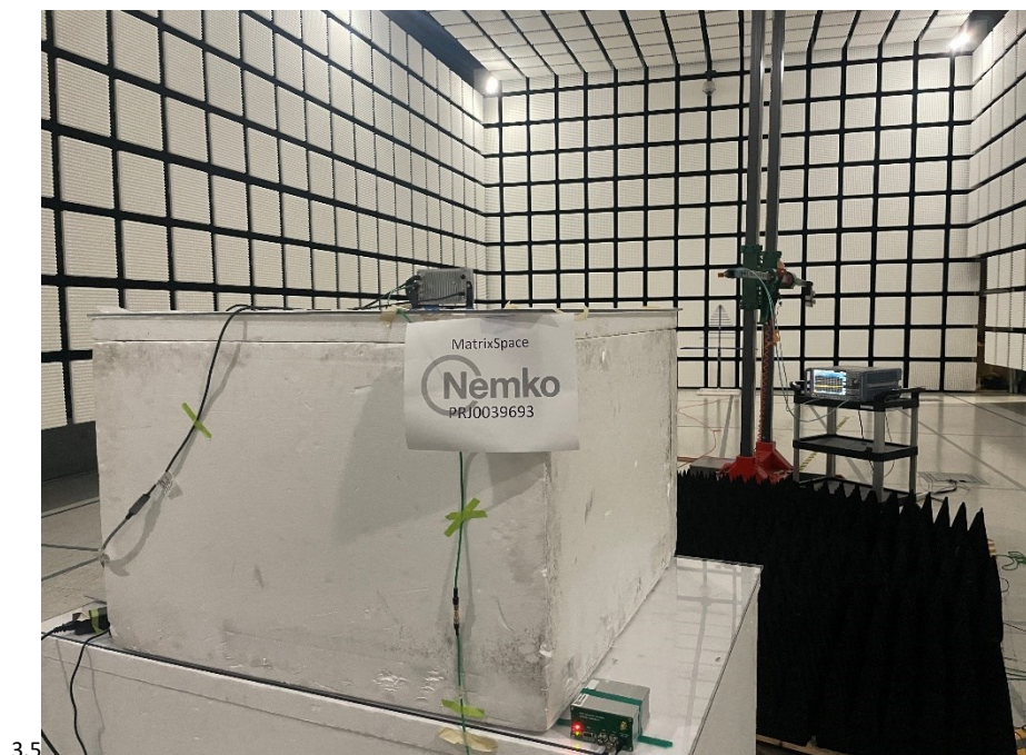
Figure 15 - Radiated emissions above 1 GHz (50 – 75 GHz), rear view.
