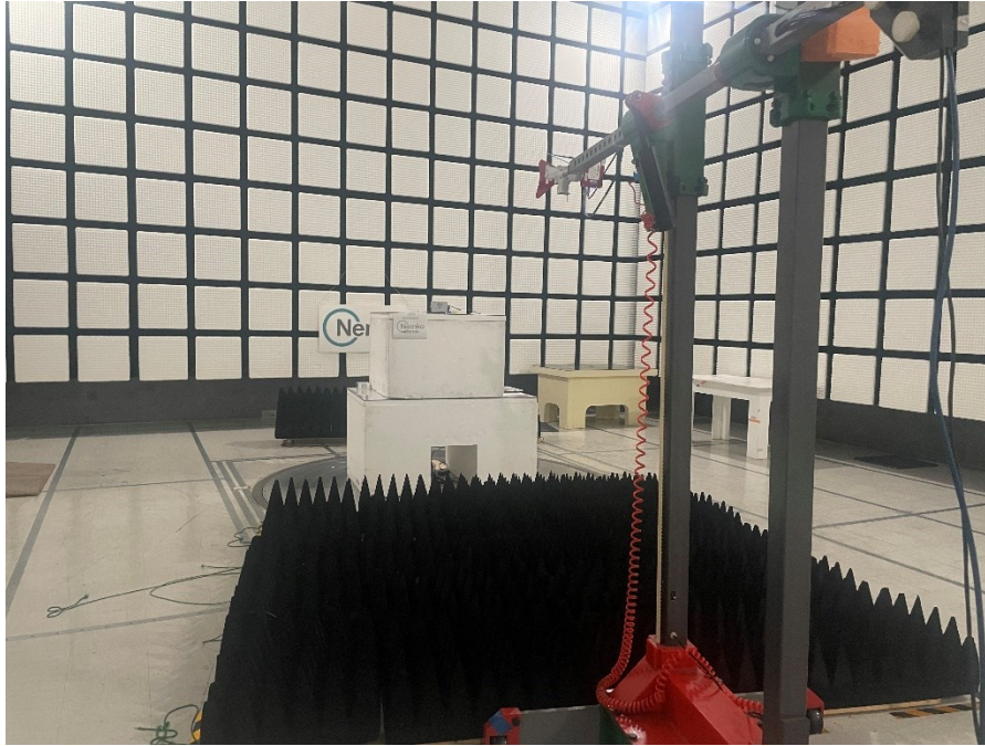
Figure 6 - Radiated emissions above 1 GHz (1– 18 GHz), front view.
