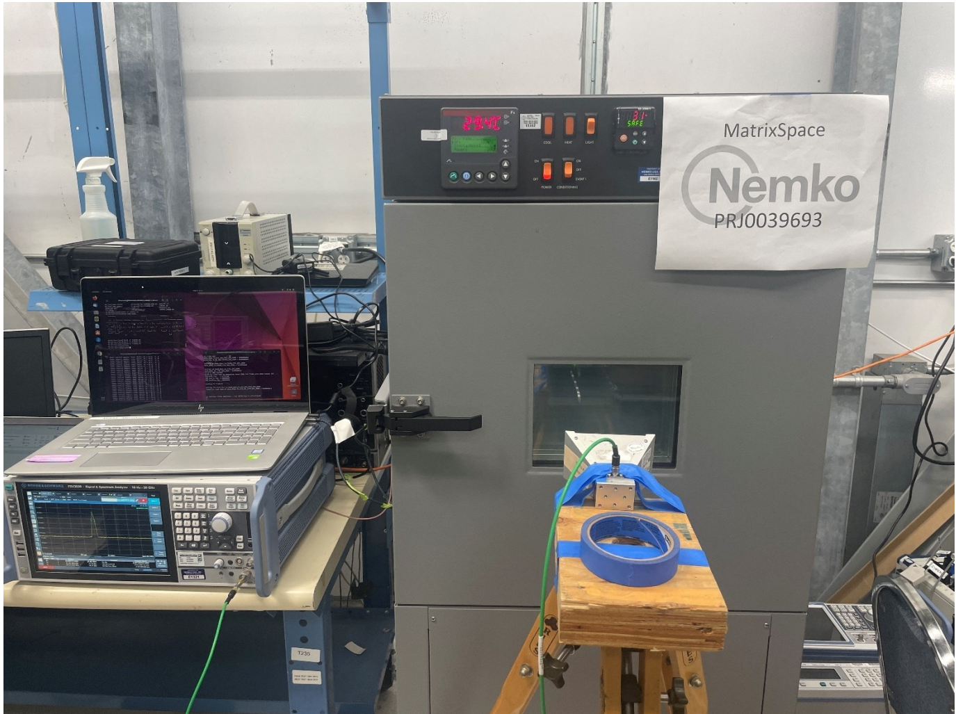
Figure 18 – Test setup: Frequency stability
