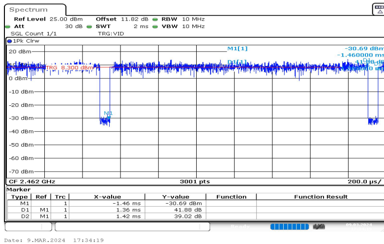
NTNV-11G-Ant1-2462
