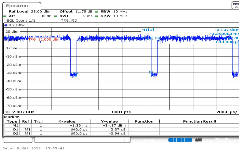
NTNV-11N40SISO-Ant1-2437
