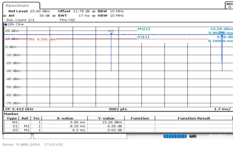
NTNV-11B-Ant1-2412
