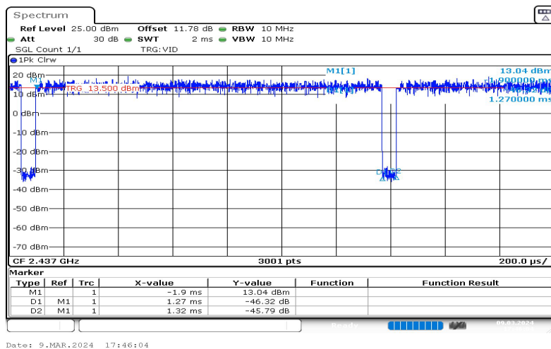
NTNV-11N20SISO-Ant1-2437
