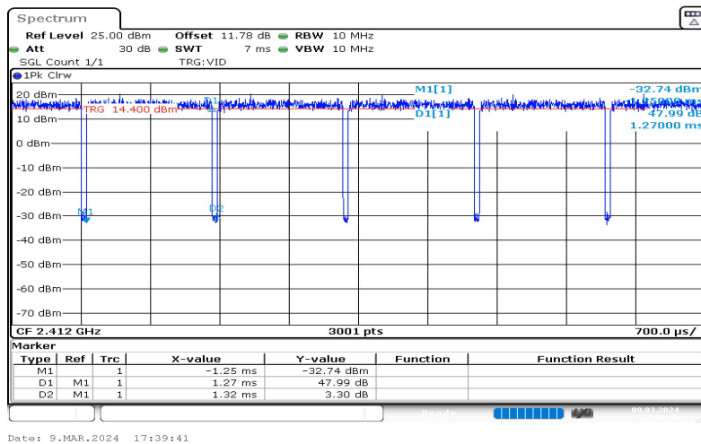
NTNV-11N20SISO-Ant1-2412
