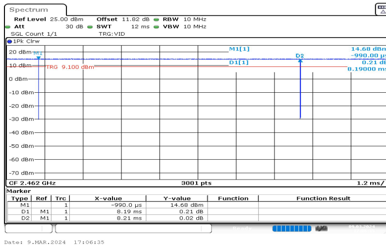
NTNV-11B-Ant1-2462
