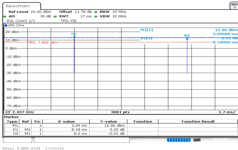
NTNV-11B-Ant1-2437
