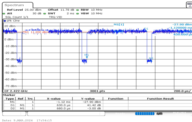
NTNV-11N40SISO-Ant1-2422
