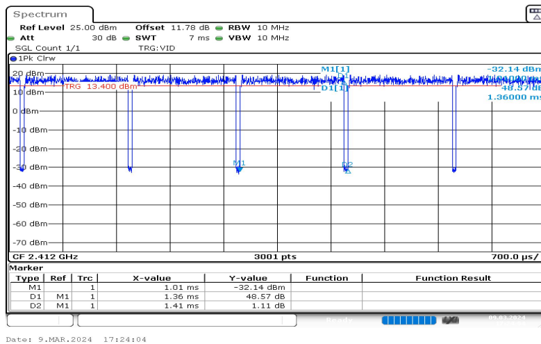
NTNV-11G-Ant1-2412
