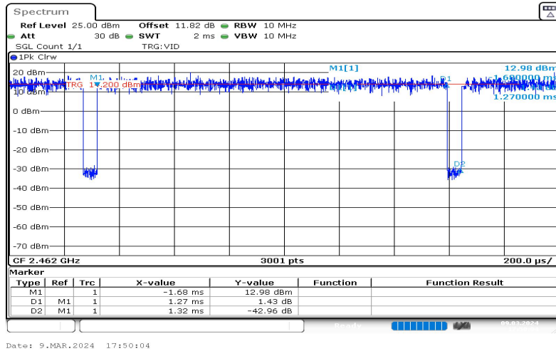
NTNV-11N20SISO-Ant1-2462
