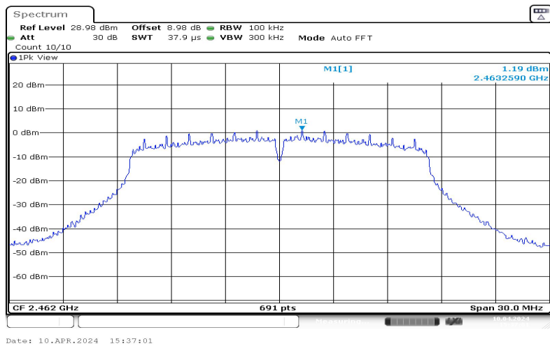
11G-Ant1-2462-0~Reference-1.19
