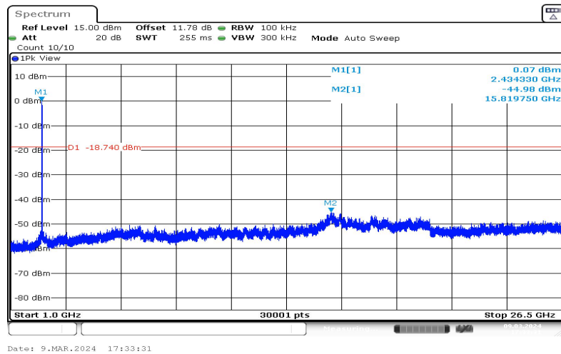
11G-Ant1-2437-1000~26500-1.26
