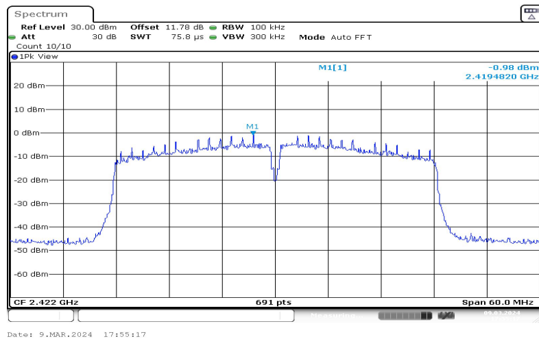
11N40SISO-Ant1-2422-0~Reference--0.98
