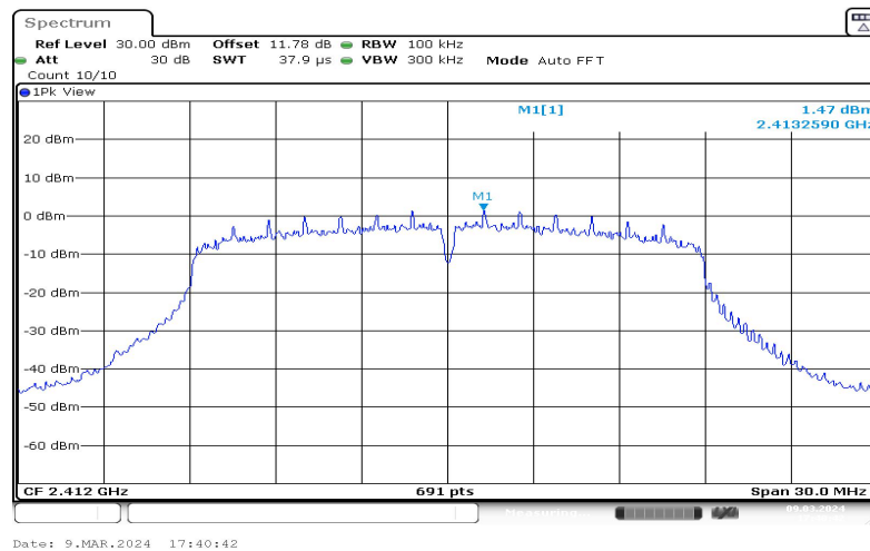
11N20SISO-Ant1-2412-0~Reference-1.47
