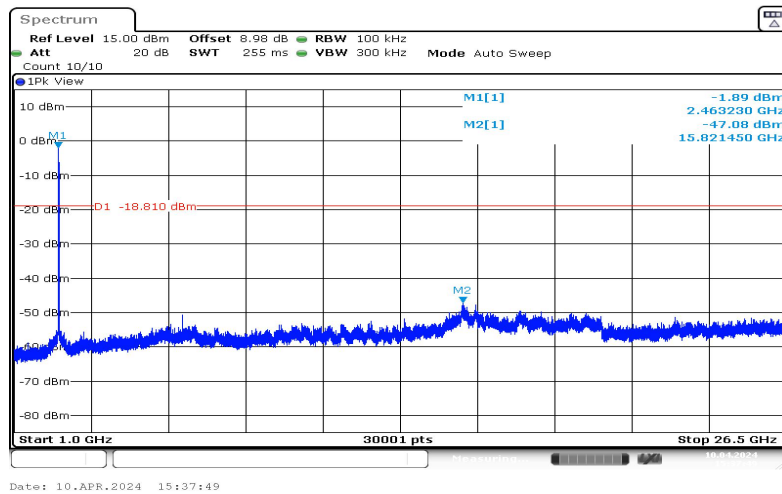
11G-Ant1-2462-1000~26500-1.19
