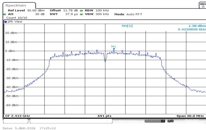
11G-Ant1-2412-0~Reference-1.38
