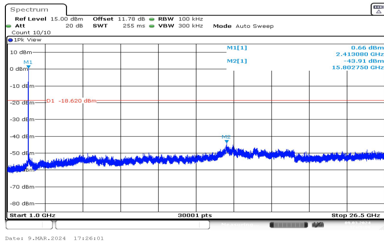
11G-Ant1-2412-1000~26500-1.38
