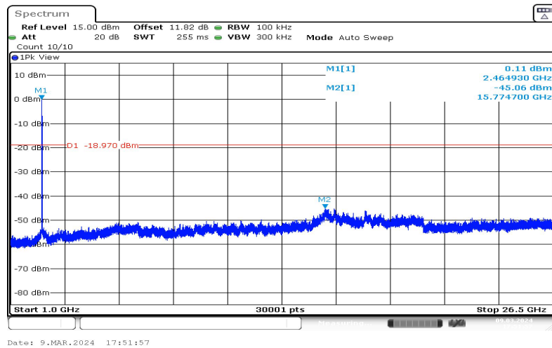
11N20SISO-Ant1-2462-1000~26500-1.03
