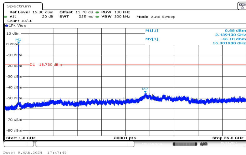
11N20SISO-Ant1-2437-1000~26500-1.27
