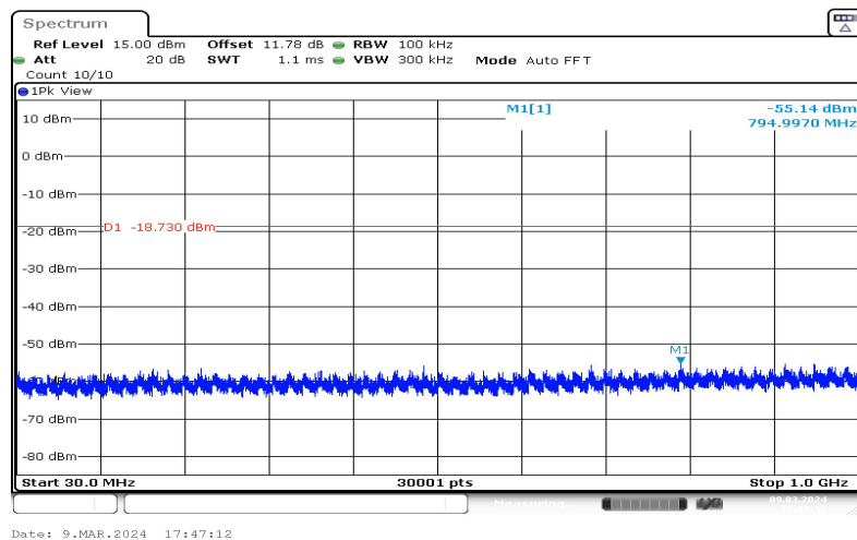
11N20SISO-Ant1-2437-30~1000-1.27
