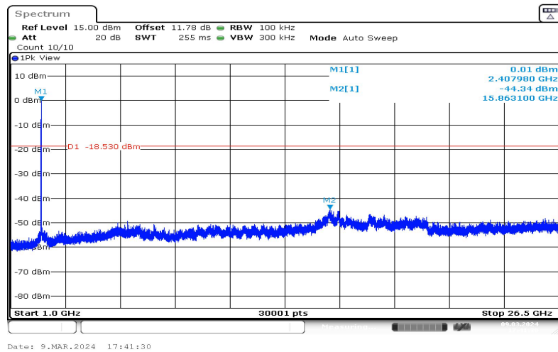
11N20SISO-Ant1-2412-1000~26500-1.47
