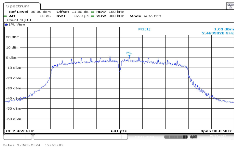
11N20SISO-Ant1-2462-0~Reference-1.03
