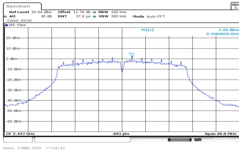
11G-Ant1-2437-0~Reference-1.26
