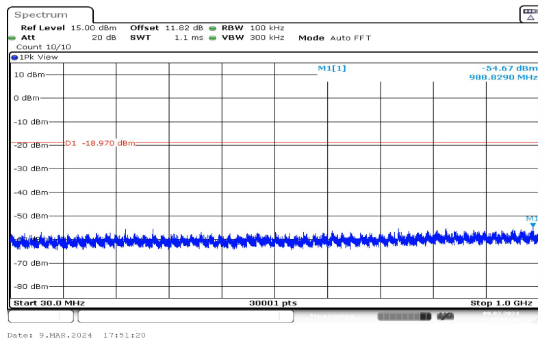
11N20SISO-Ant1-2462-30~1000-1.03
