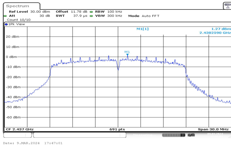
11N20SISO-Ant1-2437-0~Reference-1.27
