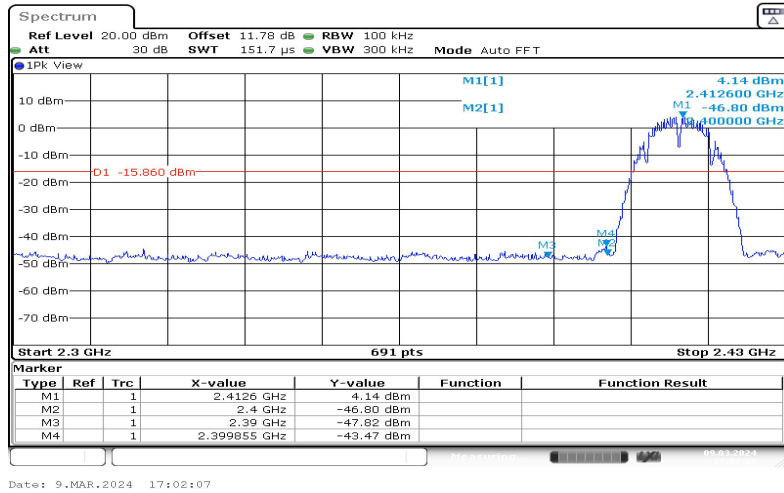
11B-Ant1-Low-2412-4.14
