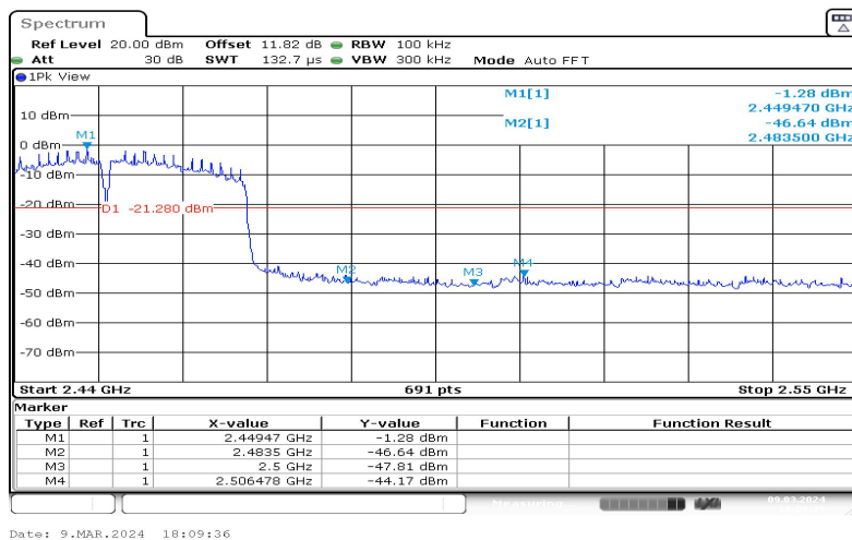
11N40SISO-Ant1-High-2452--1.28
