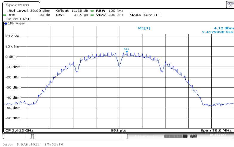
11B-Ant1-2412-0~Reference-4.12
