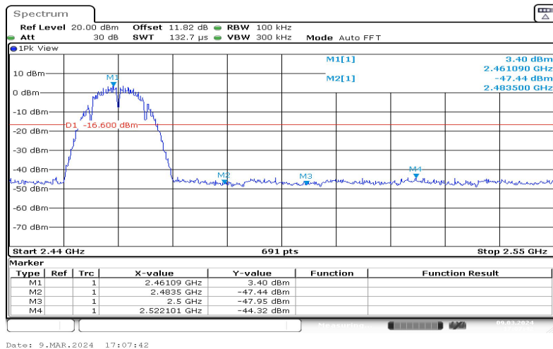
11B-Ant1-High-2462-3.40
