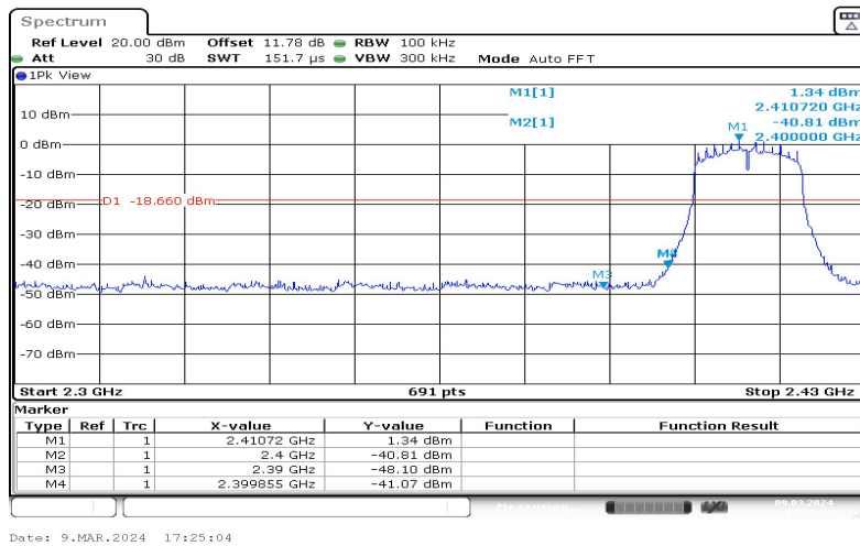
11G-Ant1-Low-2412-1.34
