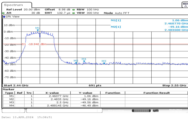
11G-Ant1-High-2462-1.06
