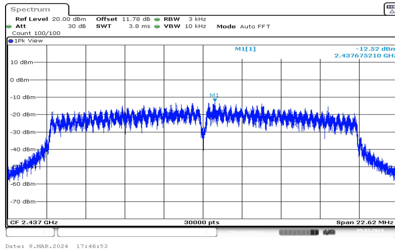
11N20SISO-Ant1-2437--12.52-0.00-0.00-0.00
