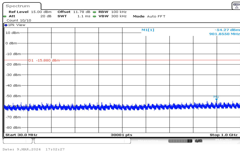
11B-Ant1-2412-30~1000-4.12
