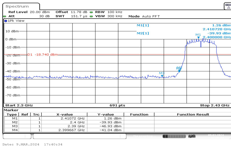
11N20SISO-Ant1-Low-2412-1.26
