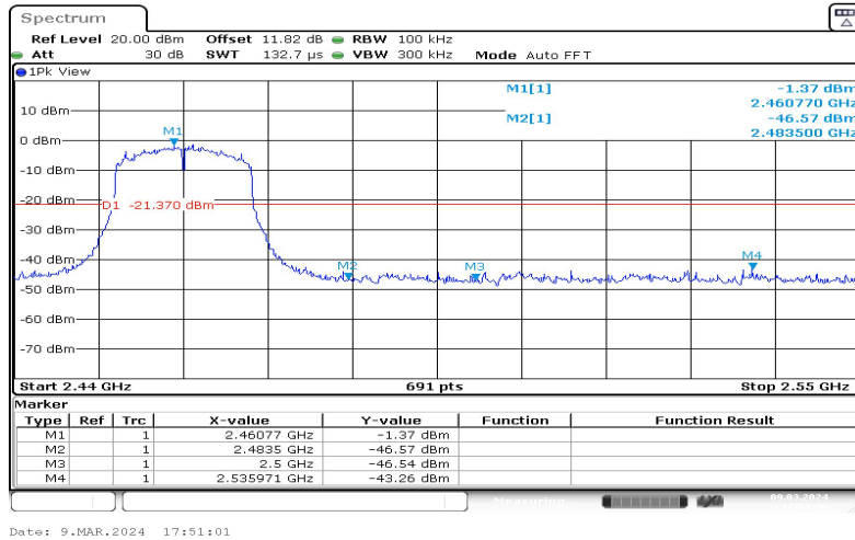
11N20SISO-Ant1-High-2462--1.37
