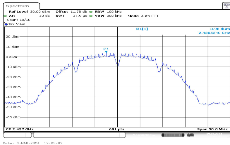
11B-Ant1-2437-0~Reference-3.96
