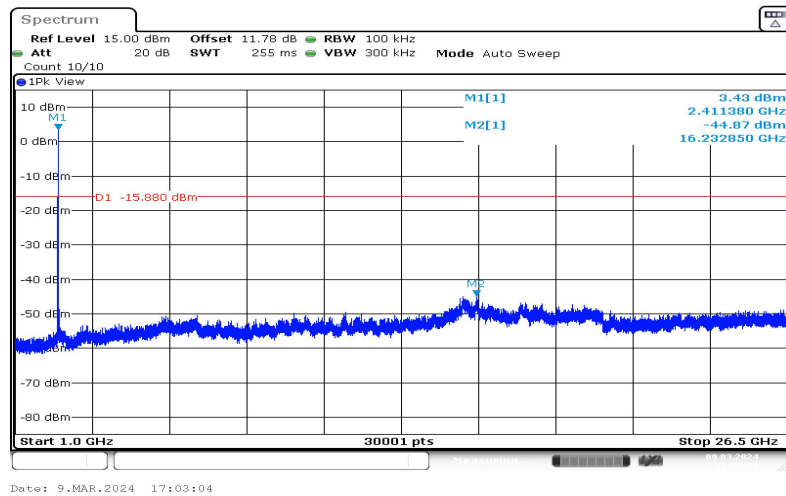
11B-Ant1-2412-1000~26500-4.12
