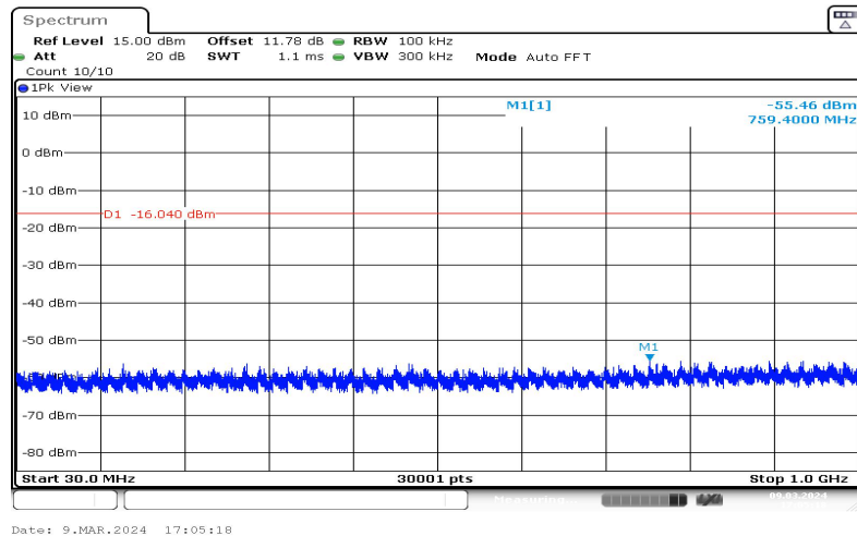
11B-Ant1-2437-30~1000-3.96
