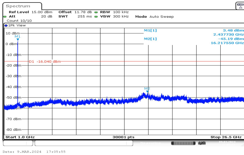
11B-Ant1-2437-1000~26500-3.96
