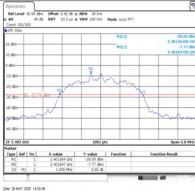
3DH5-Ant1-2402
