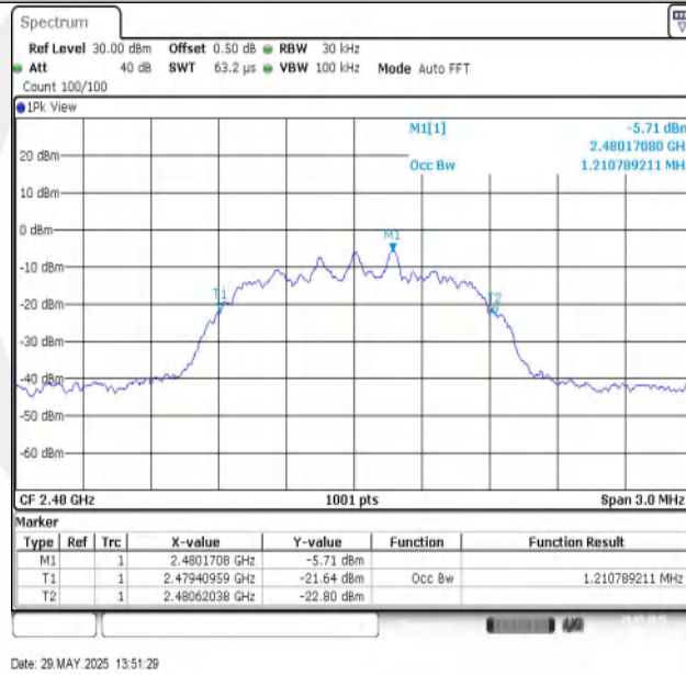
2DH5-Ant1-2480
