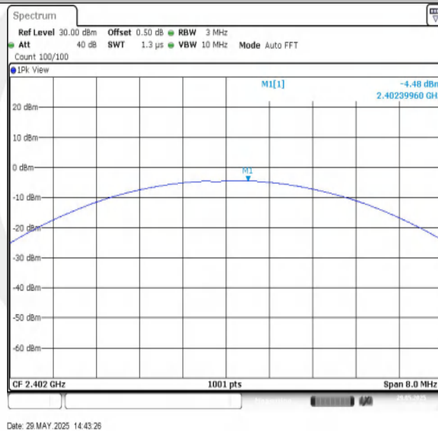
2DH5-Ant1-2402-PASS
