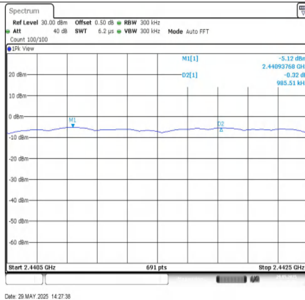
3DH5-Ant1-Hop-PASS
