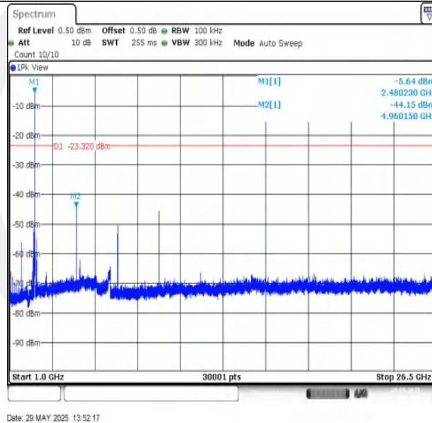
2DH5-Ant1-2480-1000~26500-PASS
