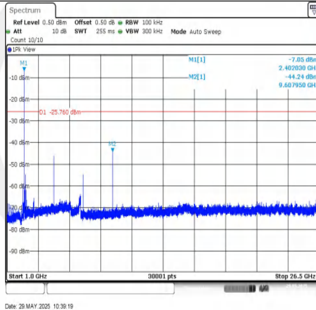
2DH5-Ant1-2402-1000~26500-PASS
