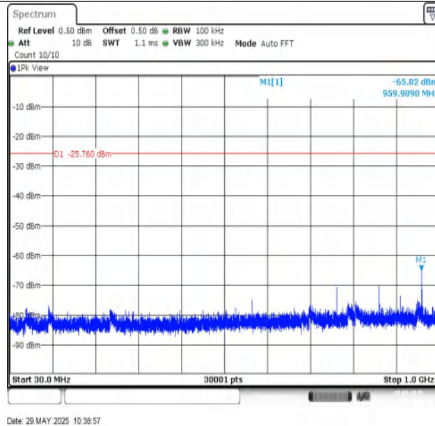
2DH5-Ant1-2402-30~1000-PASS
