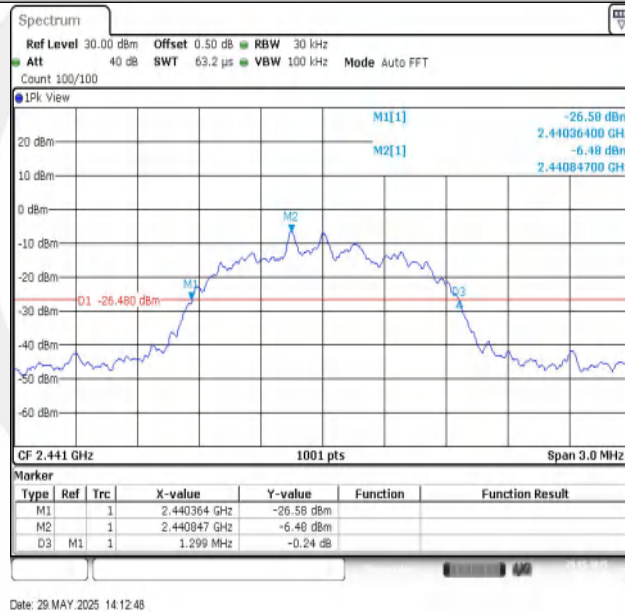
3DH5-Ant1-2441
