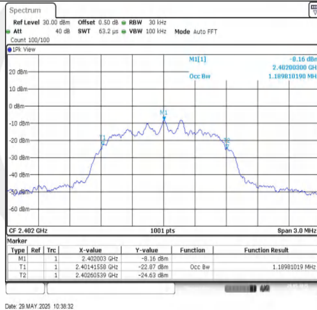
2DH5-Ant1-2402
