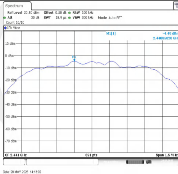
3DH5-Ant1-2441-0~Reference-PASS
