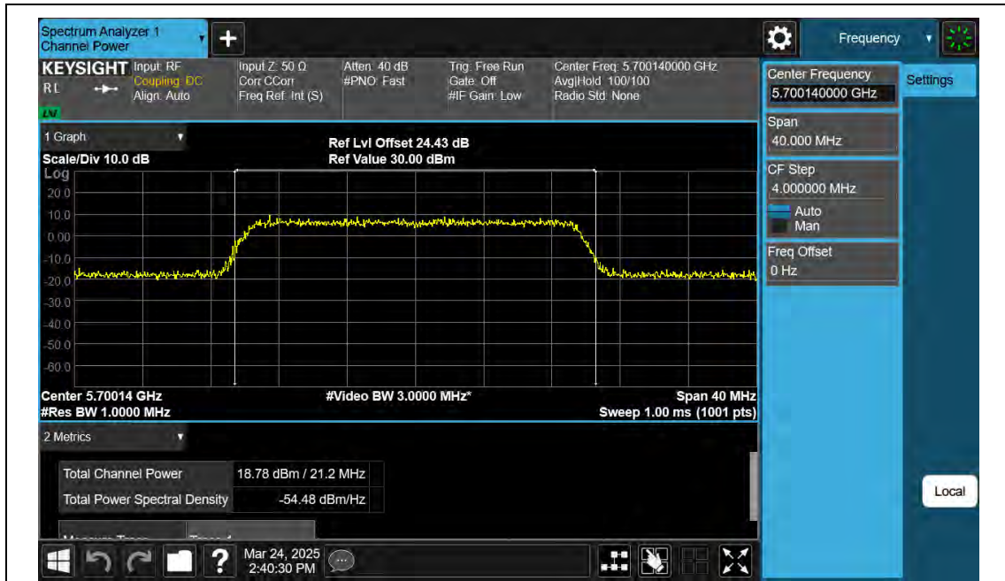
11AX20SISO-Ant2-5700-PASS
