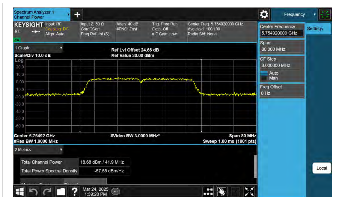
11AC40SISO-Ant2-5755-PASS
