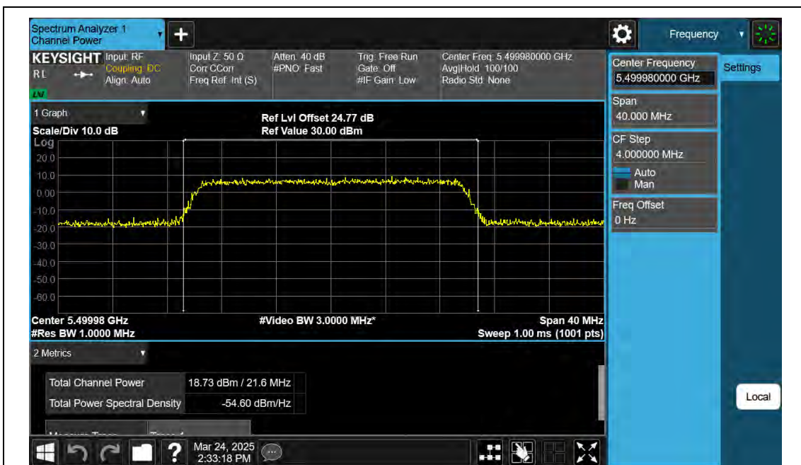
11AX20SISO-Ant2-5500-PASS
