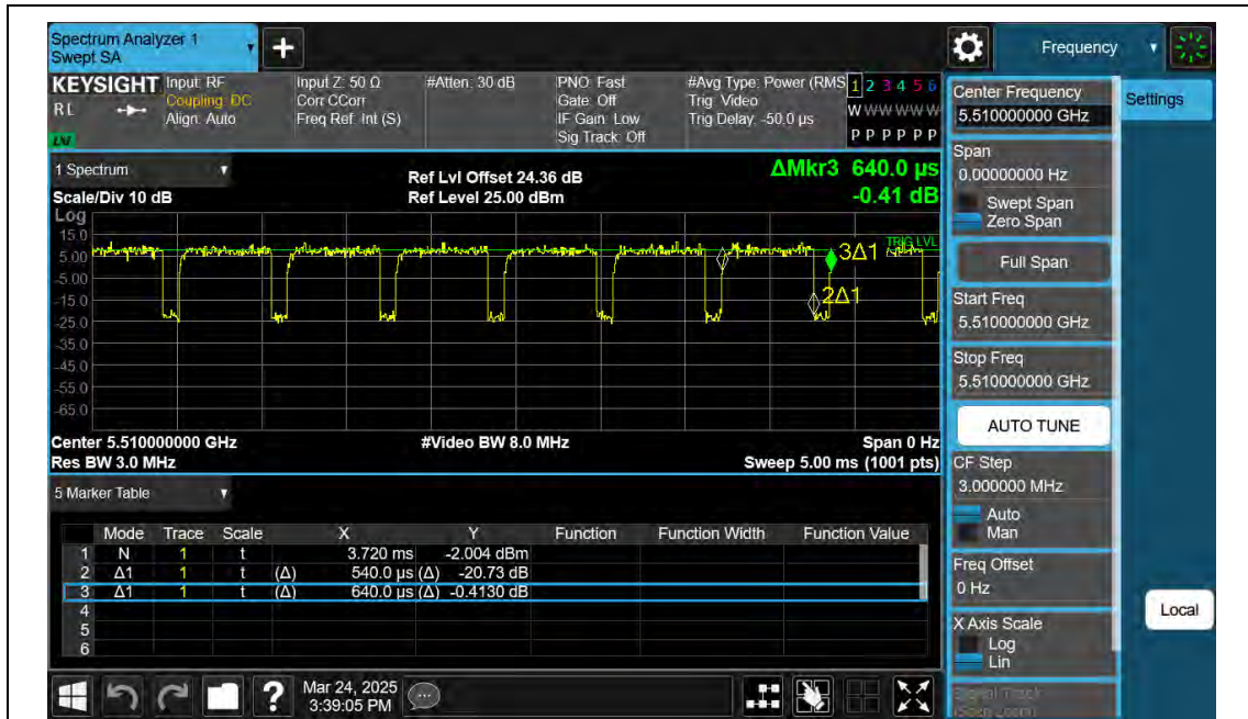
NTNV-11AX40SISO-Ant2-5510
