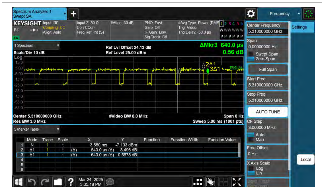
NTNV-11AX40SISO-Ant2-5310
