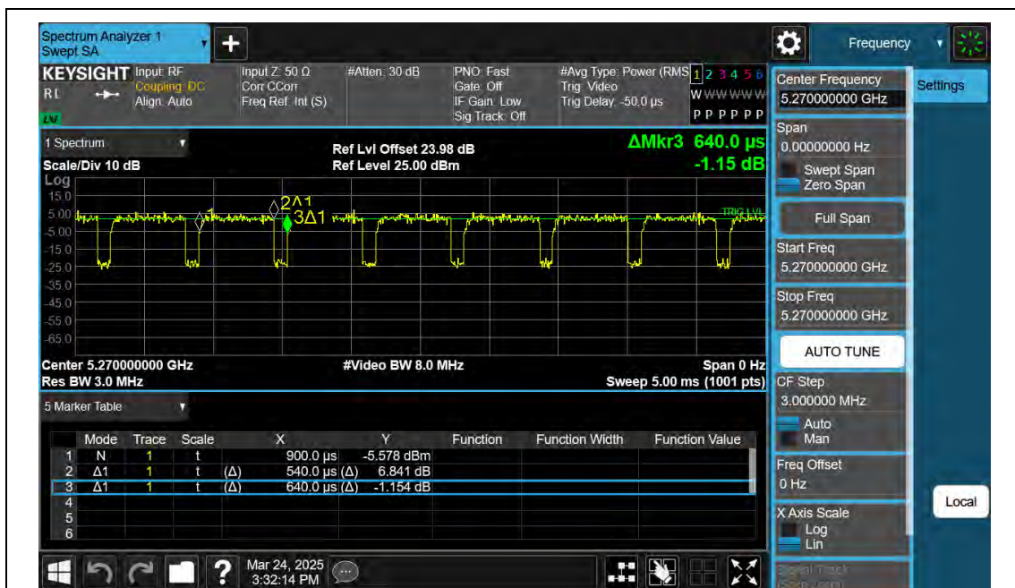
NTNV-11AX40SISO-Ant2-5270
