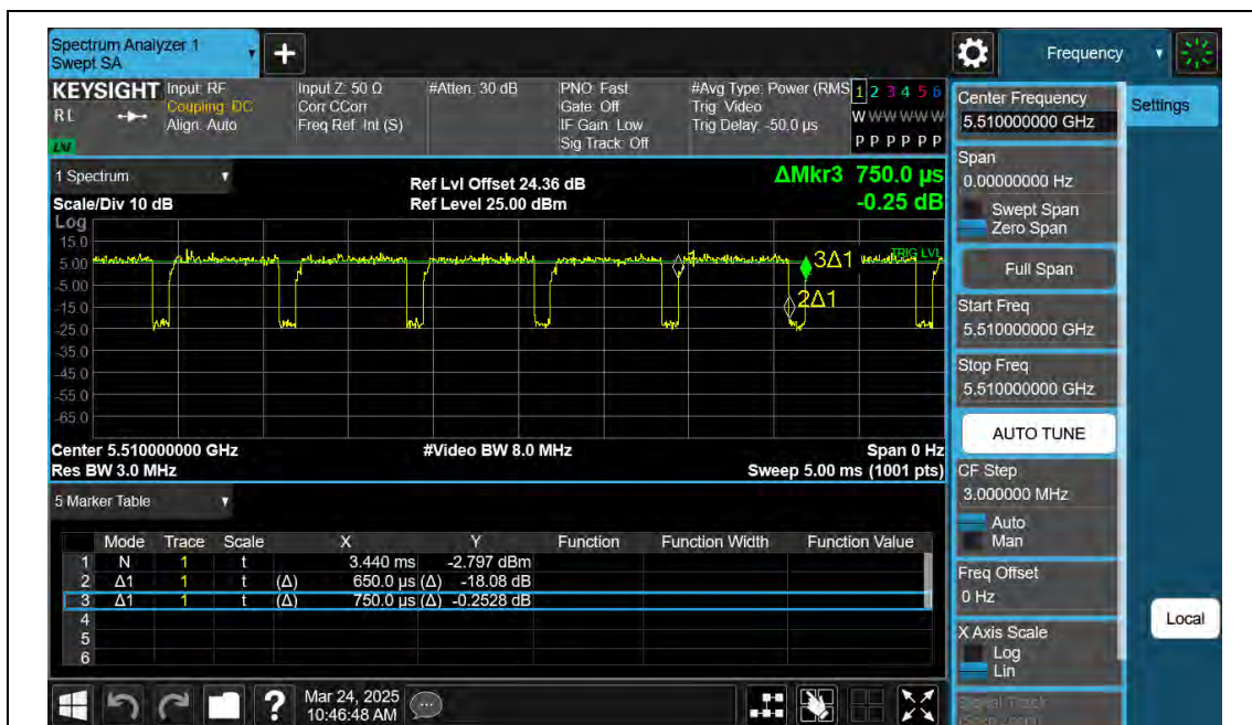
NTNV-11N40SISO-Ant2-5510
