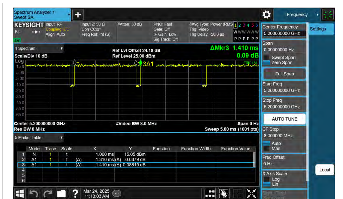
NTNV-11AC20SISO-Ant2-5200
