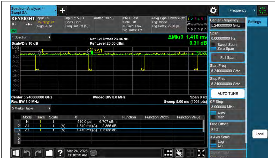
NTNV-11AC20SISO-Ant2-5240
