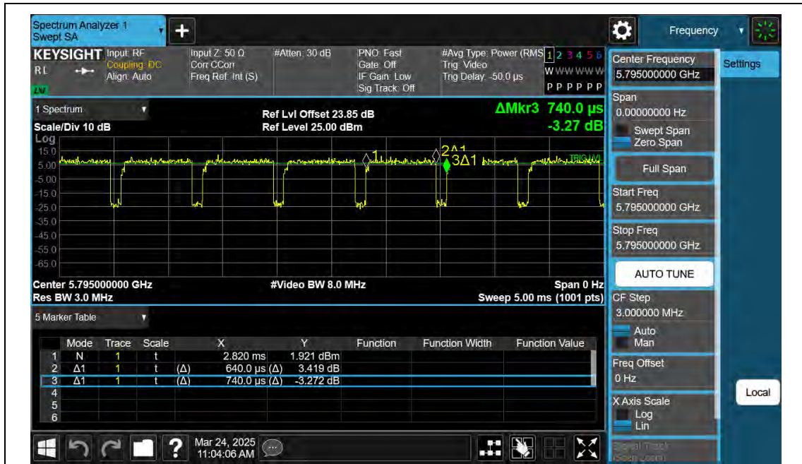
NTNV-11N40SISO-Ant2-5795
