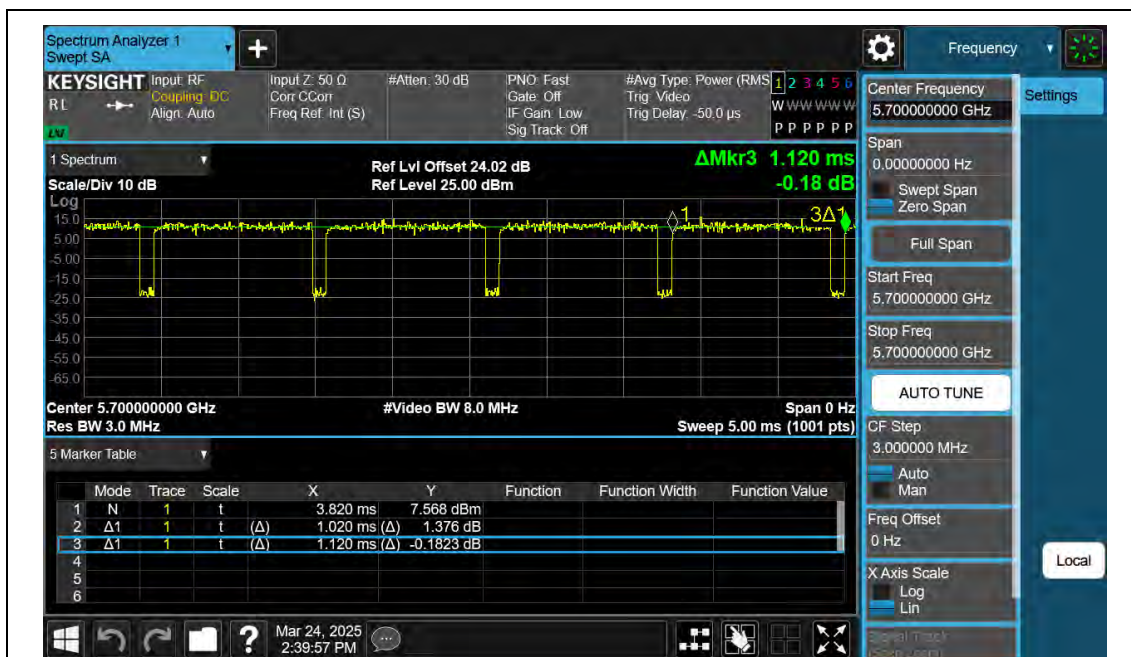
NTNV-11AX20SISO-Ant2-5700
