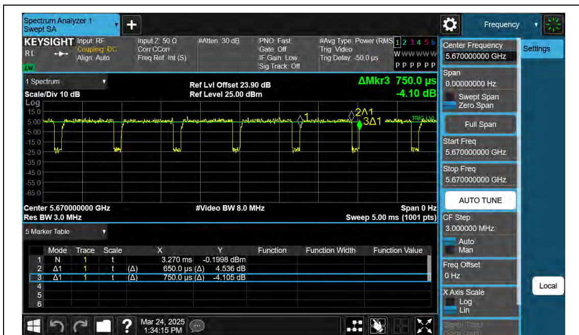
NTNV-11AC40SISO-Ant2-5670
