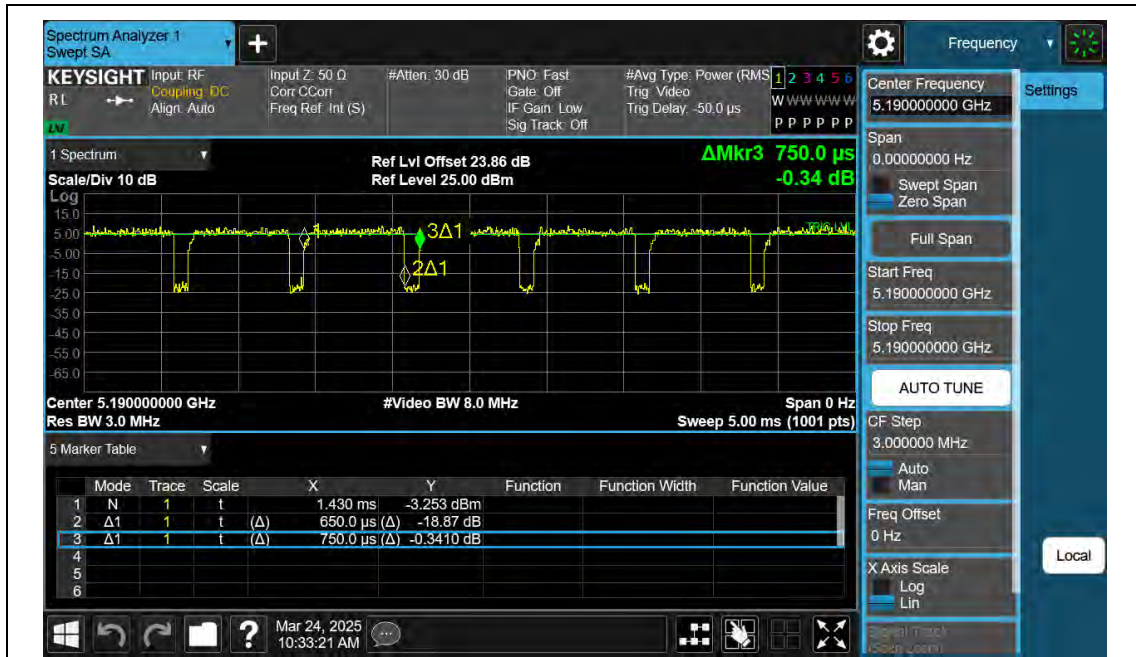
NTNV-11N40SISO-Ant2-5190
