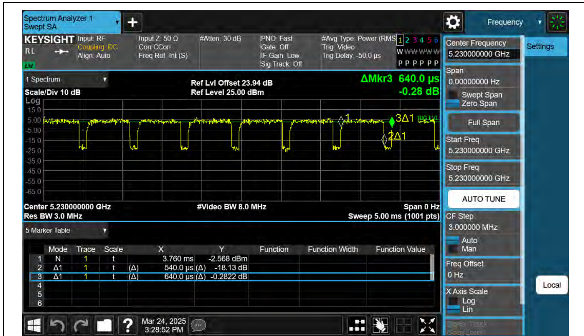
NTNV-11AX40SISO-Ant2-5230
