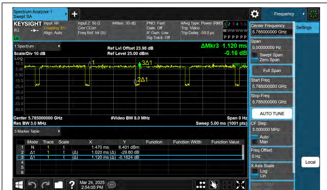
NTNV-11AX20SISO-Ant2-5785
