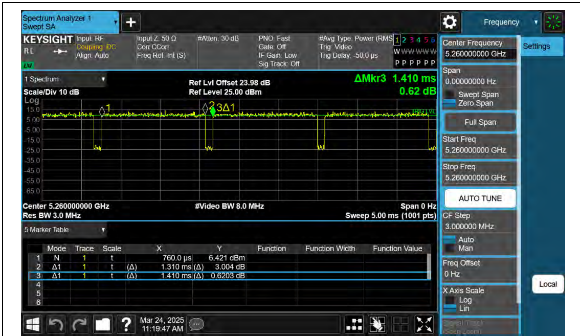
NTNV-11AC20SISO-Ant2-5260
