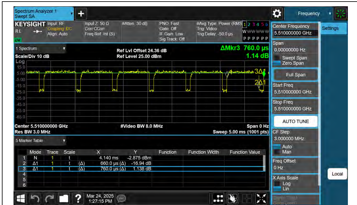
NTNV-11AC40SISO-Ant2-5510
