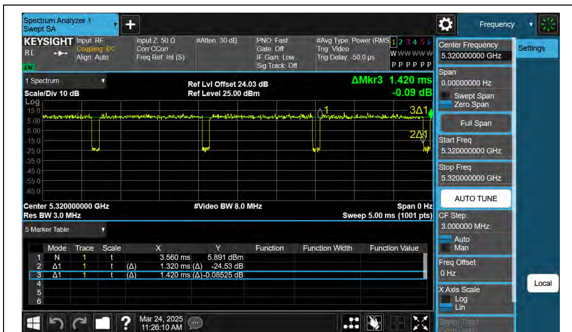
NTNV-11AC20SISO-Ant2-5320
