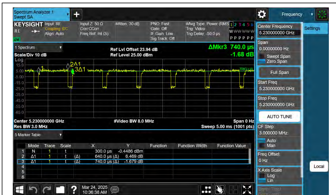
NTNV-11N40SISO-Ant2-5230
