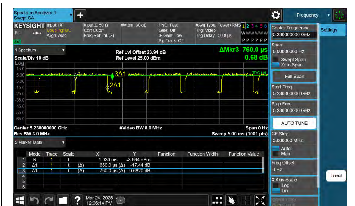
NTNV-11AC40SISO-Ant2-5230
