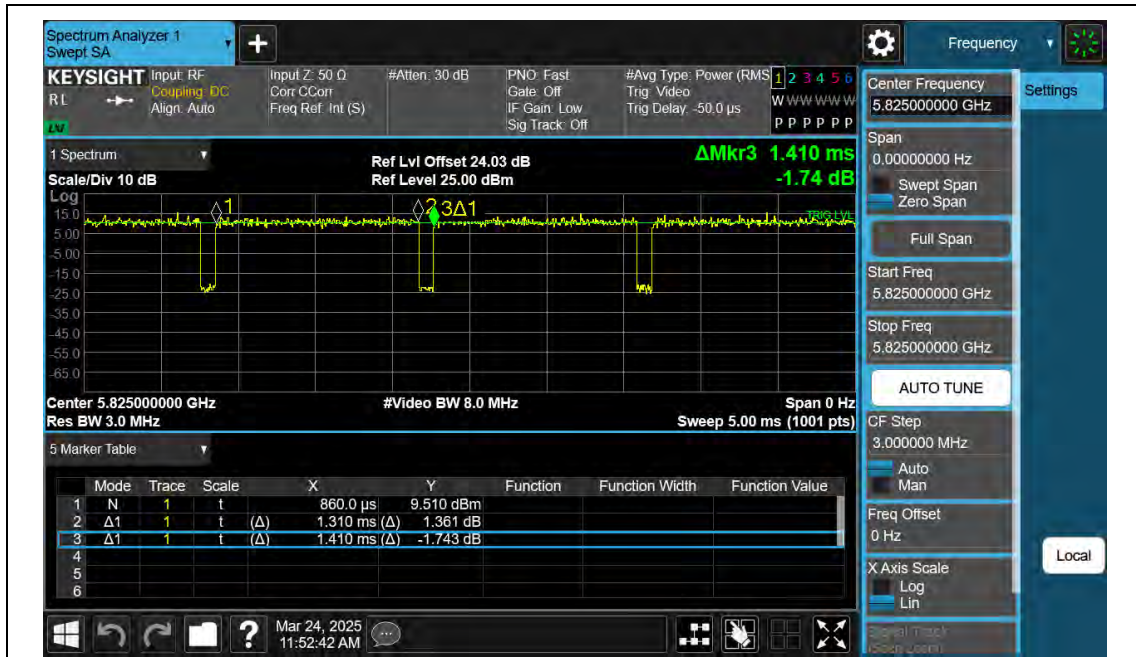
NTNV-11AC20SISO-Ant2-5825
