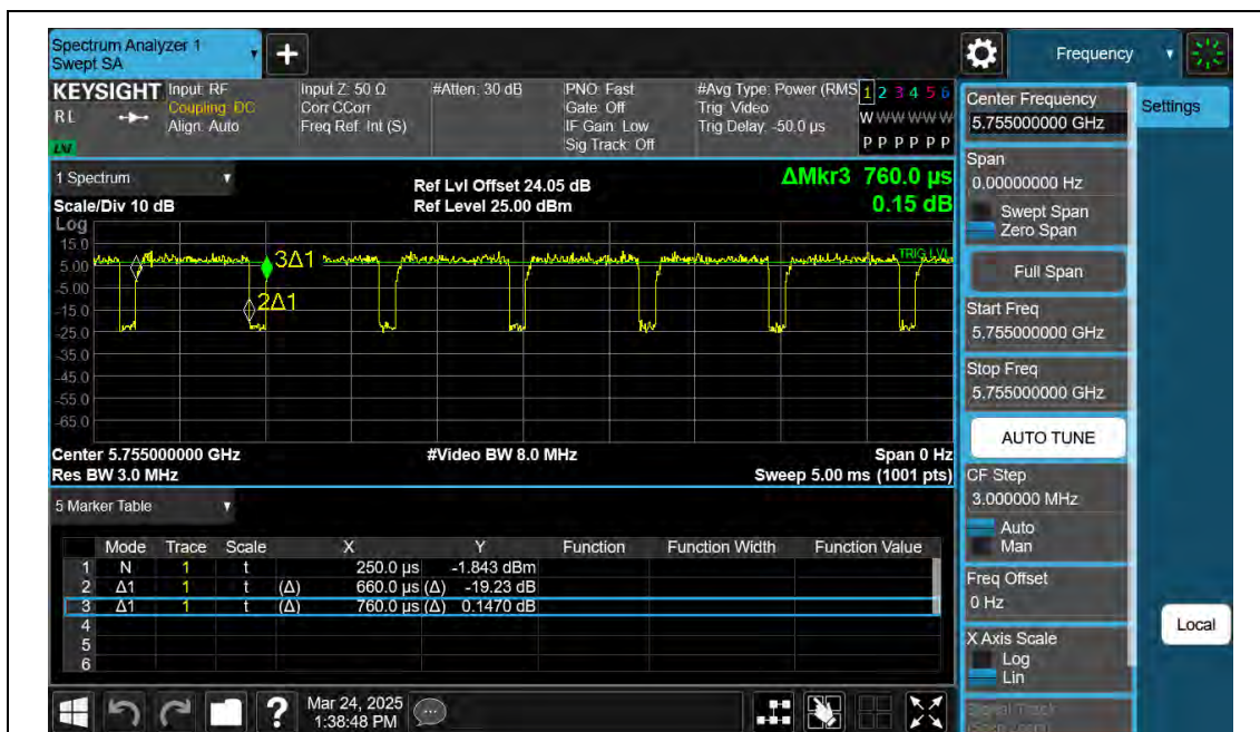
NTNV-11AC40SISO-Ant2-5755
