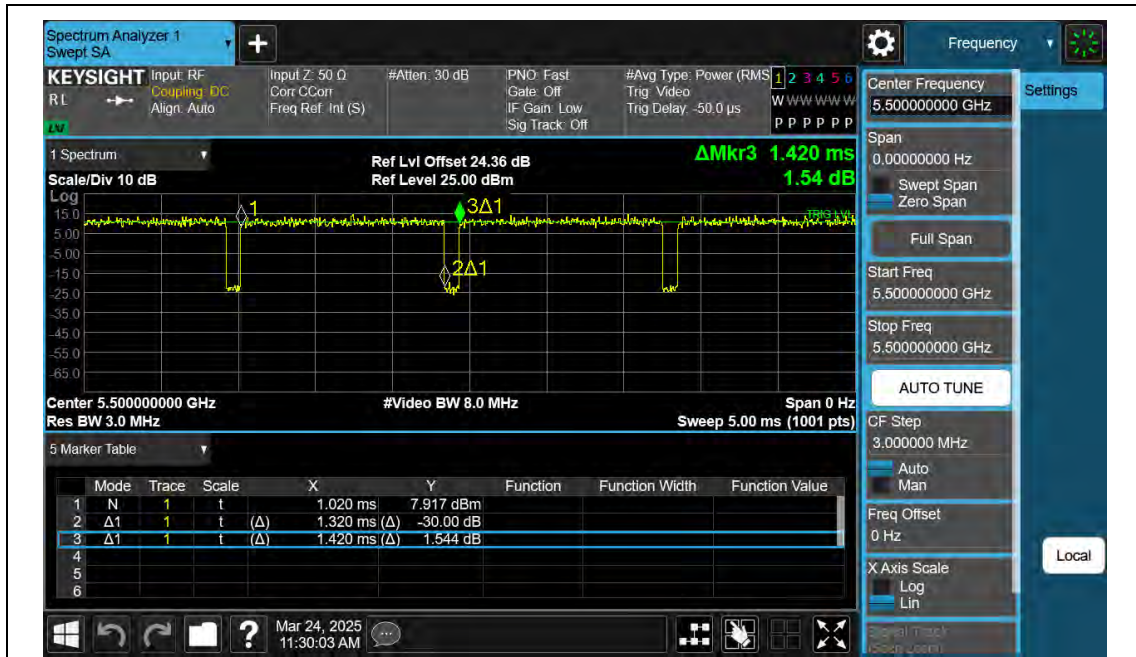
NTNV-11AC20SISO-Ant2-5500
