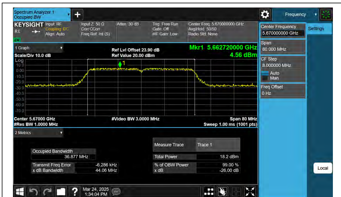
11AC40SISO-Ant2-5670
