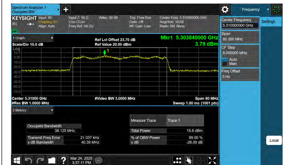
11AX40SISO-Ant1-5510
