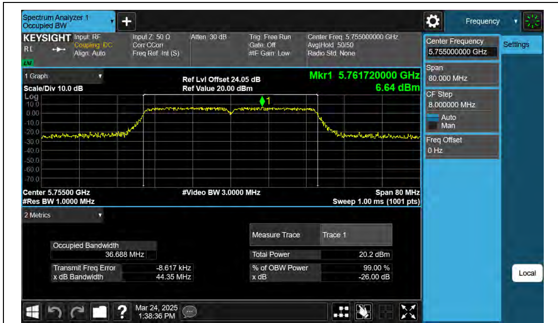
11AC40SISO-Ant2-5755
