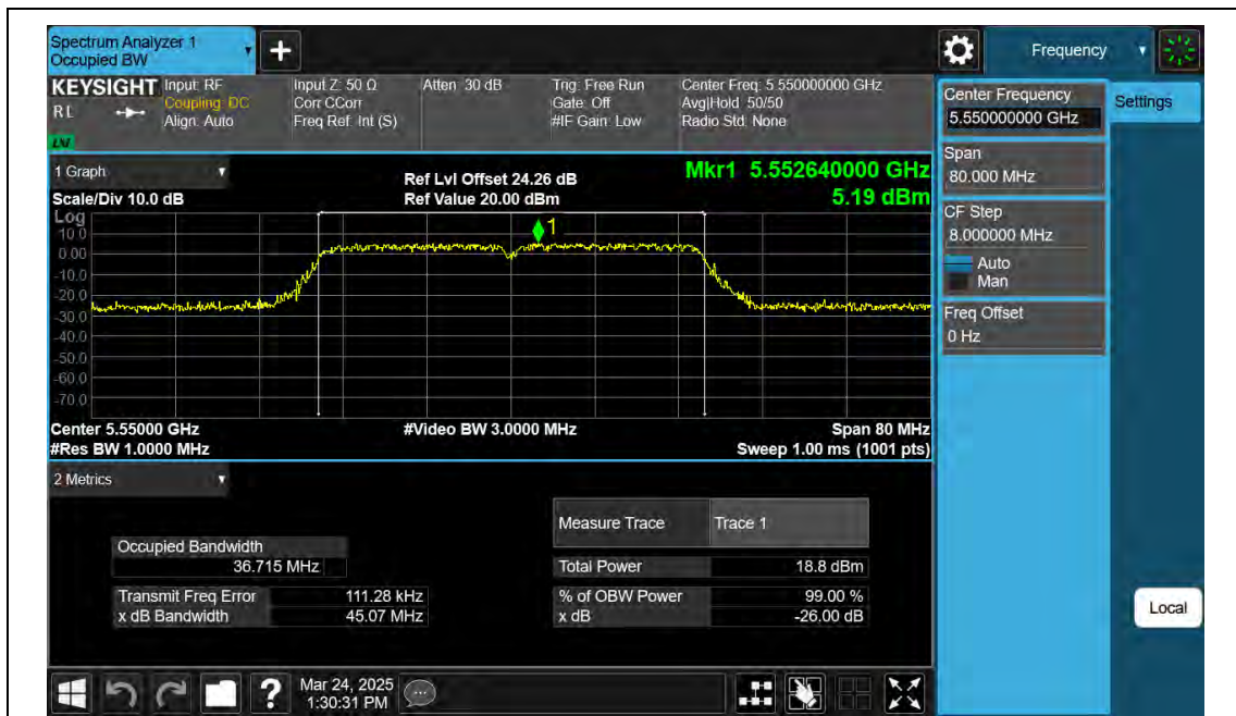
11AC40SISO-Ant2-5550
