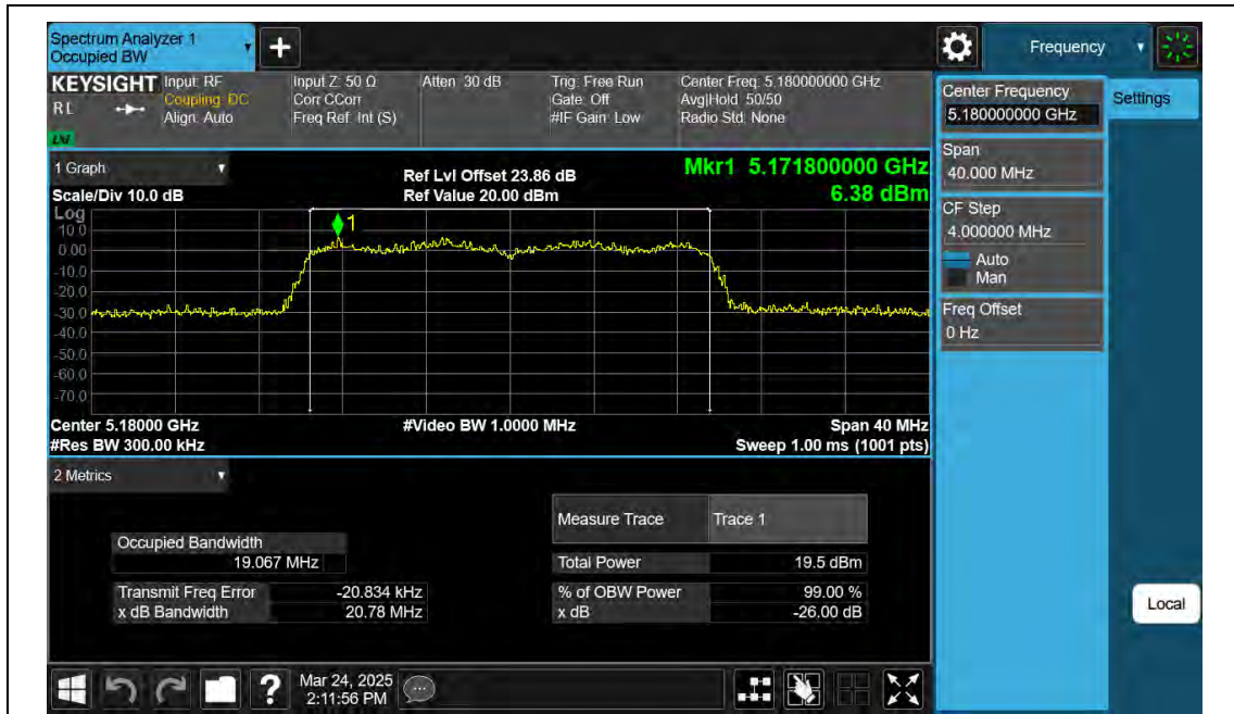
11AX20SISO-Ant2-5180
