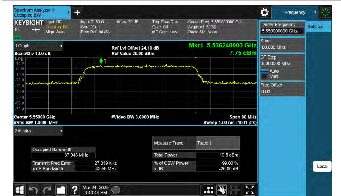
11AX40SISO-Ant1-5670
