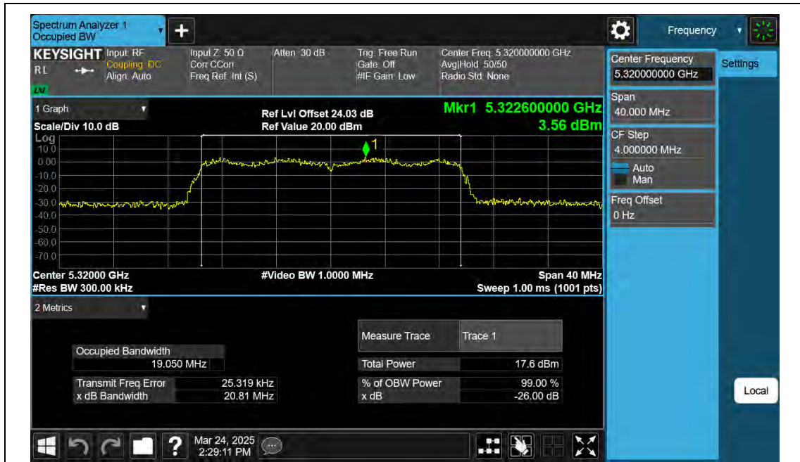
11AX20SISO-Ant2-5320
