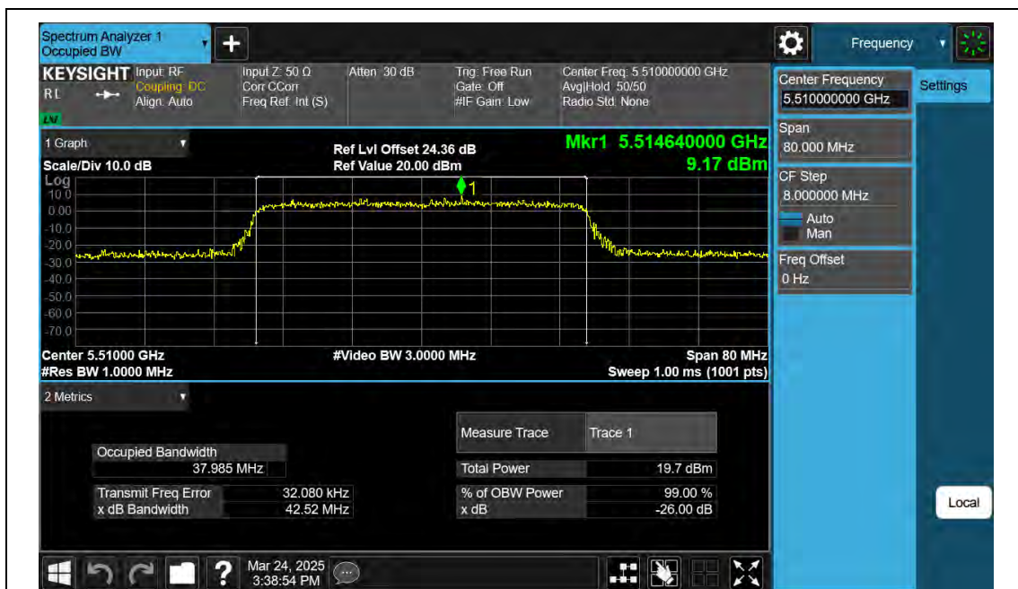
11AX40SISO-Ant2-5510
