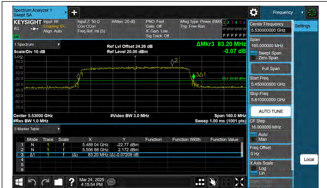
11AX80SISO-Ant2-5530
