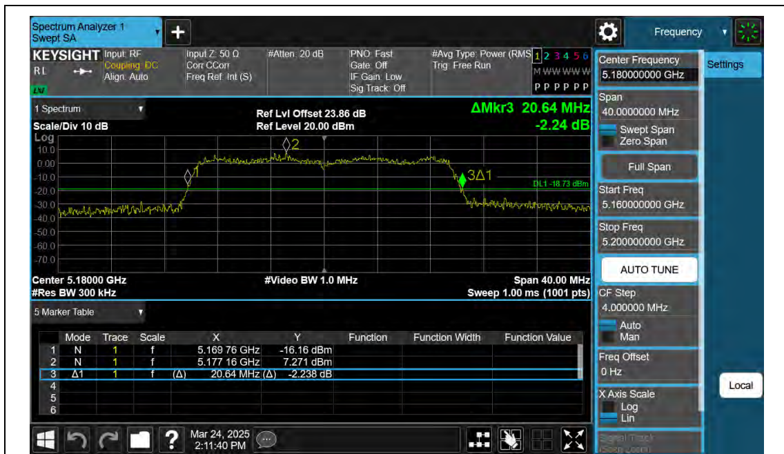
11AX20SISO-Ant2-5180
