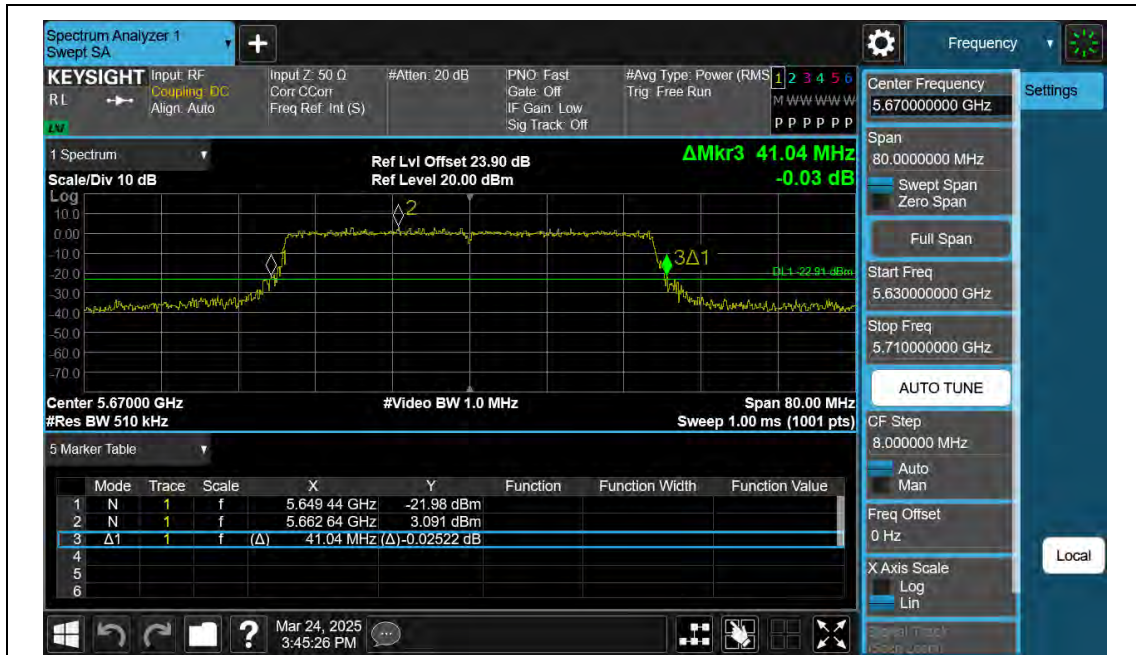
11AX40SISO-Ant2-5670
