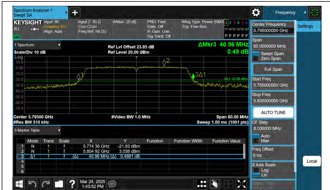
11AC40SISO-Ant2-5795
