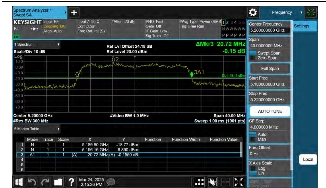
11AX20SISO-Ant2-5200
