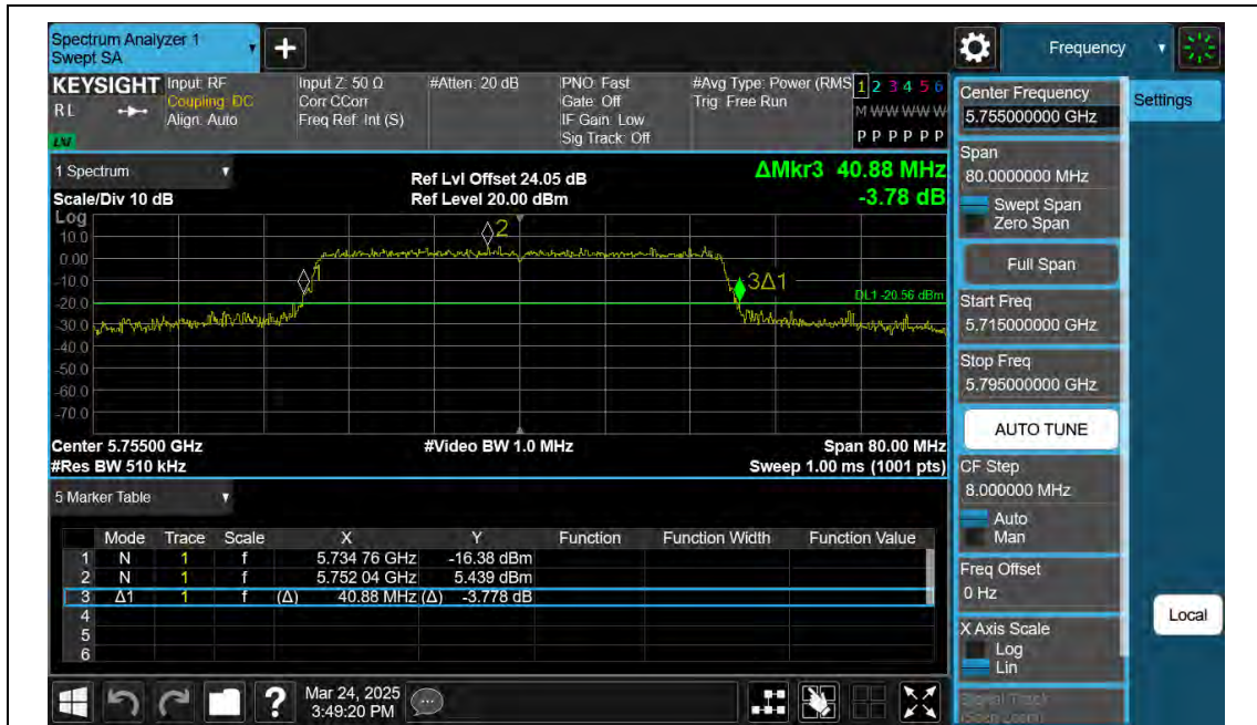
11AX40SISO-Ant2-5755
