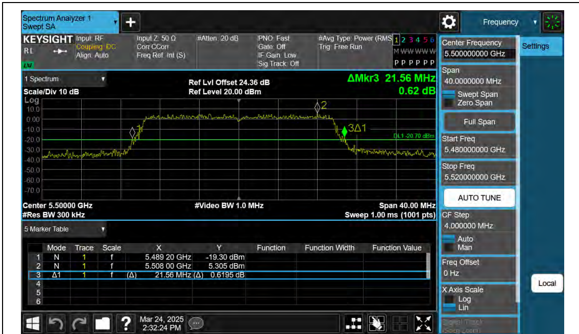
11AX20SISO-Ant2-5500
