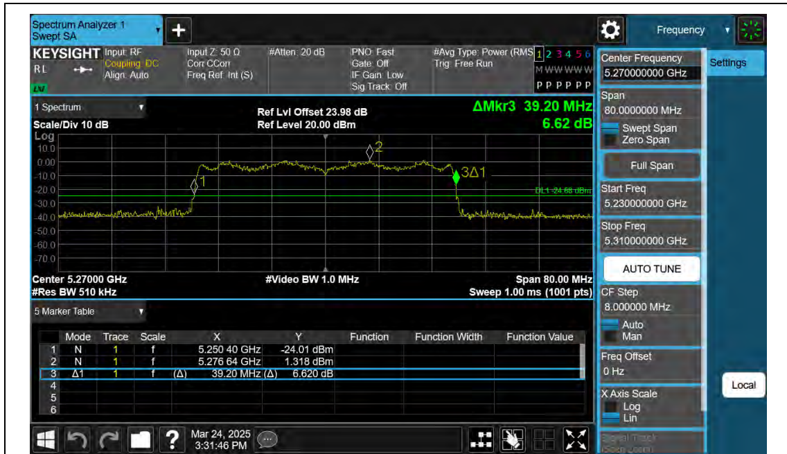
11AX40SISO-Ant2-5270
