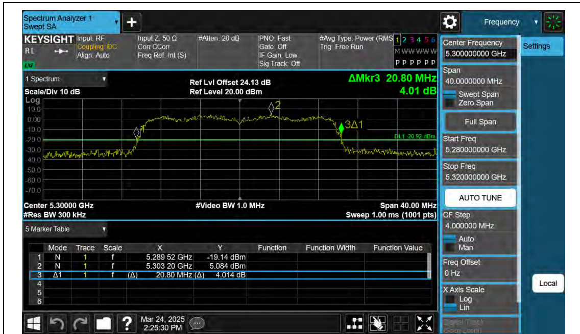
11AX20SISO-Ant2-5300
