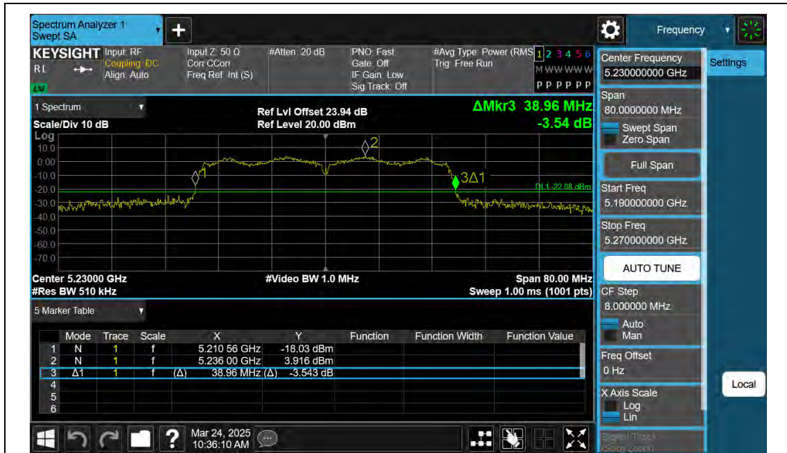
11N40SISO-Ant2-5230
