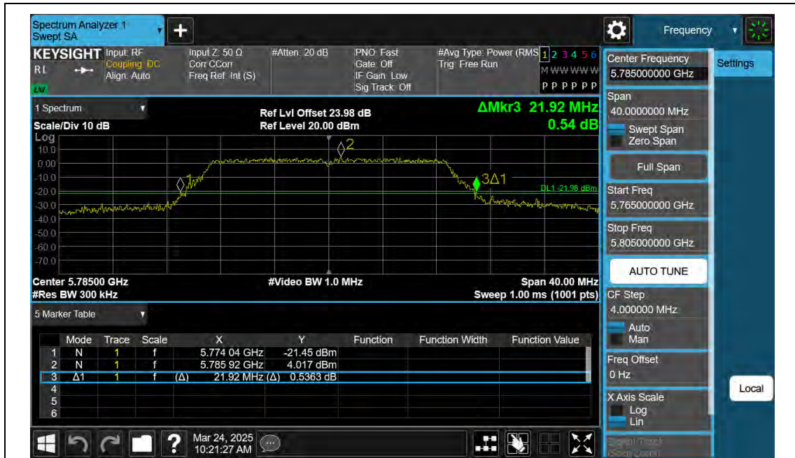
11N20SISO-Ant2-5785
