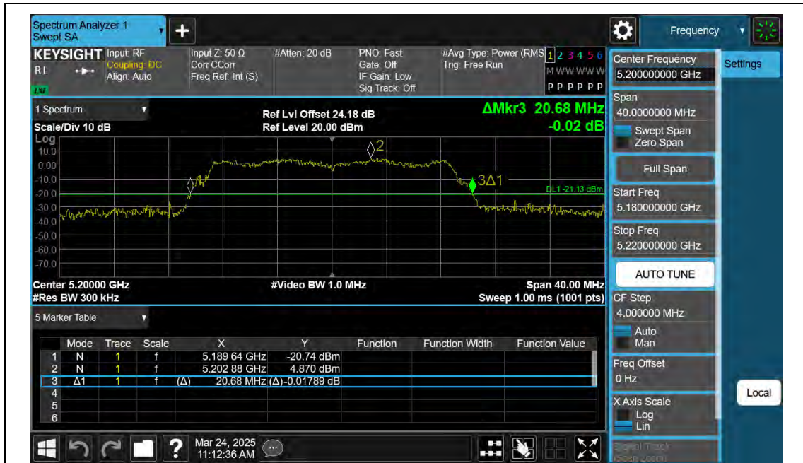
11AC20SISO-Ant2-5200
