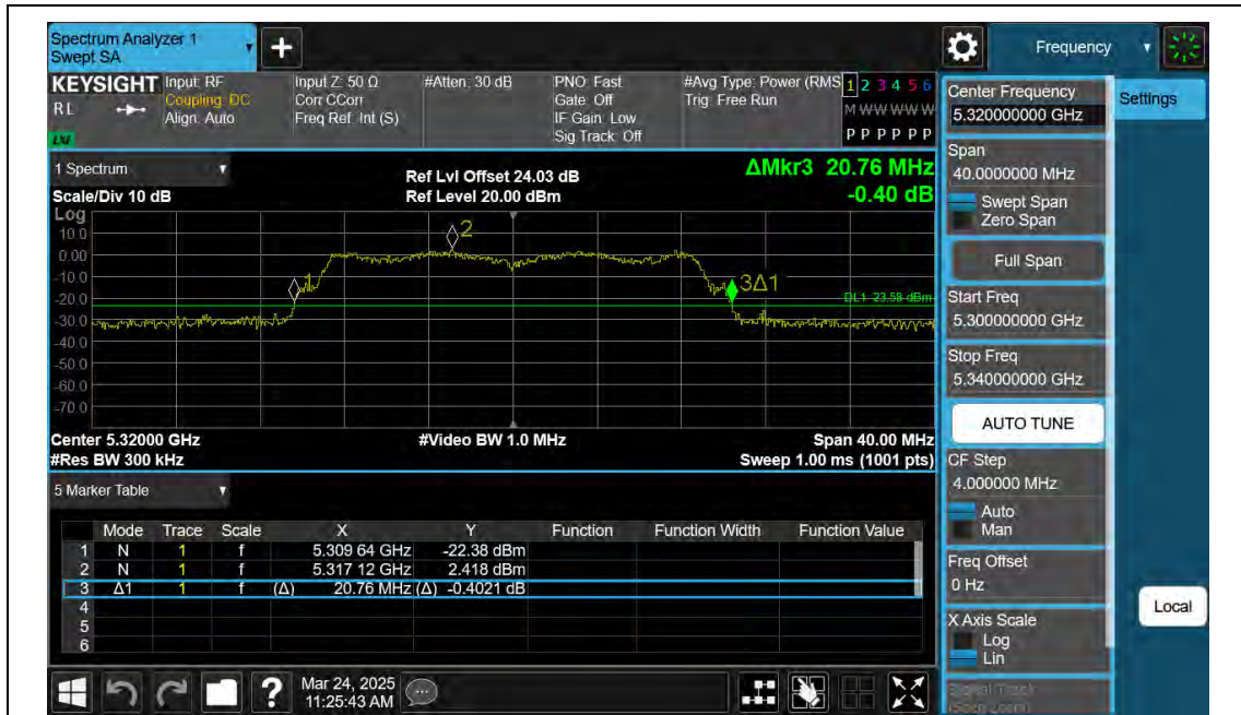
11AC20SISO-Ant2-5320
