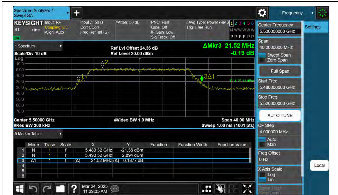
11AC20SISO-Ant2-5500
