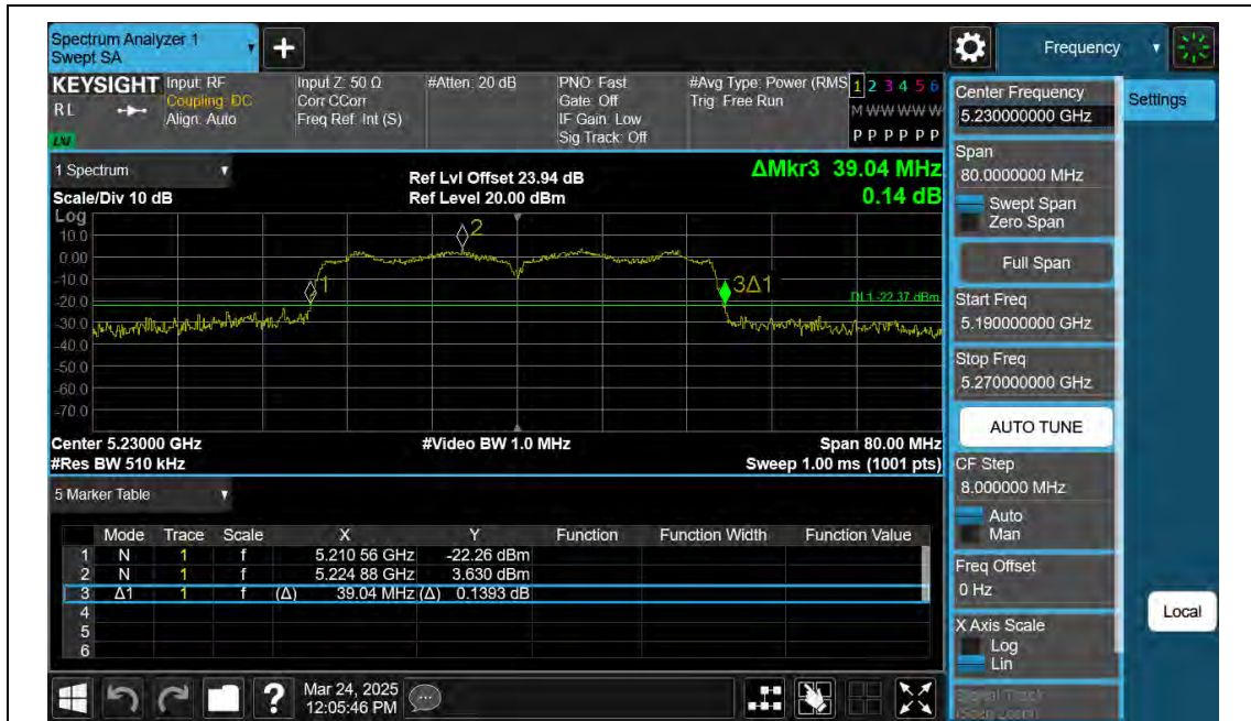
11AC40SISO-Ant2-5230
