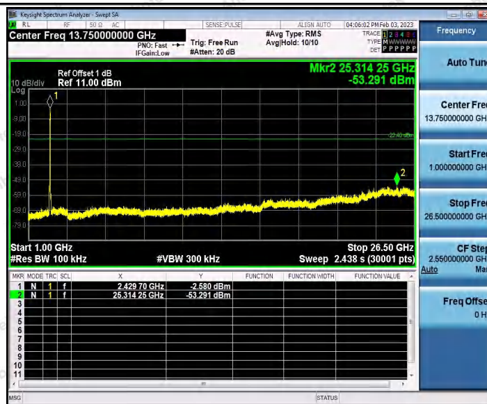
11AX40_Ant2_2437_0~Reference
