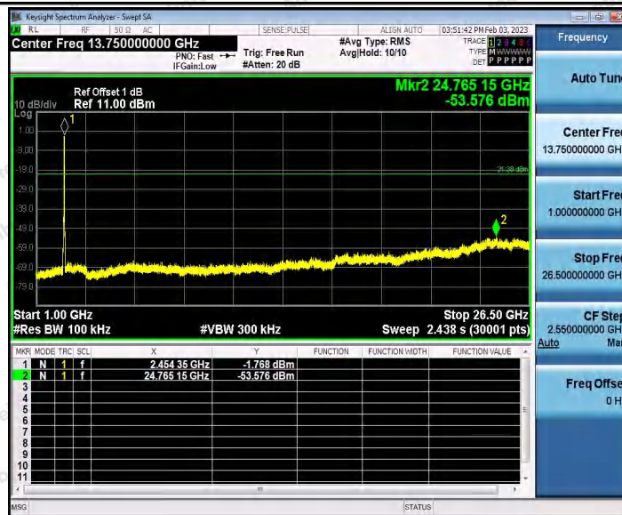
11N40_Ant2_2452_0~Reference
