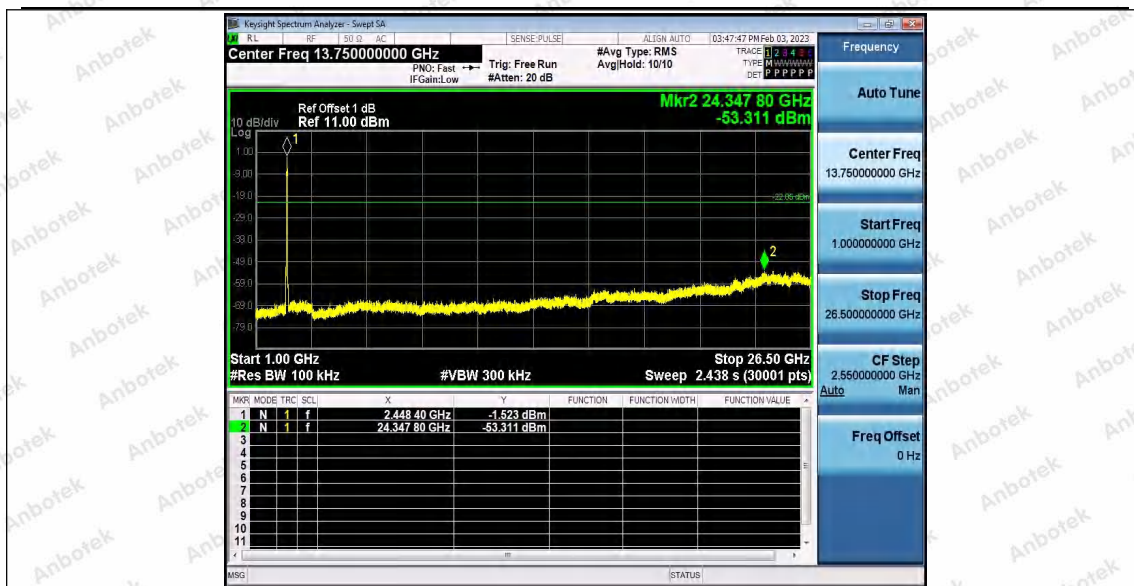
11N40_Ant2_2437_0~Reference
