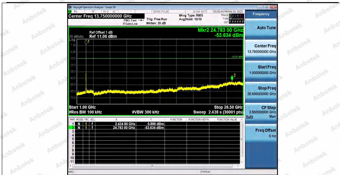
11AX20_Ant2_2437_0~Reference
