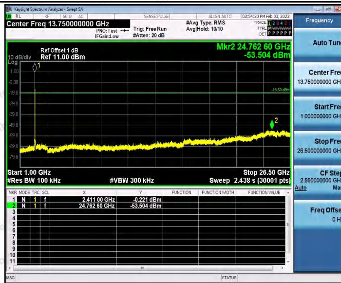
11AX20_Ant2_2412_0~Reference
