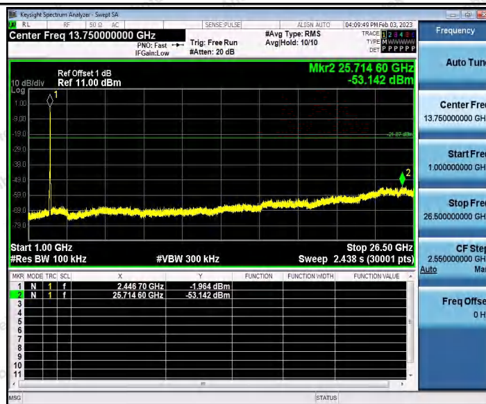
11AX40_Ant2_2452_0~Reference
