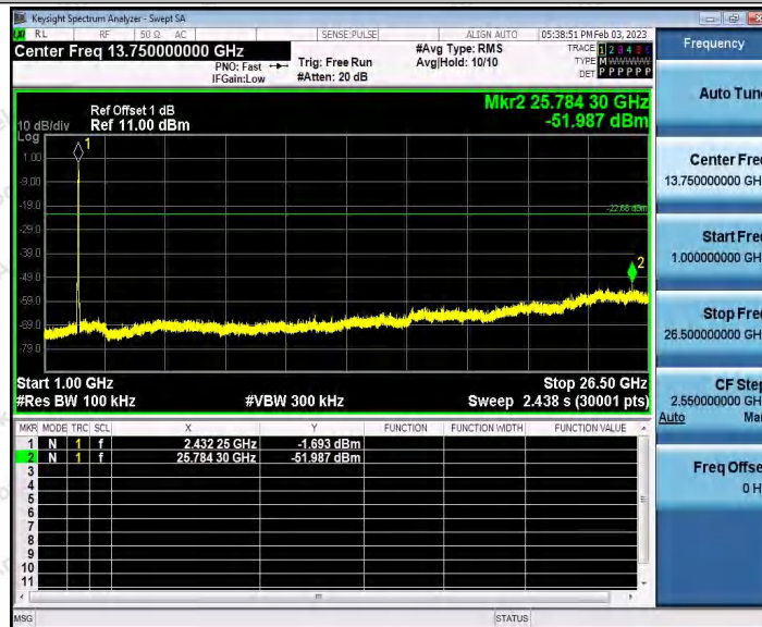
11AX40_Ant1_2452_0~Reference
