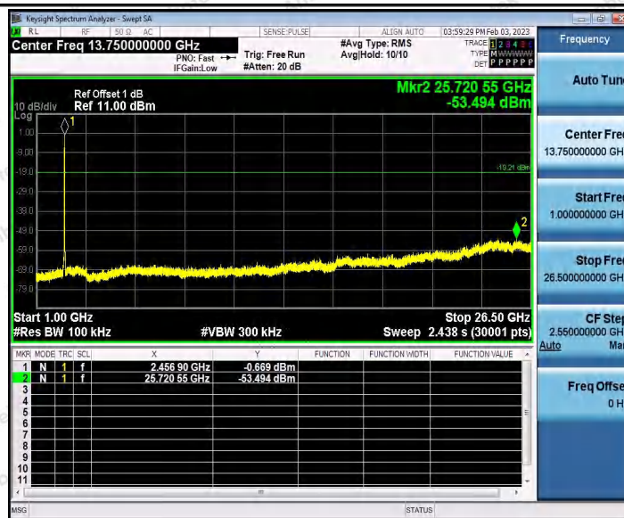
11AX20_Ant2_2462_0~Reference
