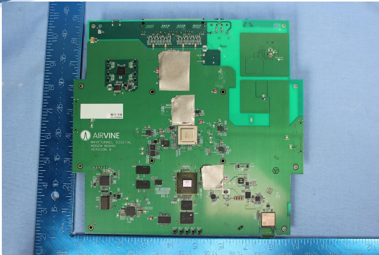
Main Board Bottom
