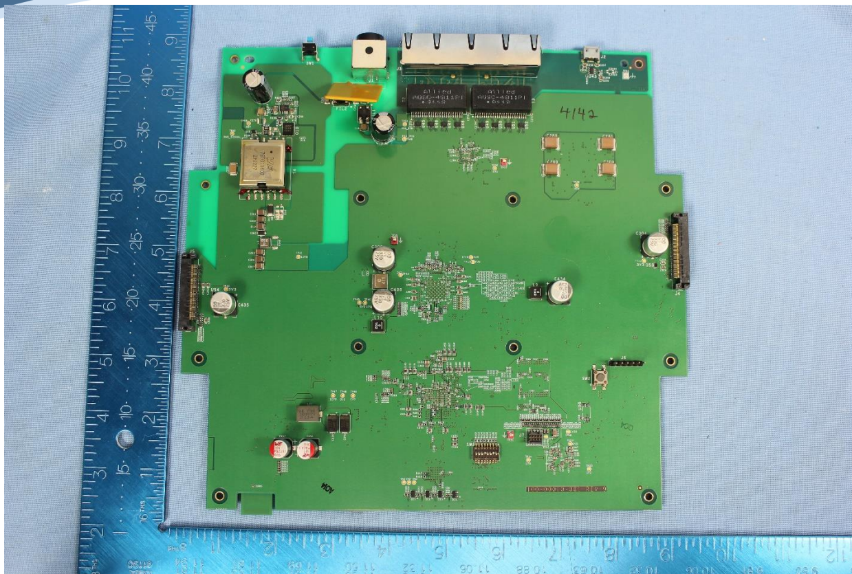
Main Board Top
