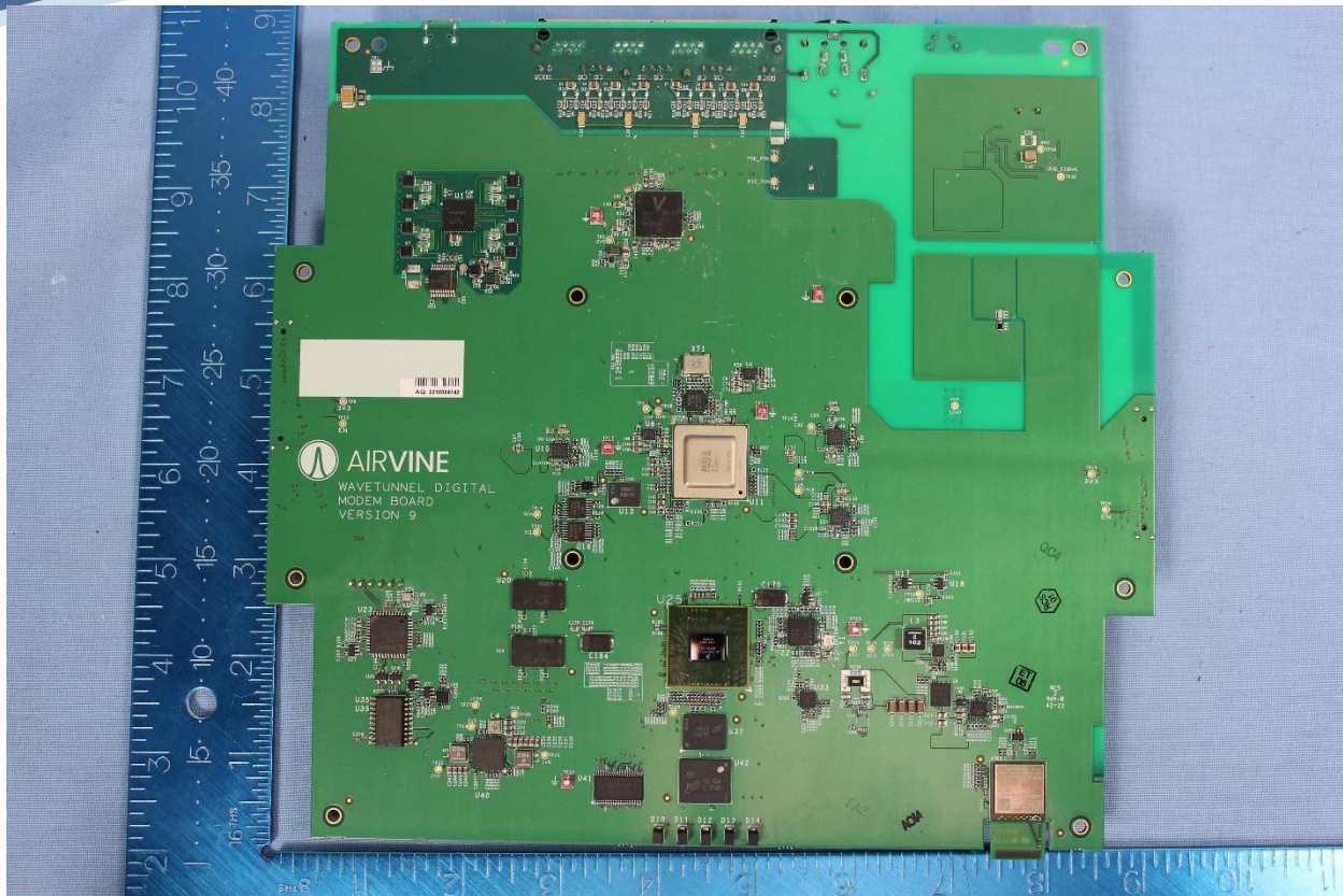
Main Board Bottom Shielding Removed
