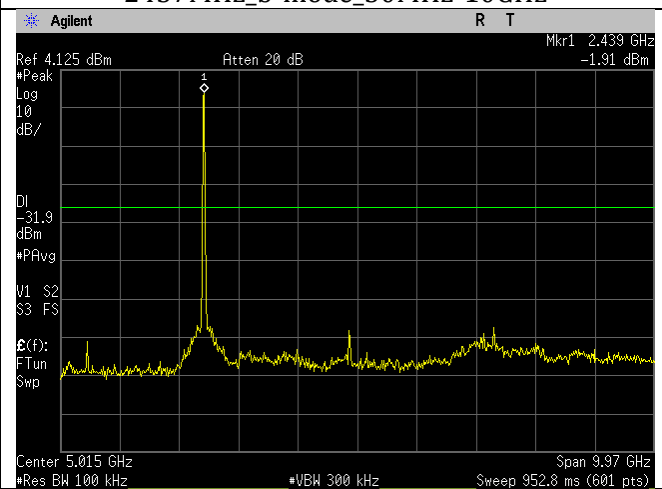
2437MHz_g-mode_30MHz-10GHz
