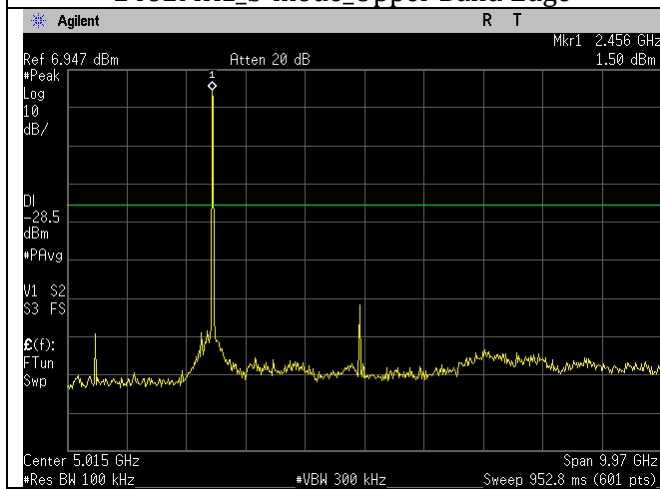
2462MHz_b-mode_30MHz-10GHz
