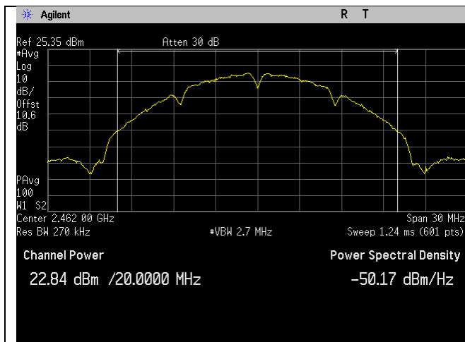
2462MHz_b-mode
