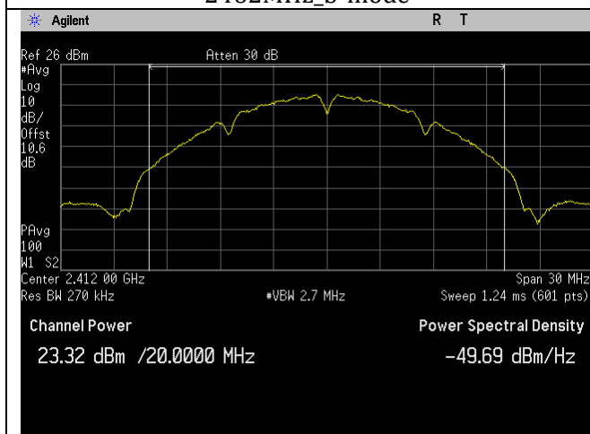
2412MHz_b-mode
