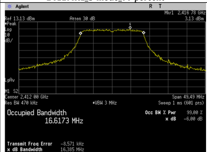
2412MHz_g-mode_99 percent
