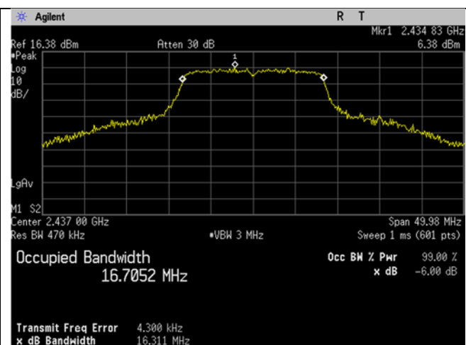
2437MHz_g-mode_99 percent
