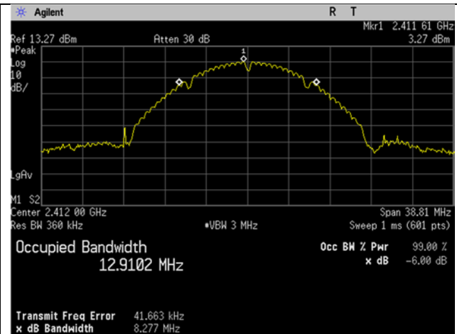
2412MHz_b-mode_99 percent
