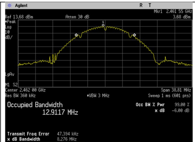
2462MHz_b-mode_99 percent
