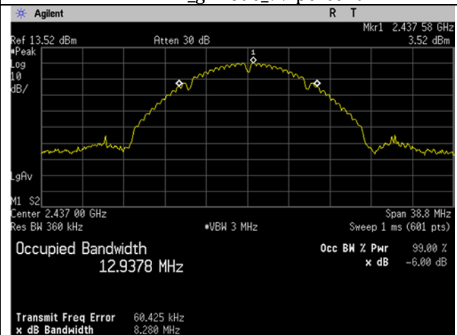
2437MHz_b-mode_99 percent
