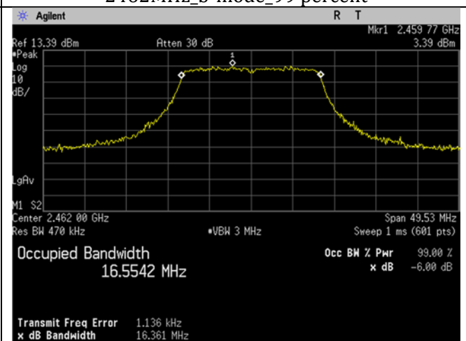
2462MHz_g-mode_99 percent
