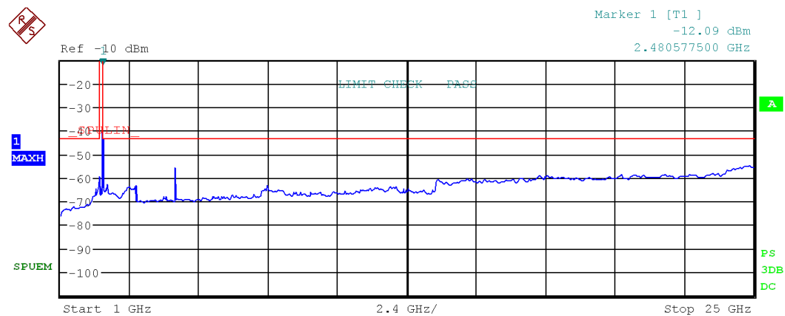
Figure 38: Chart of emissions test from 1 GHz to 25 GHz on highest channel, PK-detector
