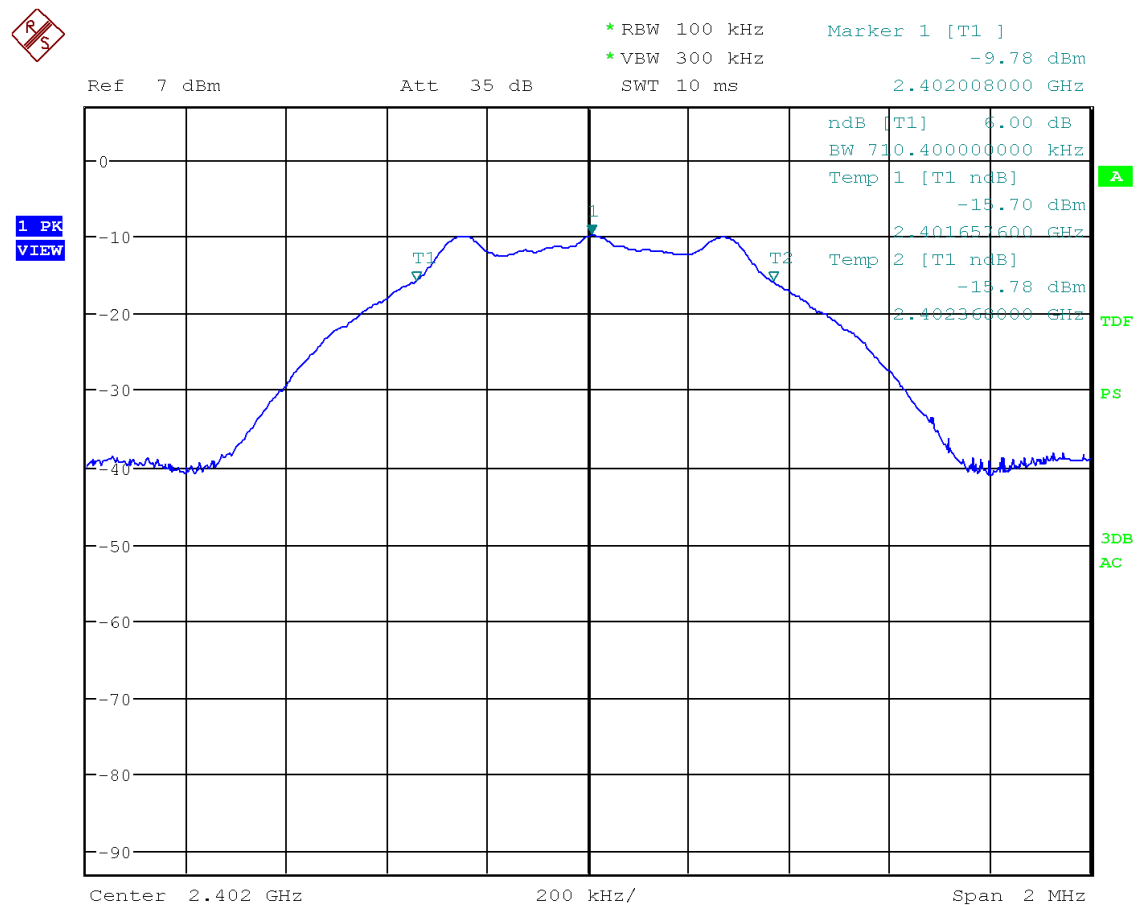
Figure 10: Chart of 6 dB bandwidth test on lowest channel
