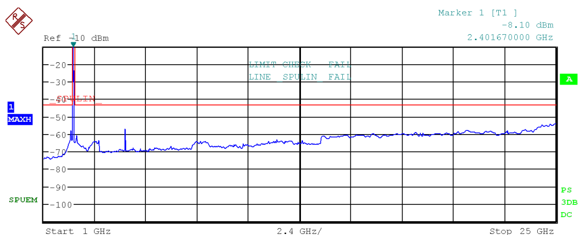
Figure 28: Chart of emissions test from 1 GHz to 25 GHz on lowest channel, PK-detector
