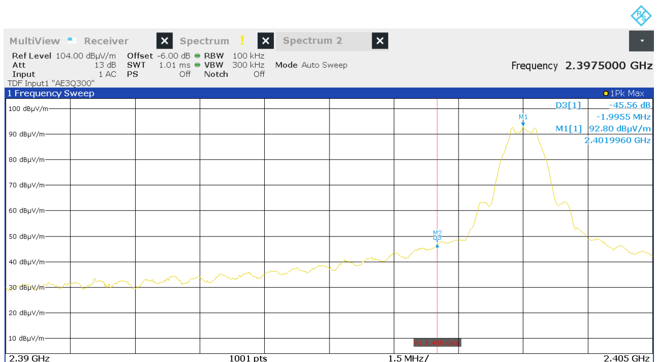
Figure 51: Chart of lower band-edge measurement on lowest channel, EUT position Y, antenna polarization horizontal
