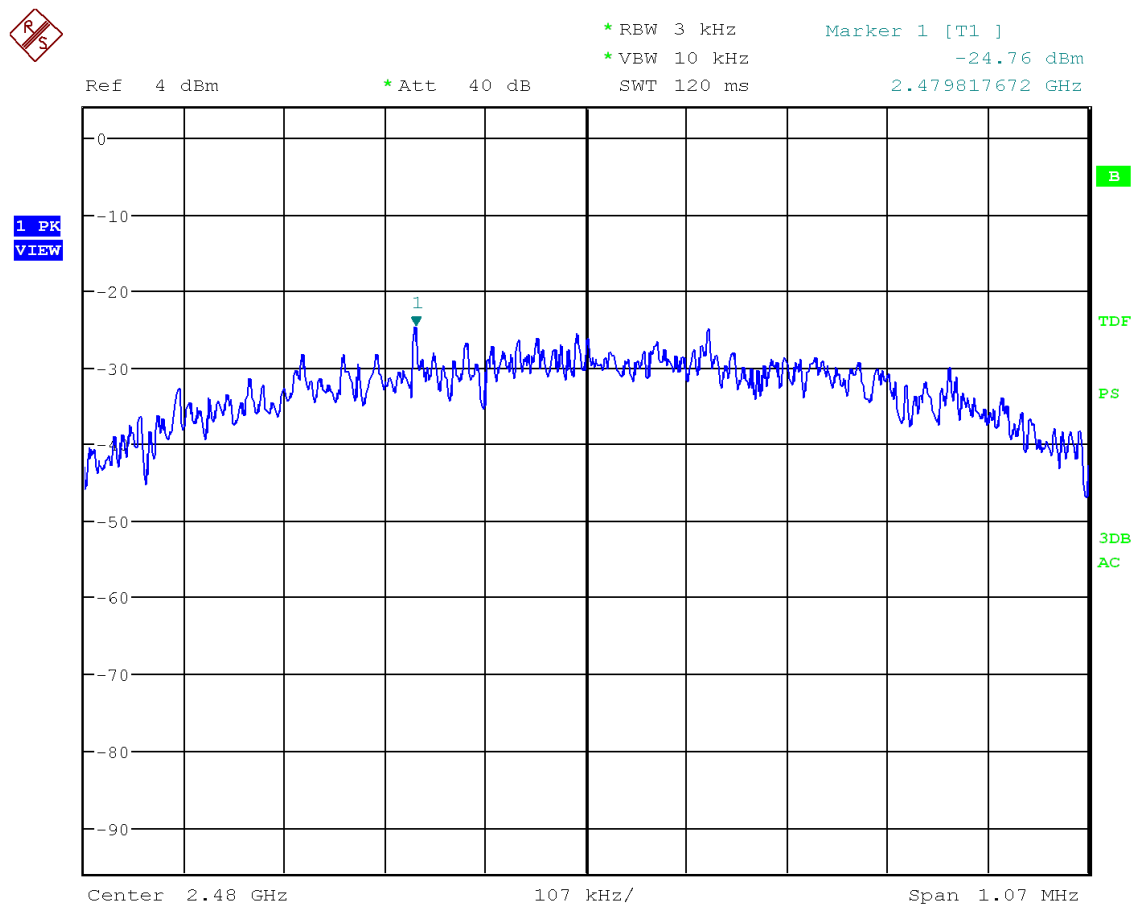
Figure 21: Chart of power spectral density on highest channel
