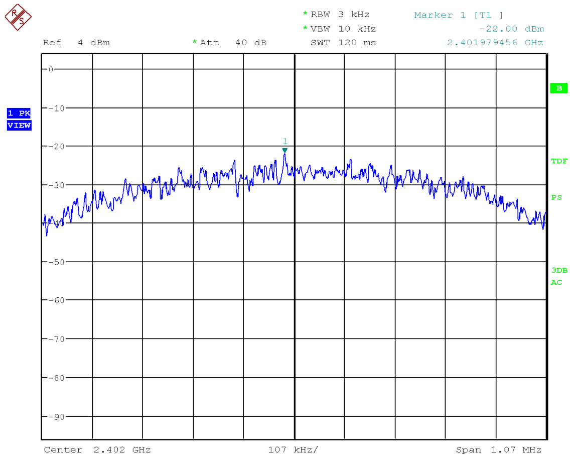
Figure 19: Chart of power spectral density on lowest channel
