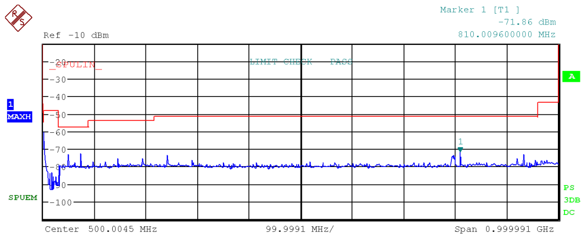
Figure 33: Chart of emissions test from 9 kHz to 1 GHz on lowest channel, PK-detector
