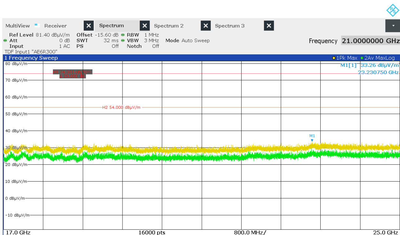
Figure 48: Chart of exploratory emission test from 17 GHz to 25 GHz on highest channel at 0.5 m, EUT position X, antenna polarization vertical and horizontal
