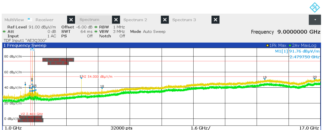
Figure 47: Chart of emissions test from 1 GHz to 17 GHz on highest channel, EUT position Y, antenna polarization horizontal
