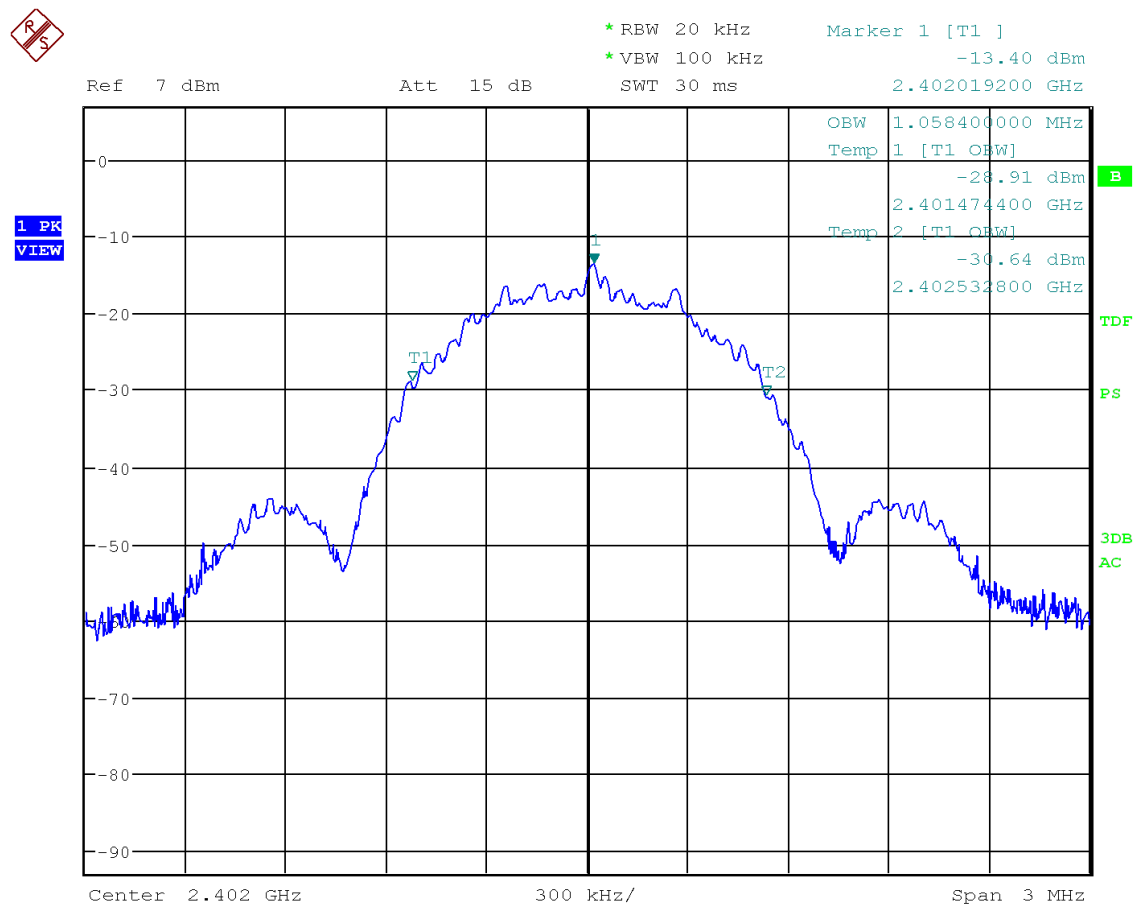
Figure 13: Chart of occupied bandwidth test on lowest channel
