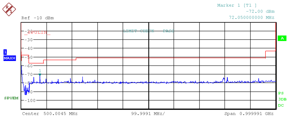
Figure 31: Chart of emissions test from 9 kHz to 1 GHz on highest channel, PK-detector
