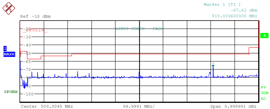
Figure 35: Chart of emissions test from 9 kHz to 1 GHz on middle channel, PK-detector
