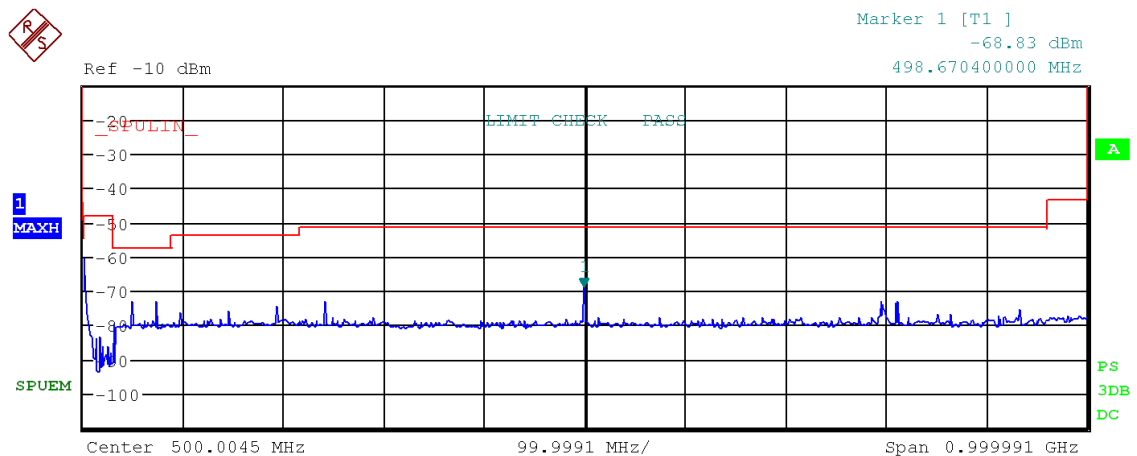
Figure 29: Chart of emissions test from 9 kHz to 1 GHz on middle channel, PK-detector
