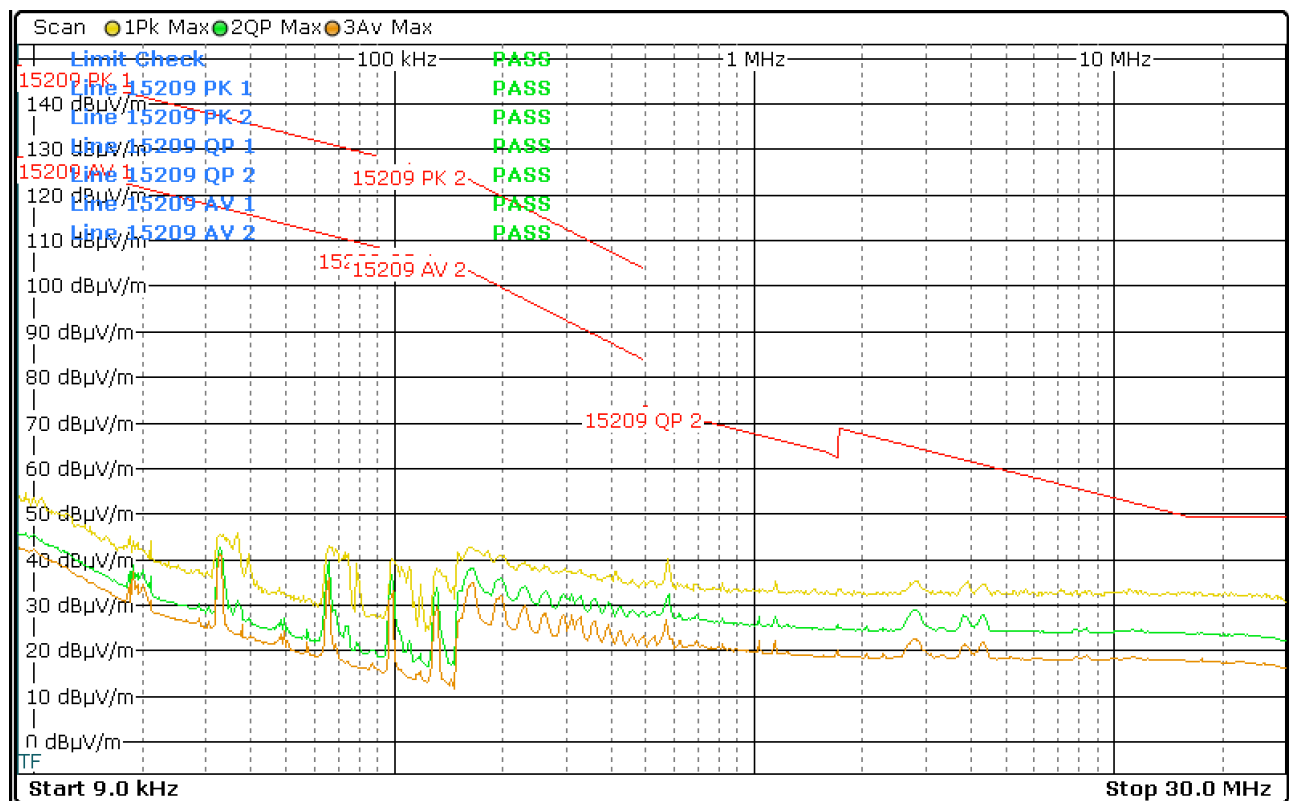
Figure 39: Chart of emissions test below 30 MHz on lowest channel, EUT position X, antenna in line
