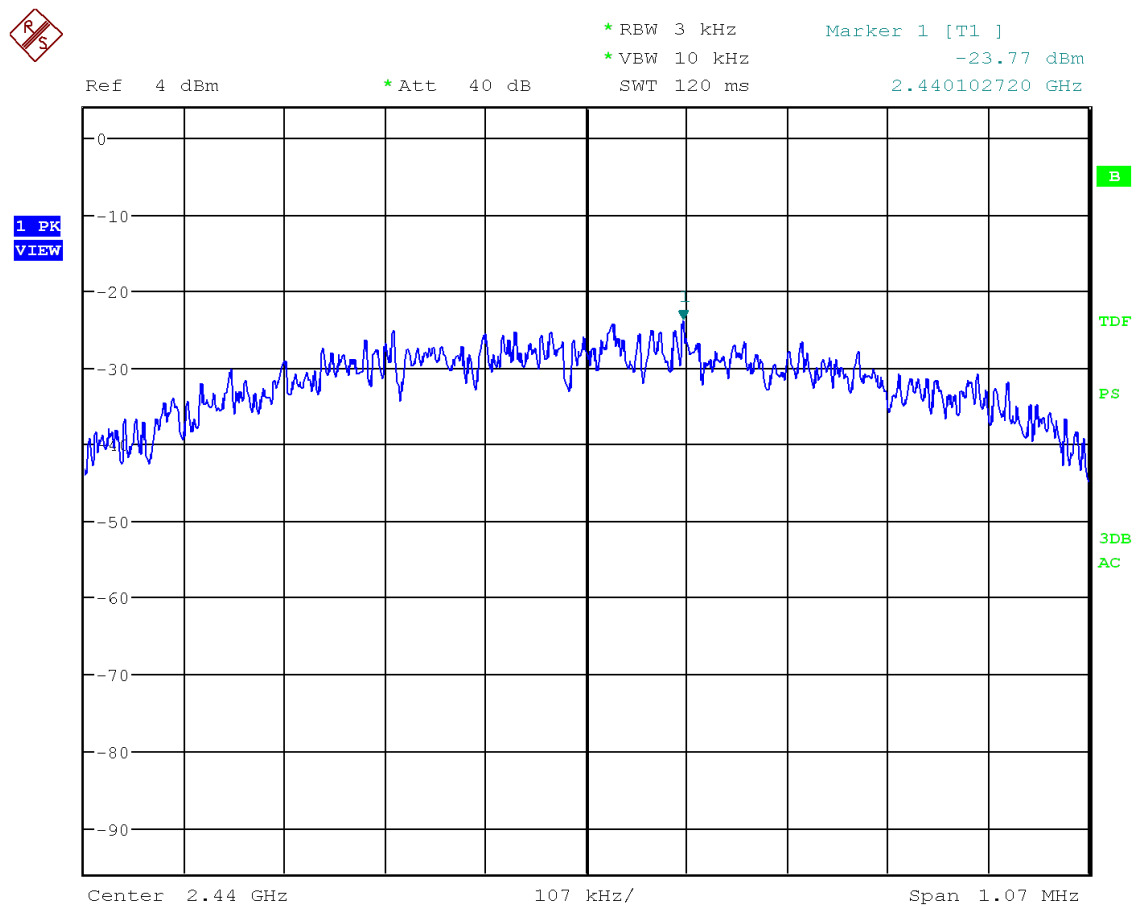
Figure 20: Chart of power spectral density on middle channel
