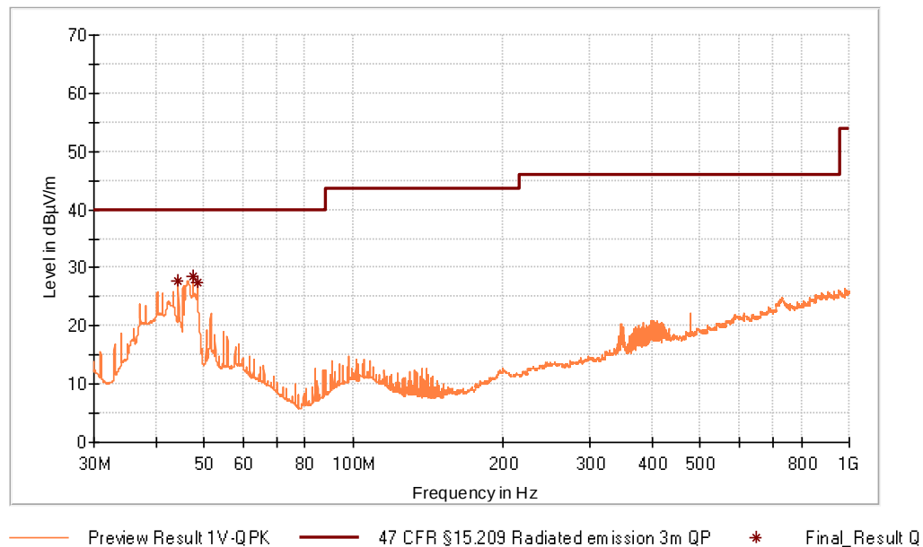
Figure 42: Chart of radiated emissions test from 30 MHz to 1 GHz on lowest channel, EUT position Z, antenna polarization vertical
