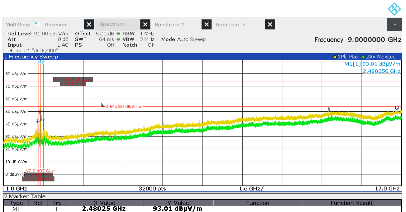
Figure 54: Chart of emissions test from 1 GHz to 17 GHz on highest channel, EUT position Y, antenna polarization horizontal
