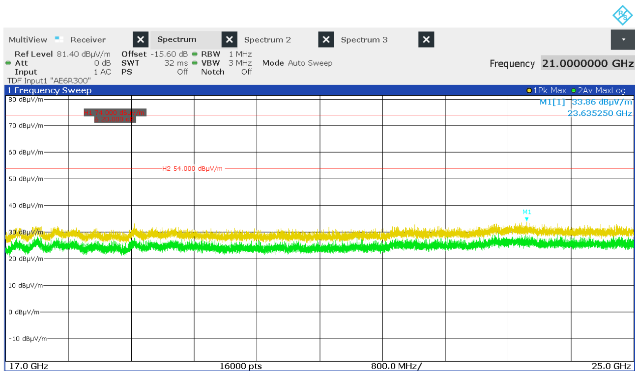
Figure 55: Chart of exploratory emission test from 17 GHz to 25 GHz on highest channel at 0.5 m, EUT position X, antenna polarization vertical and horizontal
