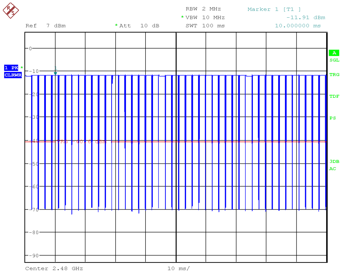
Figure 25: Chart of duty cycle measurement on highest channel_sweep time 100 ms
