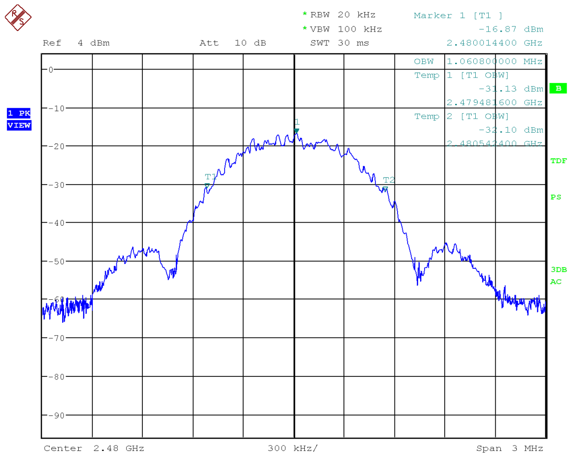
Figure 15: Chart of occupied bandwidth test on highest channel
