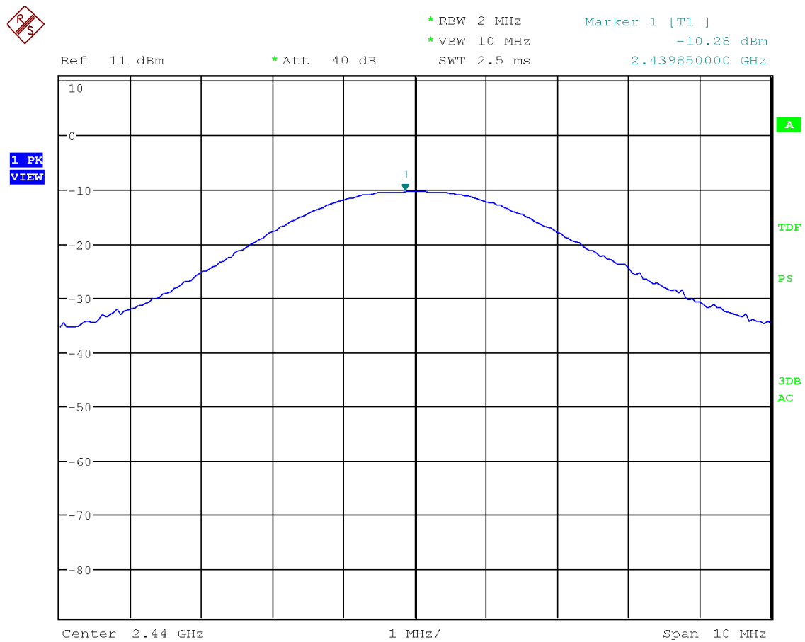
Figure 17: Chart of conducted output power on middle channel
