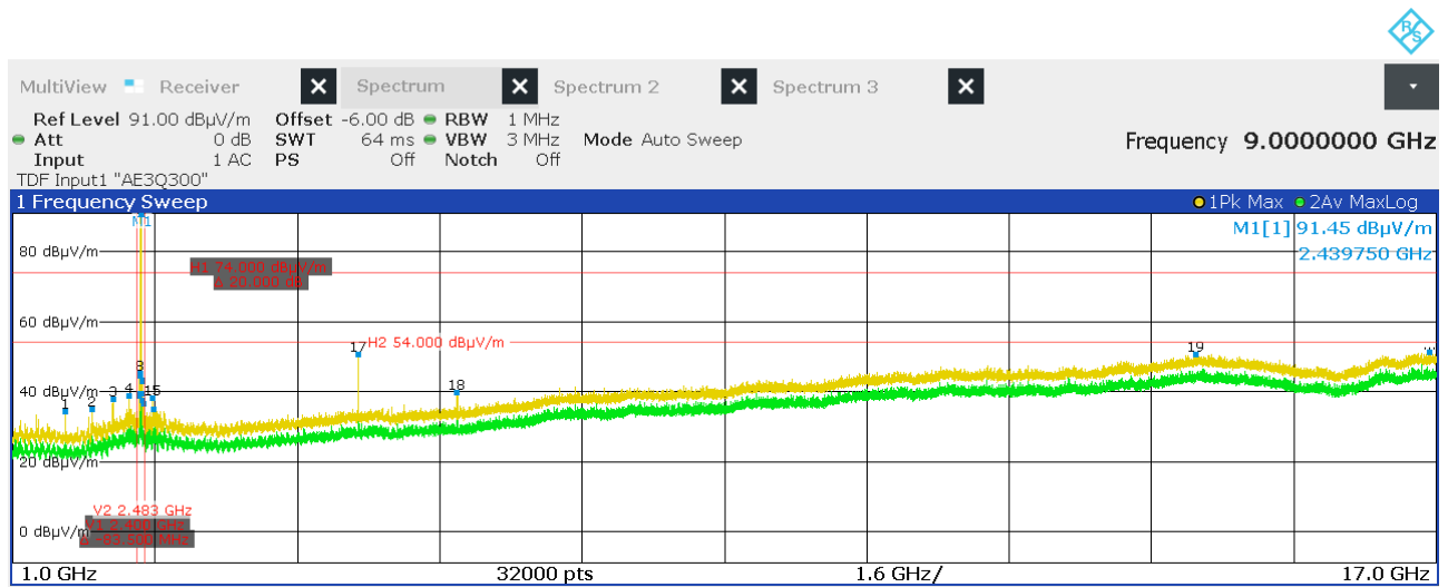
Figure 45: Chart of radiated emissions pre-measurement from 1 GHz to 17 GHz on middle channel, EUT position Y, antenna polarization horizontal
