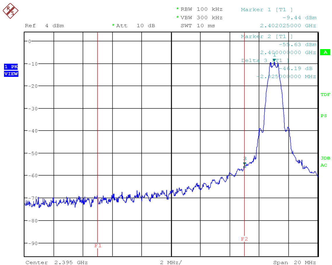
Figure 22: Chart of lower band-edge measurement on lowest channel
