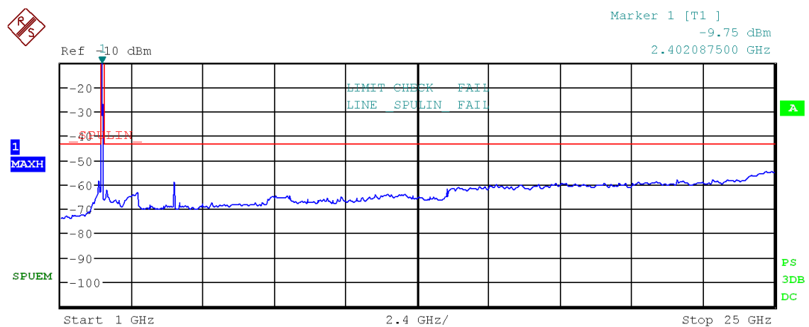
Figure 34: Chart of emissions test from 1 GHz to 25 GHz on lowest channel, PK-detector
