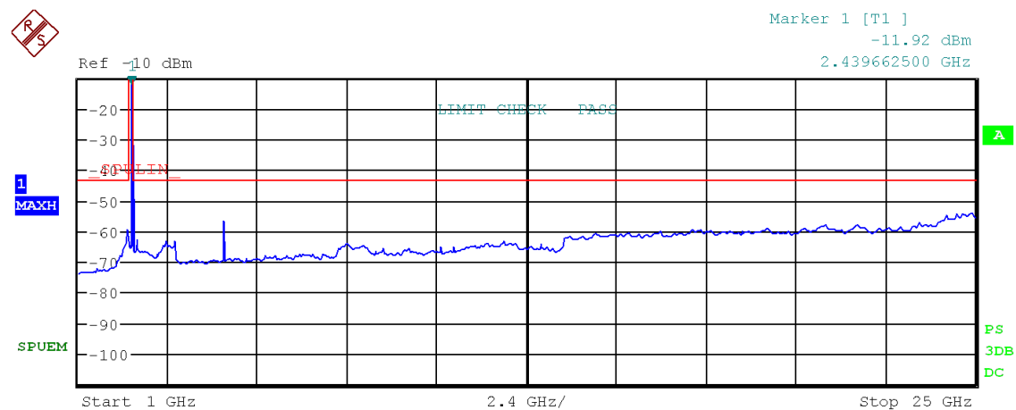
Figure 30: Chart of emissions test from 1 GHz to 25 GHz on middle channel, PK-detector
