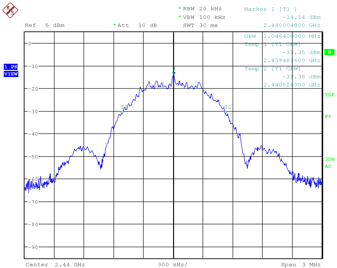
Figure 14: Chart of occupied bandwidth test on middle channel
