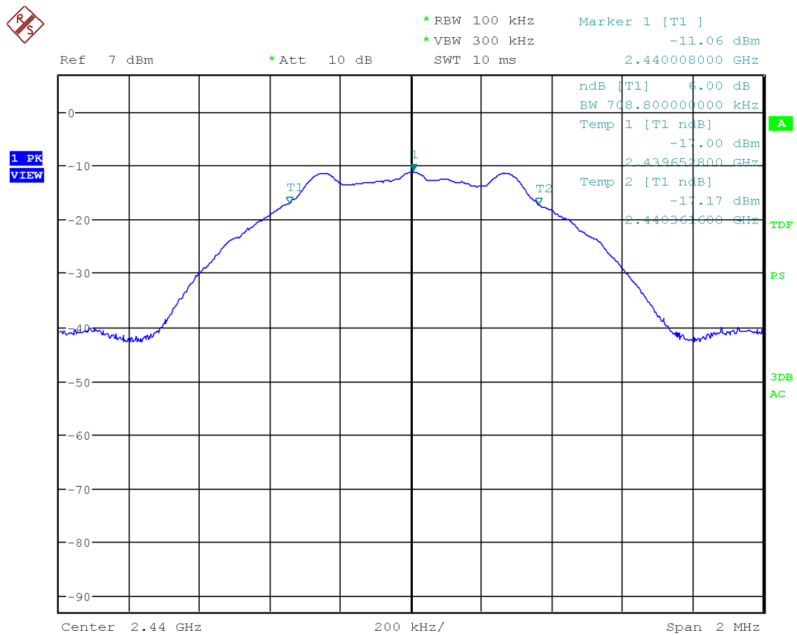
Figure 11: Chart of 6 dB bandwidth test on middle channel
