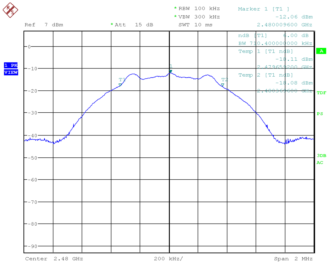
Figure 12: Chart of 6 dB bandwidth test on highest channel
