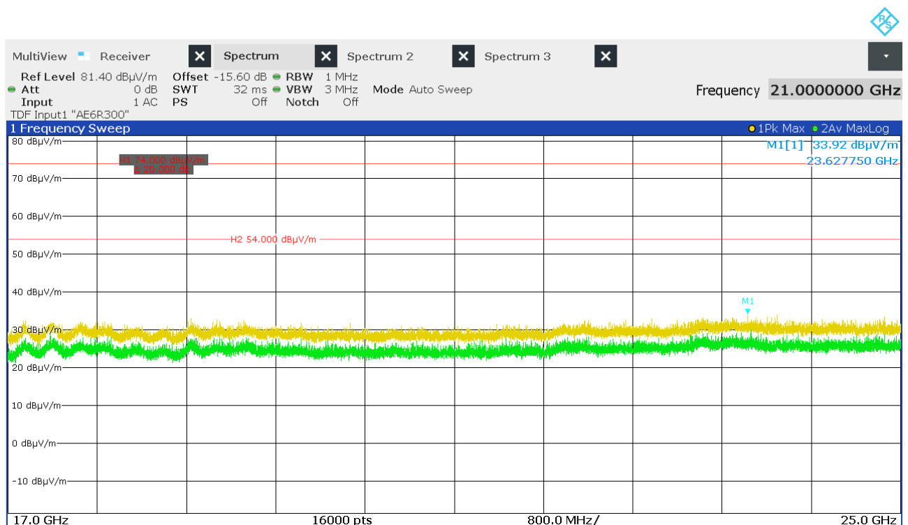
Figure 53: Chart of exploratory emissions measurement from 17 GHz to 25 GHz on middle channel, EUT position X, antenna polarization vertical and horizontal
