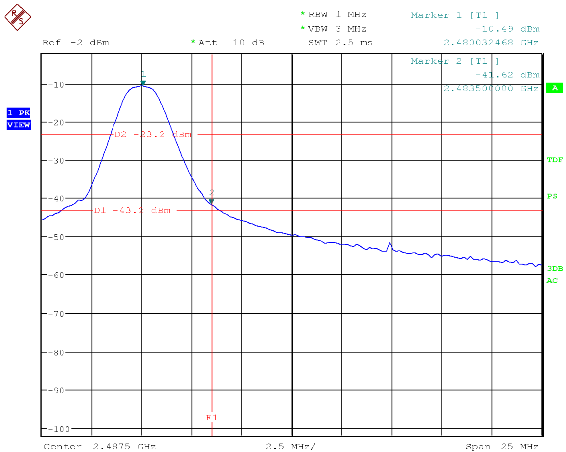
Figure 23: Chart of upper band-edge measurement on highest channel (PK)
