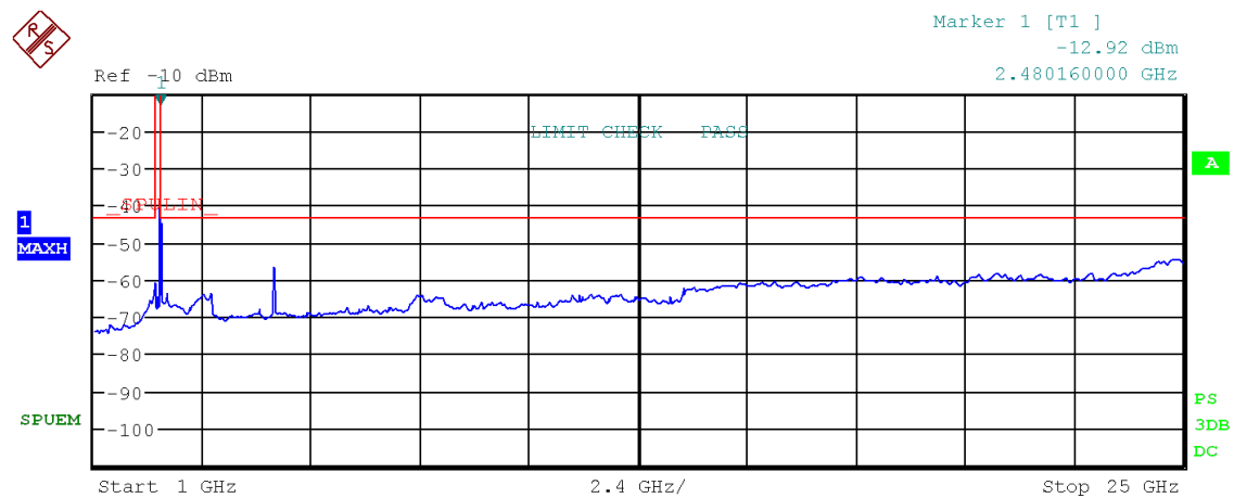
Figure 32: Chart of emissions test from 1 GHz to 25 GHz on highest channel, PK-detector
