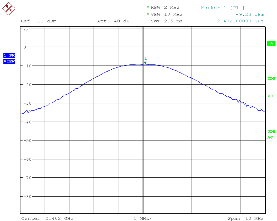
Figure 16: Chart of conducted output power on lowest channel
