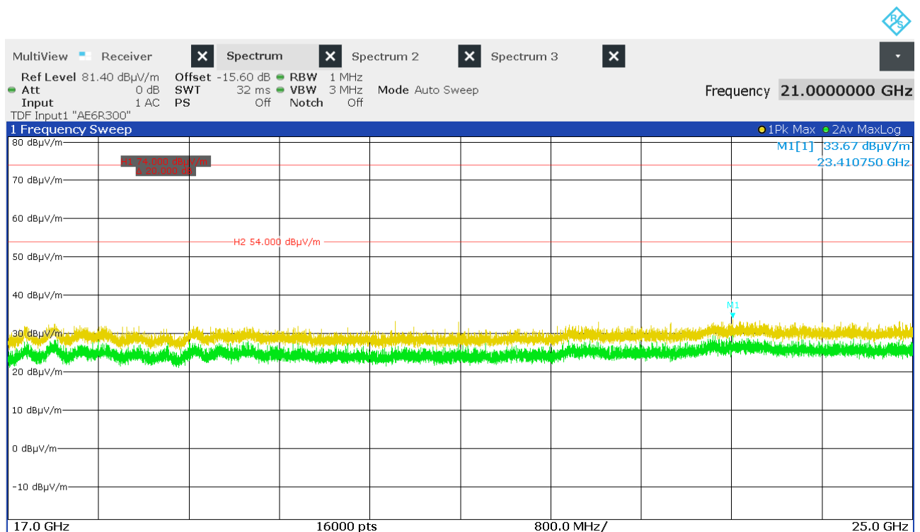
Figure 50: Chart of exploratory radiated emissions measurement from 17 GHz to 25 GHz on lowest channel, EUT position X, antenna polarization vertical and horizontal
