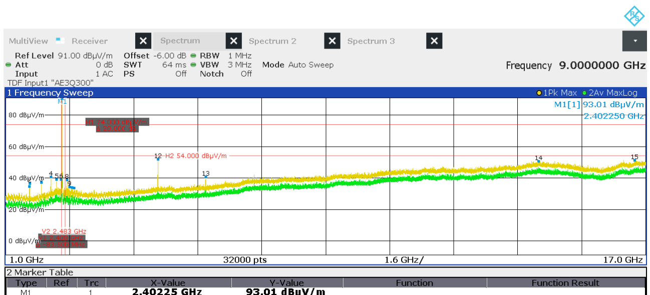
Figure 43: Chart of radiated emissions pre-measurement from 1 GHz to 17 GHz on lowest channel, EUT position Y, antenna polarization horizontal
