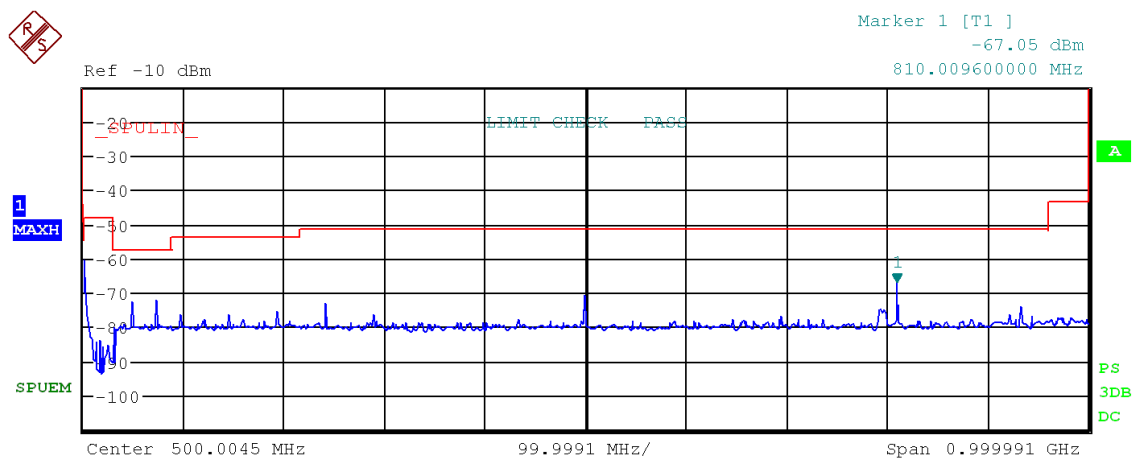
Figure 37: Chart of emissions test from 9 kHz to 1 GHz on highest channel, PK-detector
