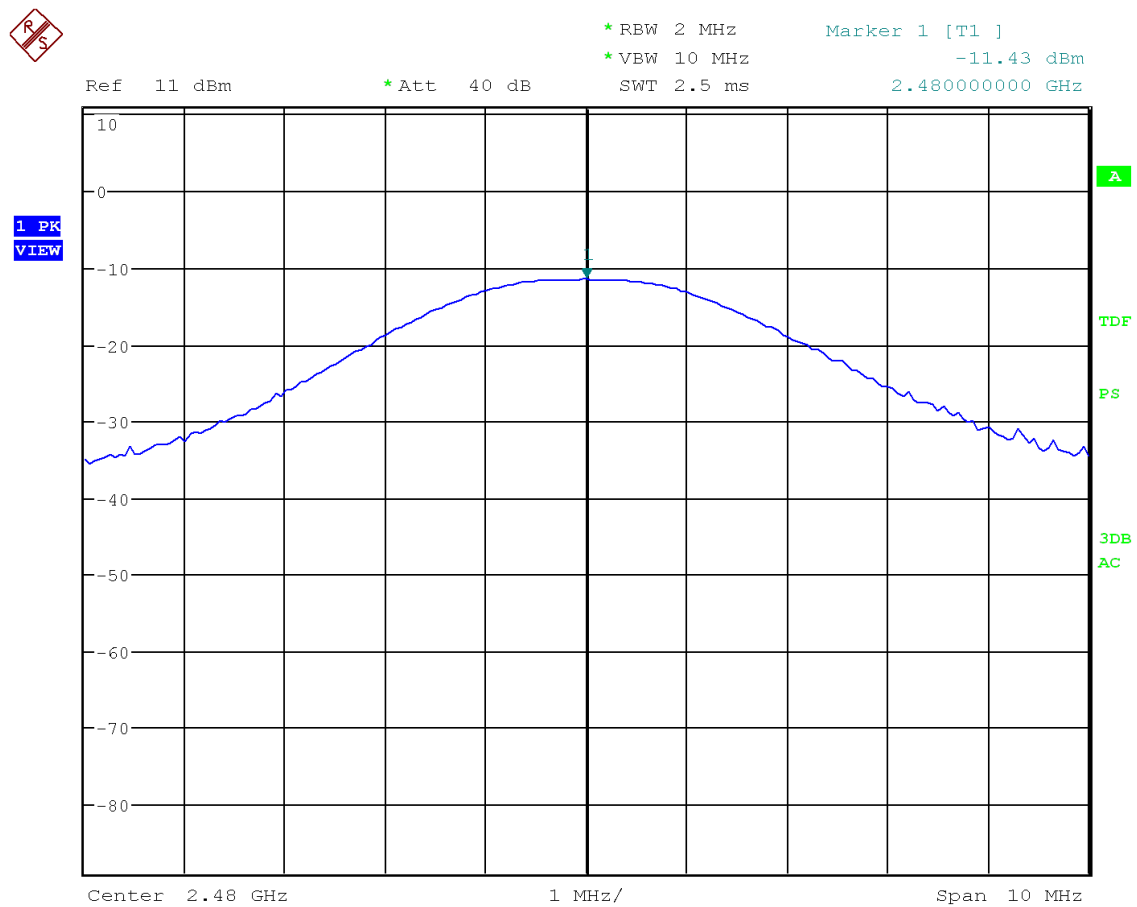
Figure 18: Chart of conducted output power on highest channel
