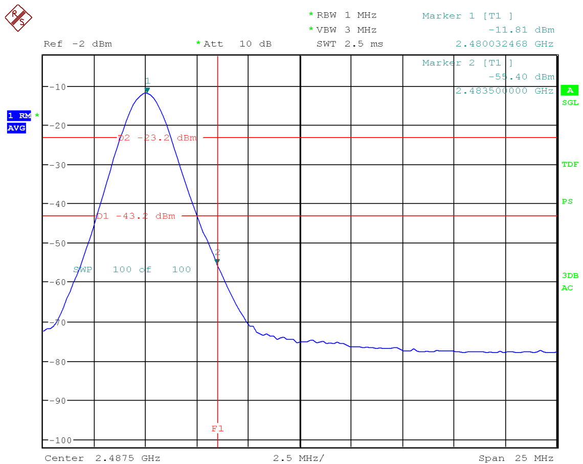
Figure 24: Chart of upper band-edge measurement on highest channel (RMS)
