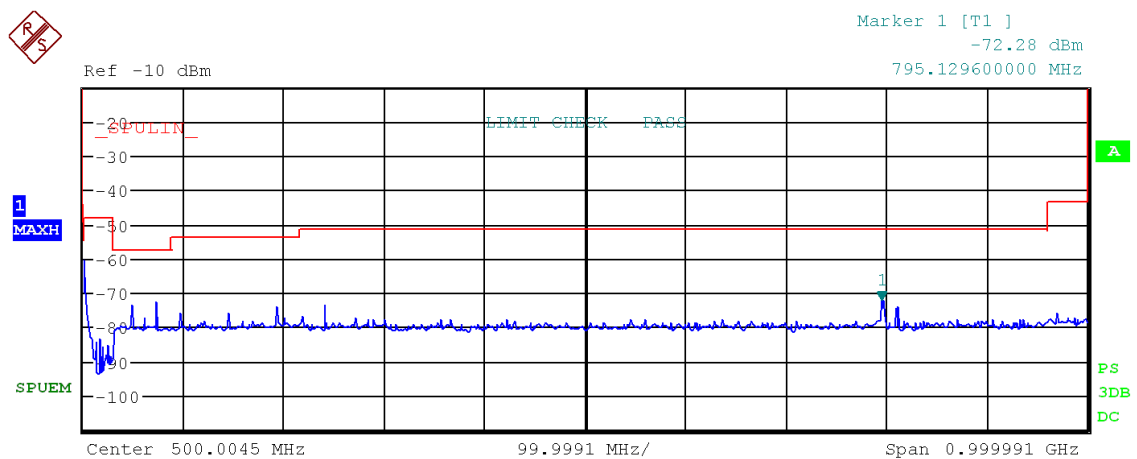
Figure 27: Chart of emissions test from 9 kHz to 1 GHz on lowest channel, PK-detector
