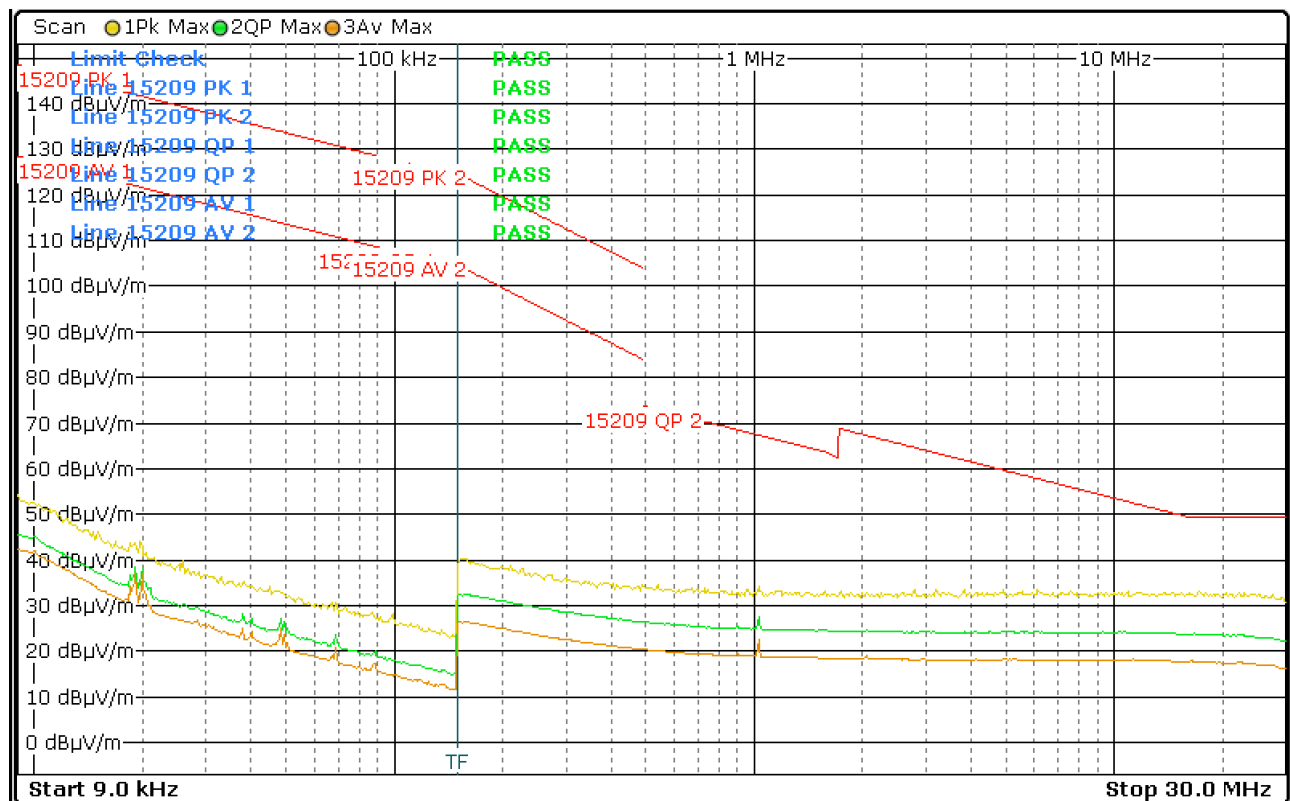
Figure 40: Chart of emissions test below 30 MHz on lowest channel, EUT position Y, antenna in line
