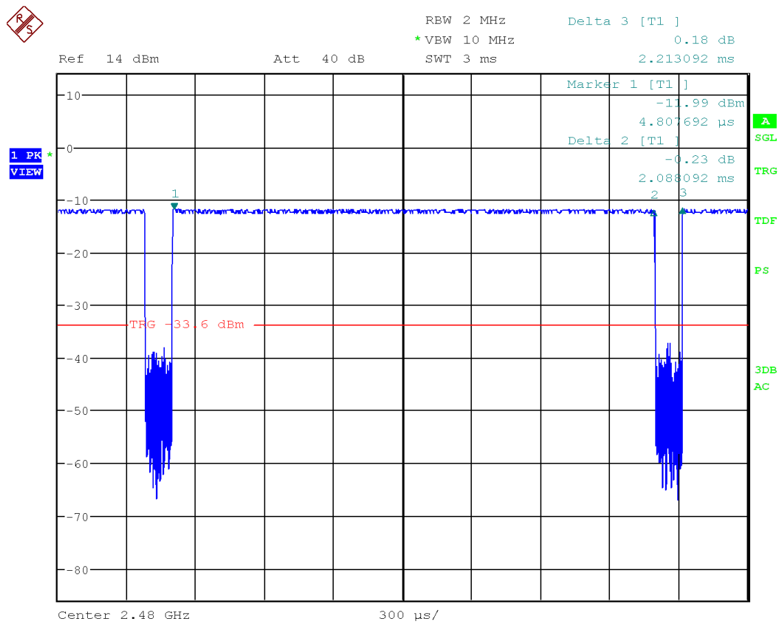
Figure 26: Chart of duty cycle measurement on highest channel_sweep time 3 ms
