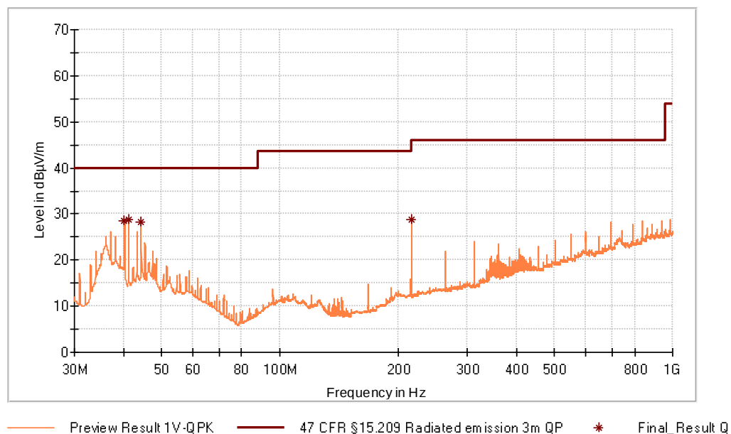
Figure 41: Chart of radiated emissions test from 30 MHz to 1 GHz on lowest channel, EUT position X, antenna polarization vertical
