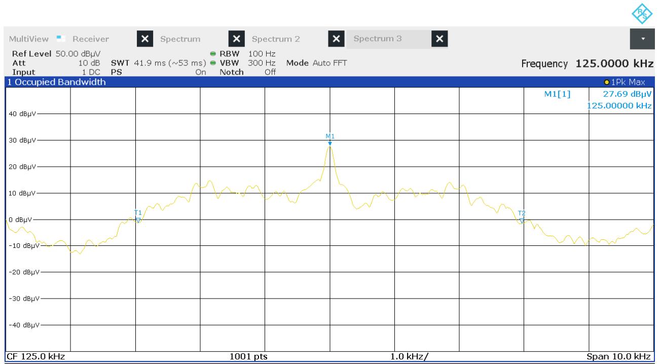
Figure 9: Chart of occupied bandwidth test, with tag
