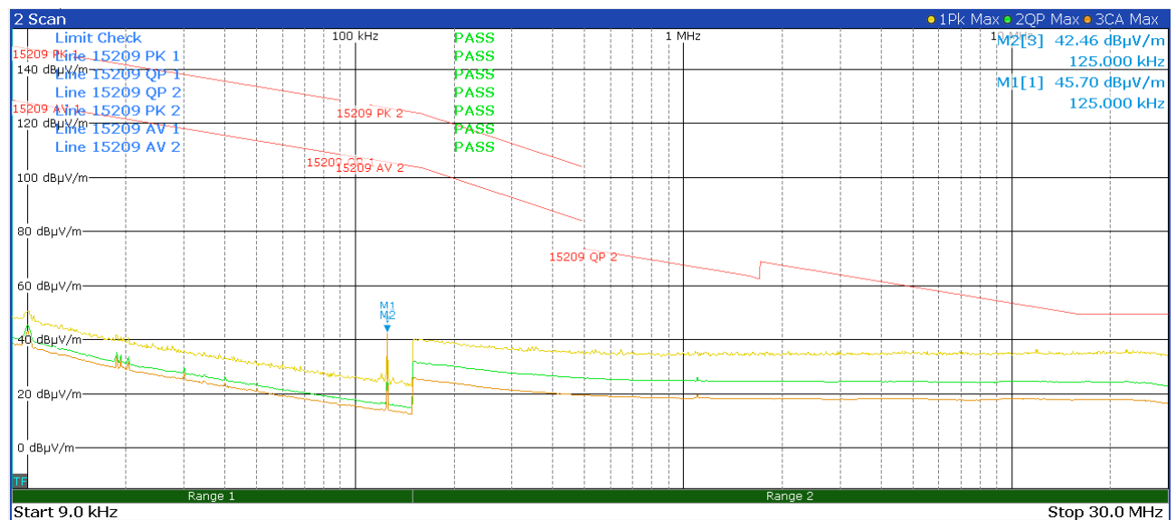
Figure 12: Chart of radiated emissions test below 30 MHz, EUT position Y, without tag, antenna in line
