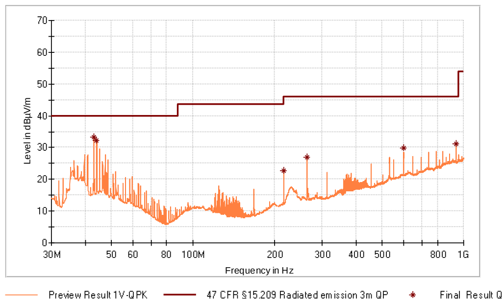
Figure 13: Chart of radiated emissions test from 30 MHz to 1 GHz, EUT position X, without tag, antenna vertical
