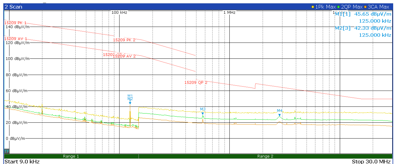
Figure 11: Chart of radiated emissions test below 30 MHz, EUT position Y, without tag, antenna in line
