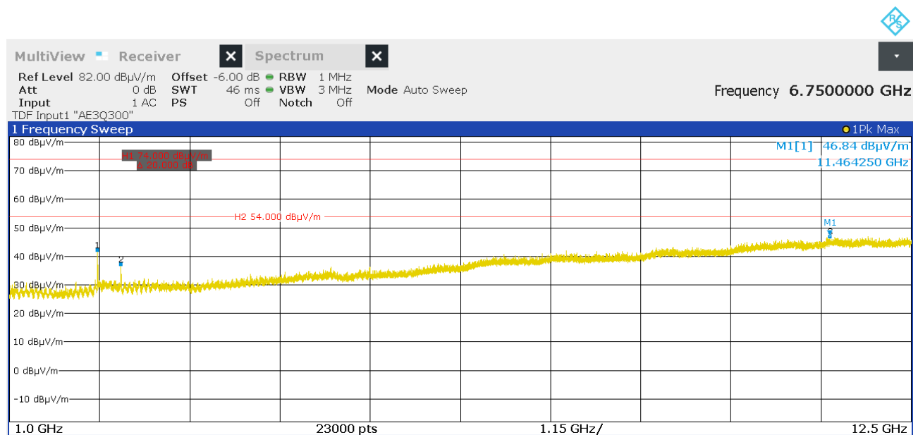
Figure 15: Chart of radiated emissions pre-measurement from 1 GHz to 12.5 GHz, EUT position Z, with tag, antenna polarization horizontal
