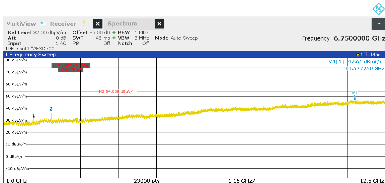
Figure 16: Chart of radiated emissions pre-measurement from 1 GHz to 12.5 GHz, EUT position Y, with tag, antenna polarization horizontal
