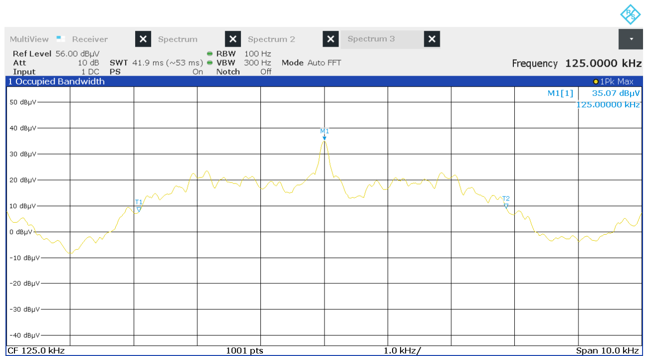
Figure 10: Chart of occupied bandwidth test, with tag
