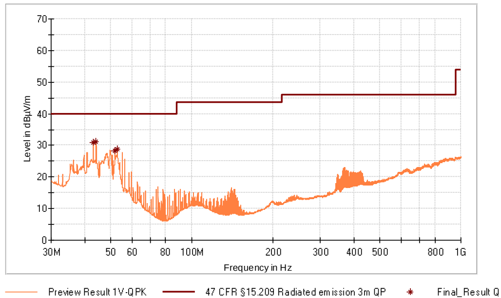
Figure 14: Chart of radiated emissions test from 30 MHz to 1 GHz, EUT position Y, with tag, antenna vertical
