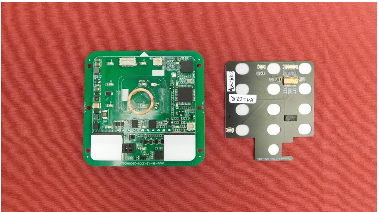
Picture 4: EUT - PCB front view with unmounted keyboard
