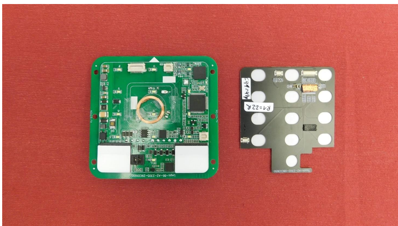
Picture 4: EUT - PCB front view with unmounted keyboard
